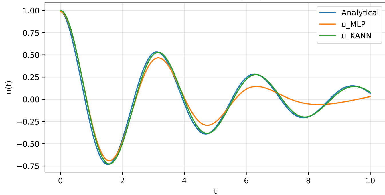
1D Oscillating Spring
