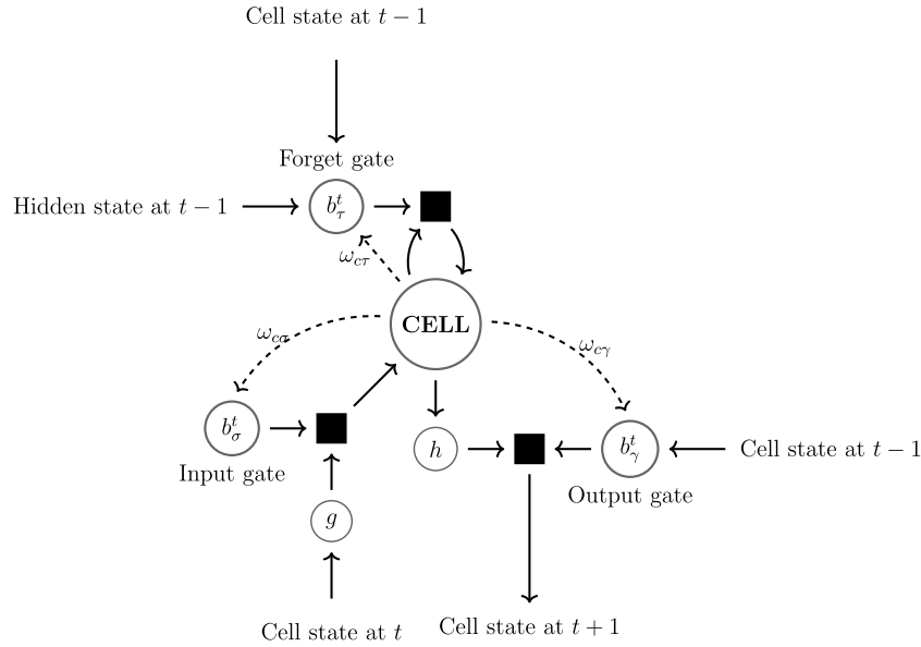
Fig. 1. LSTM memory block. The input, output and forget gates that controls the activation of the cell through the multiplicative units (black squares) from inside and outside. Note that the forget gates will multiply the previous state of the cell. Functions g and h are activation functions explained in the text.
