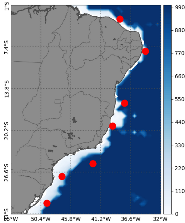
Fig. 2. Region of analysis in the Brazilian coast with bathymetry. Red circles indicates the location of the seven buoys studied in this work. The blue colour scale represents the bathymetry.
