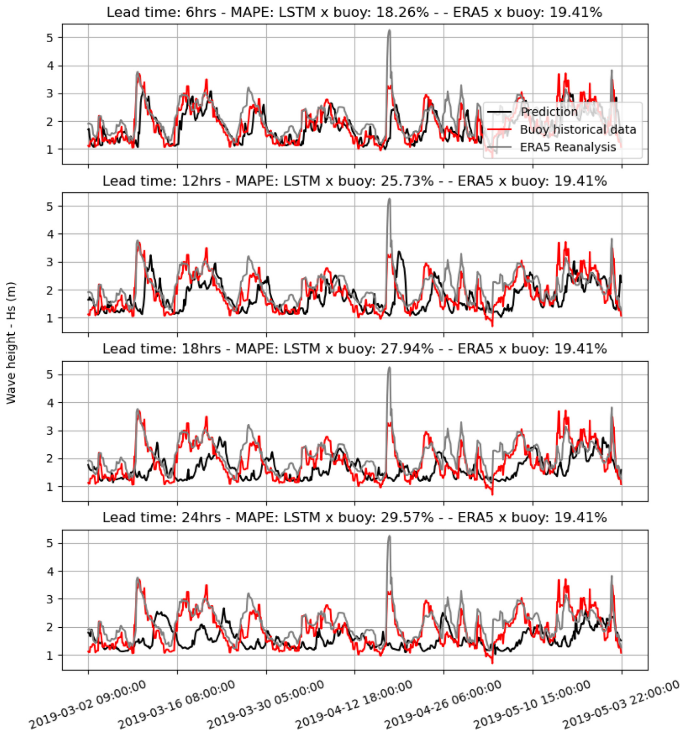
Fig. 15. Prediction of H_s using LSTM for buoy location number two using measured data as feature. Predictions are in black and buoy data given in red.
