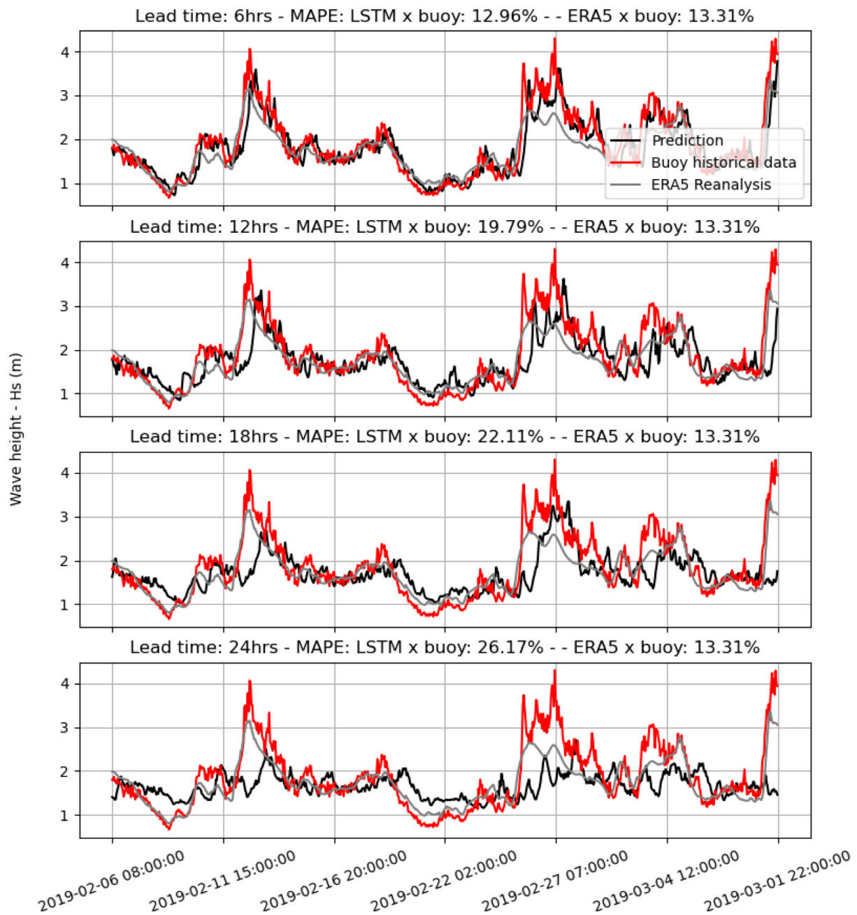
Fig. 14. Prediction of H_s using LSTM for buoy location number one using measured data as feature. Predictions are in black and buoy data given in red.
