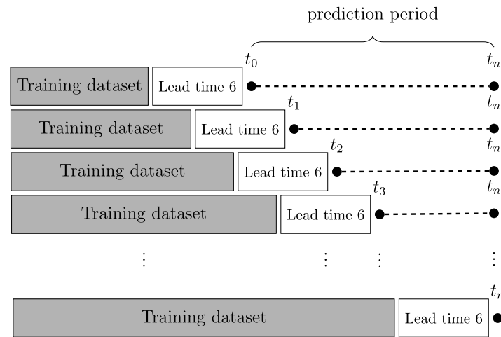
Fig. 4. Schematic of the methodology for training applied in this work, for lead time six (other lead times follow analogously). For each verification time t_i , where i = 1, \dots, n , the training set consists of data until six hours steps prior to t_i .
