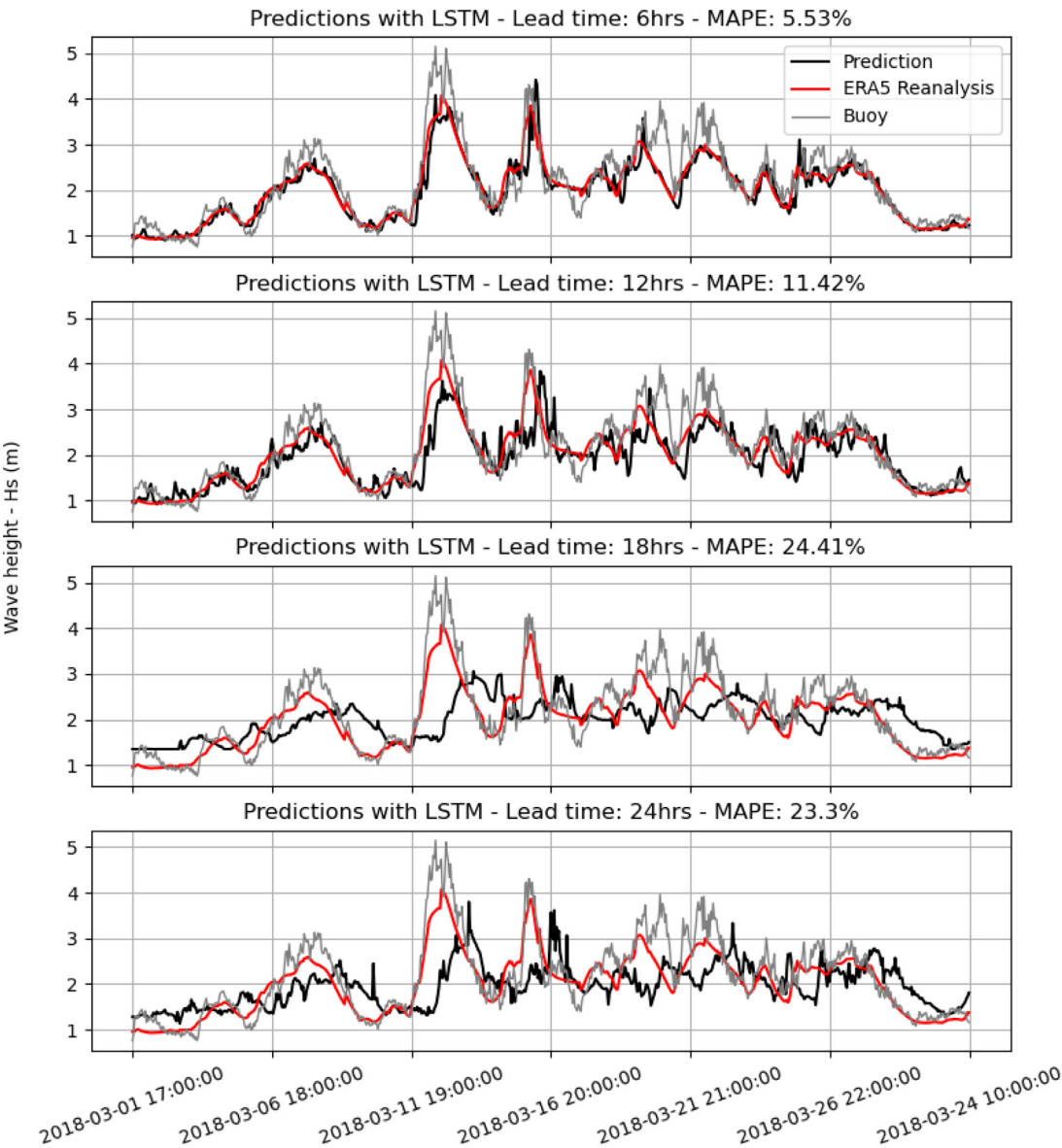
Fig. 12. Multi-variable prediction for buoy location number one using LSTM for the best correlated variables. Predictions are in black, reanalysis from ERA5 in red and buoy data given in grey.
