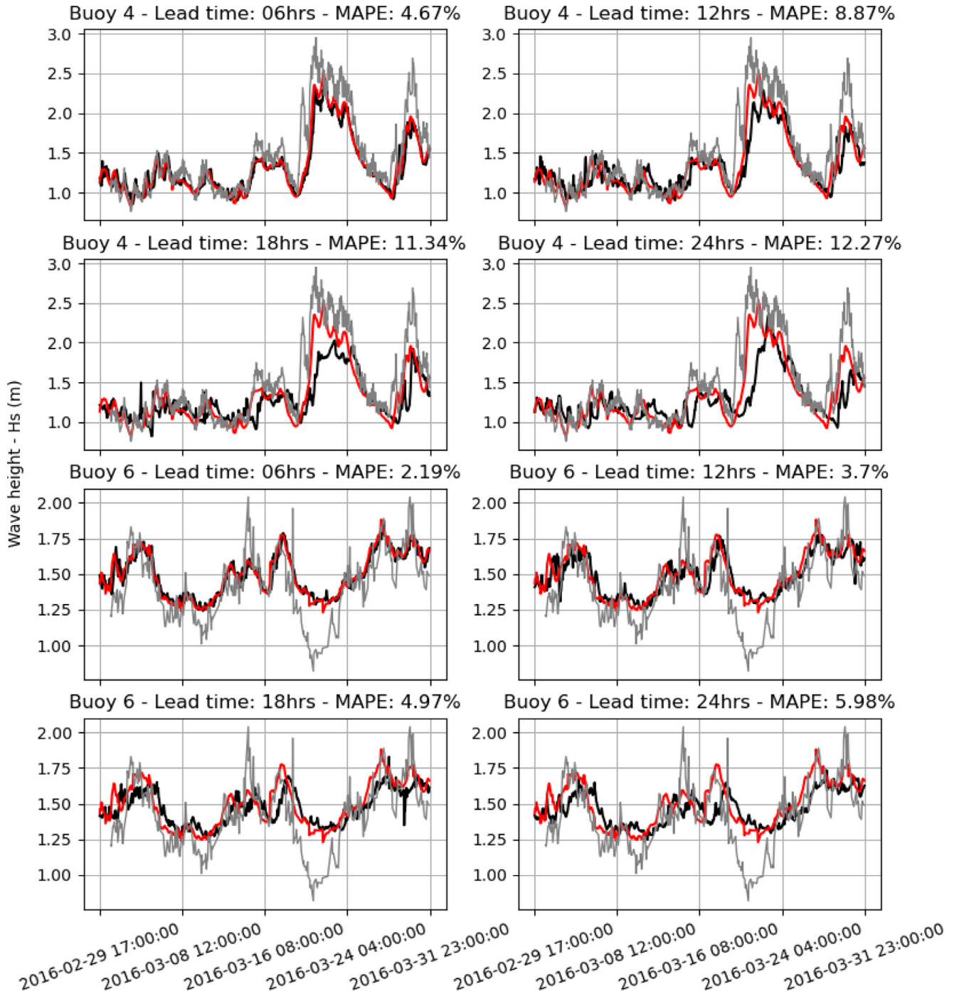
Fig. 9. Predictions (black) and reanalysis from ERA5 (red) comparison for buoys locations number four and six. The grey dashed line show real observations obtained from the buoy.
