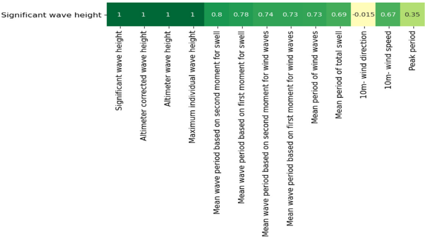
Fig. 11. Pearson’s correlation coefficient between the best 12 ERA5 ocean wave variables and H_s .
