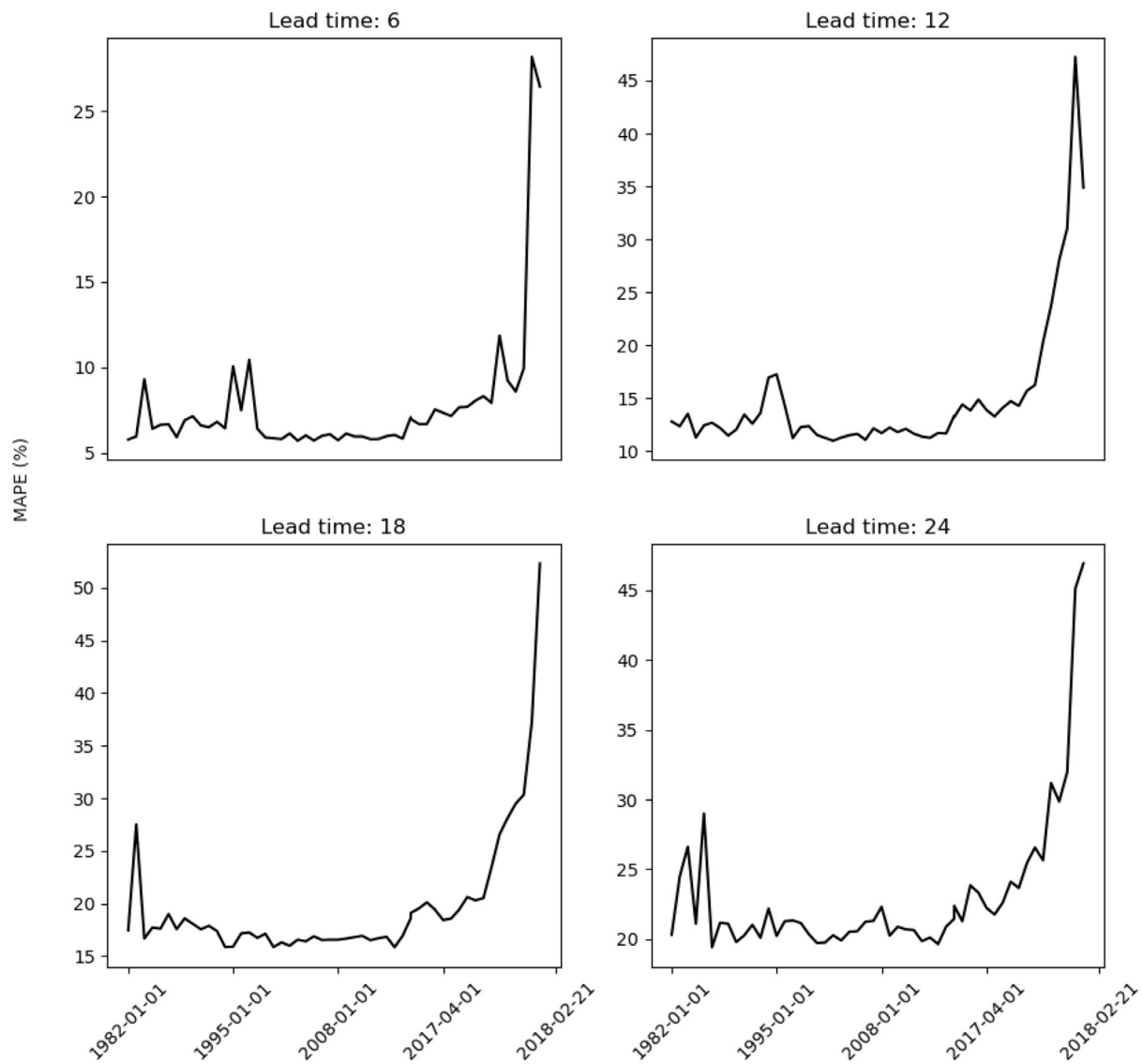
Fig. 3. MAPE calculated for LSTM predictions using different starting dates: from January/1979 until February/2018. Simulations were performed for buoy number 1 location and ERA5 as training dataset.
