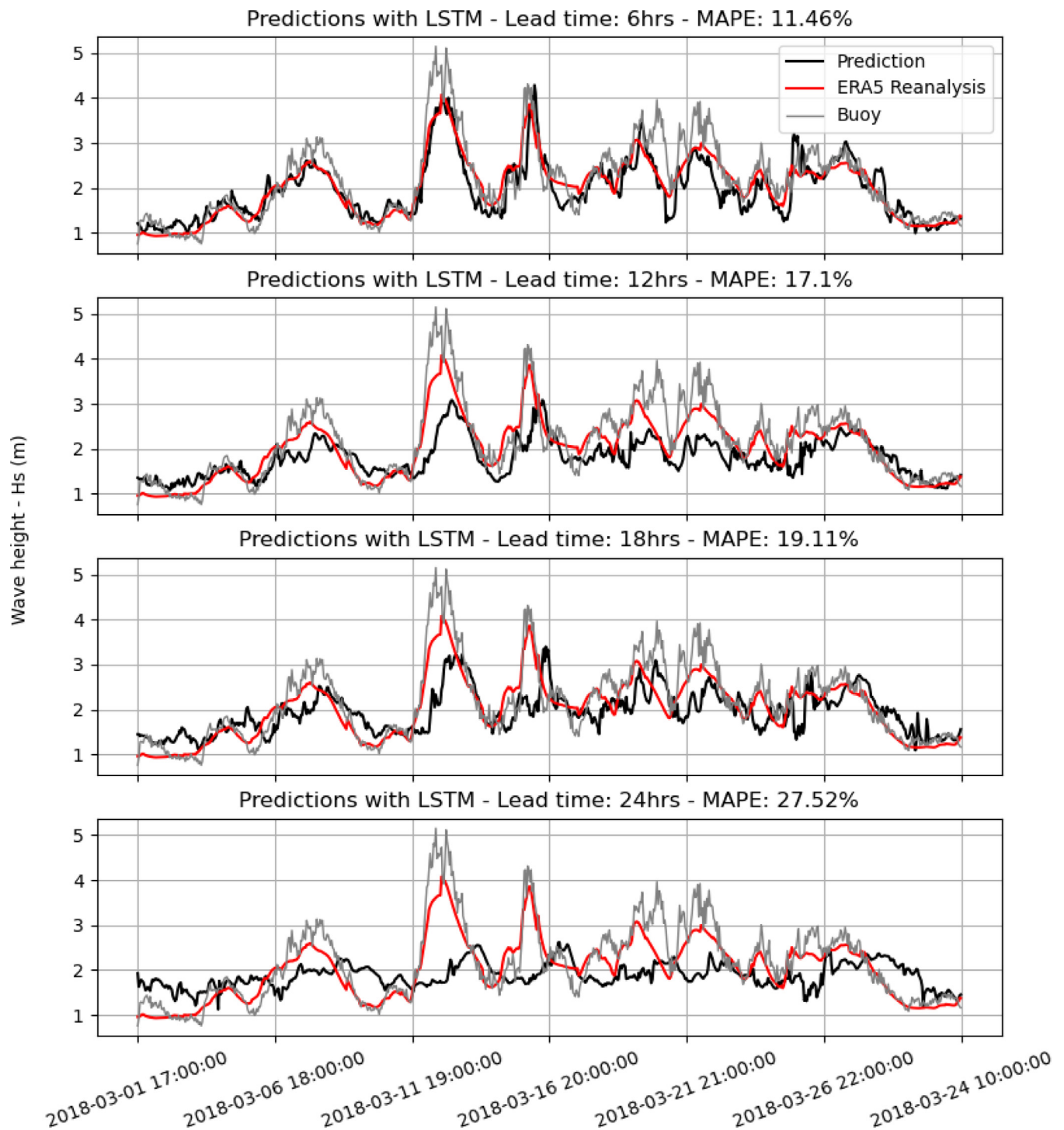
Fig. 13. Prediction using LSTM for buoy location number one considering only T_p and U_{10} as the inputs. Predictions are in black, reanalysis from ERA5 in red and buoy data given in grey.
