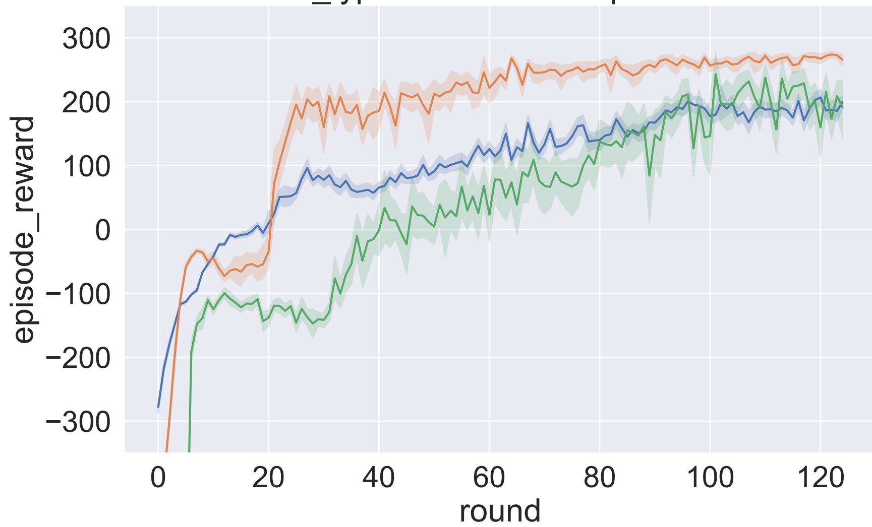
run_type = DP-FedRL Eps=5000
