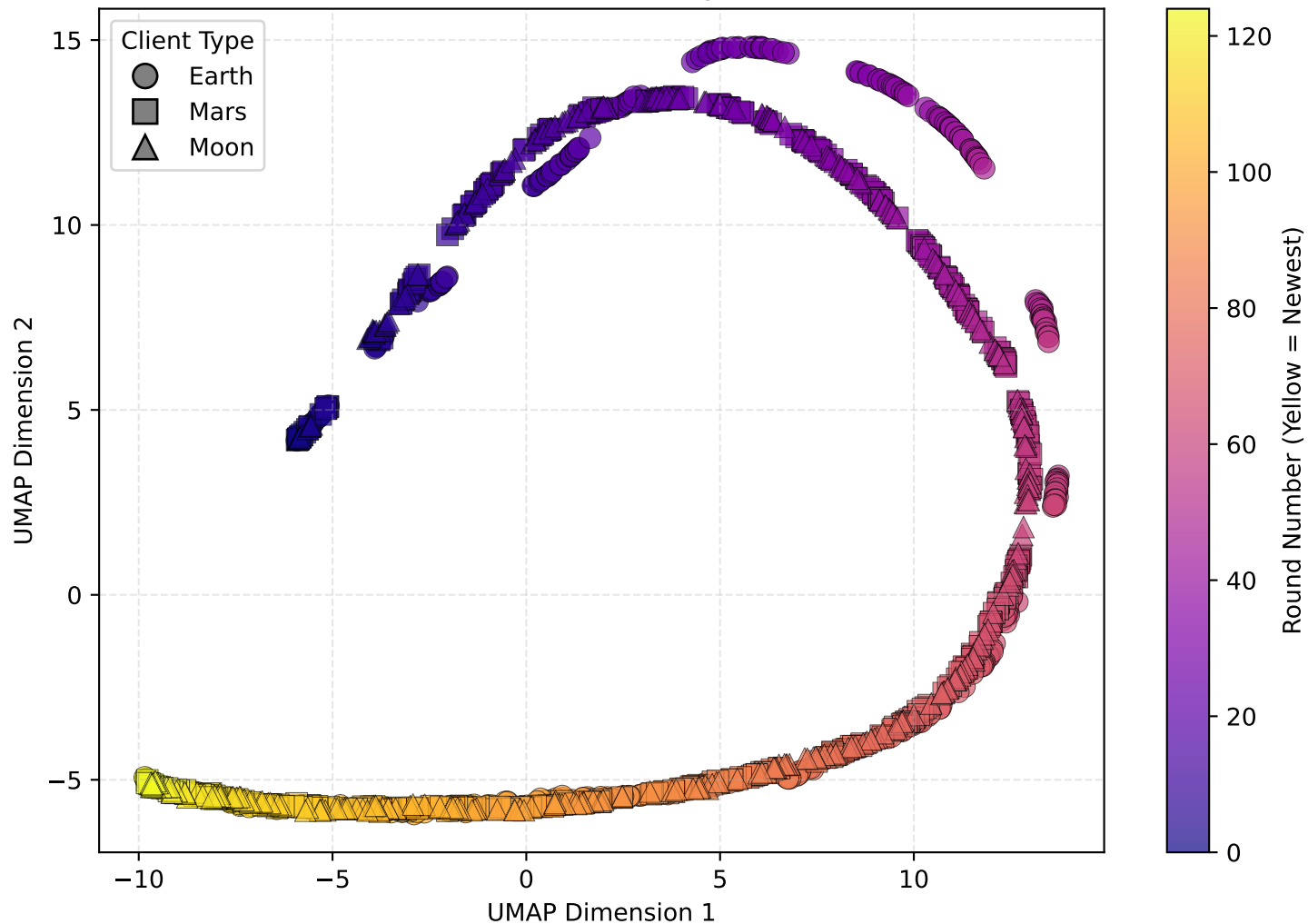
Differentially Private FL EPS=5000: UMAP Trajectory K-Means Identifiability: 59%
