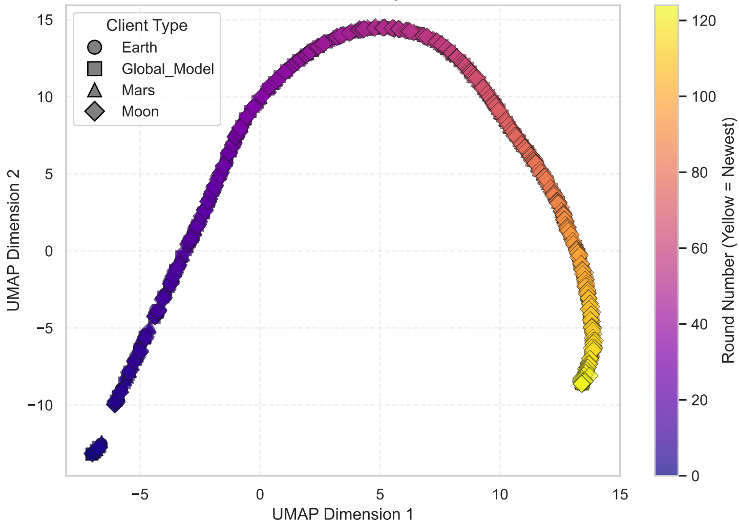
Differentially Private FL EPS=1000: UMAP Trajectory K-Means Identifiability: 35%
