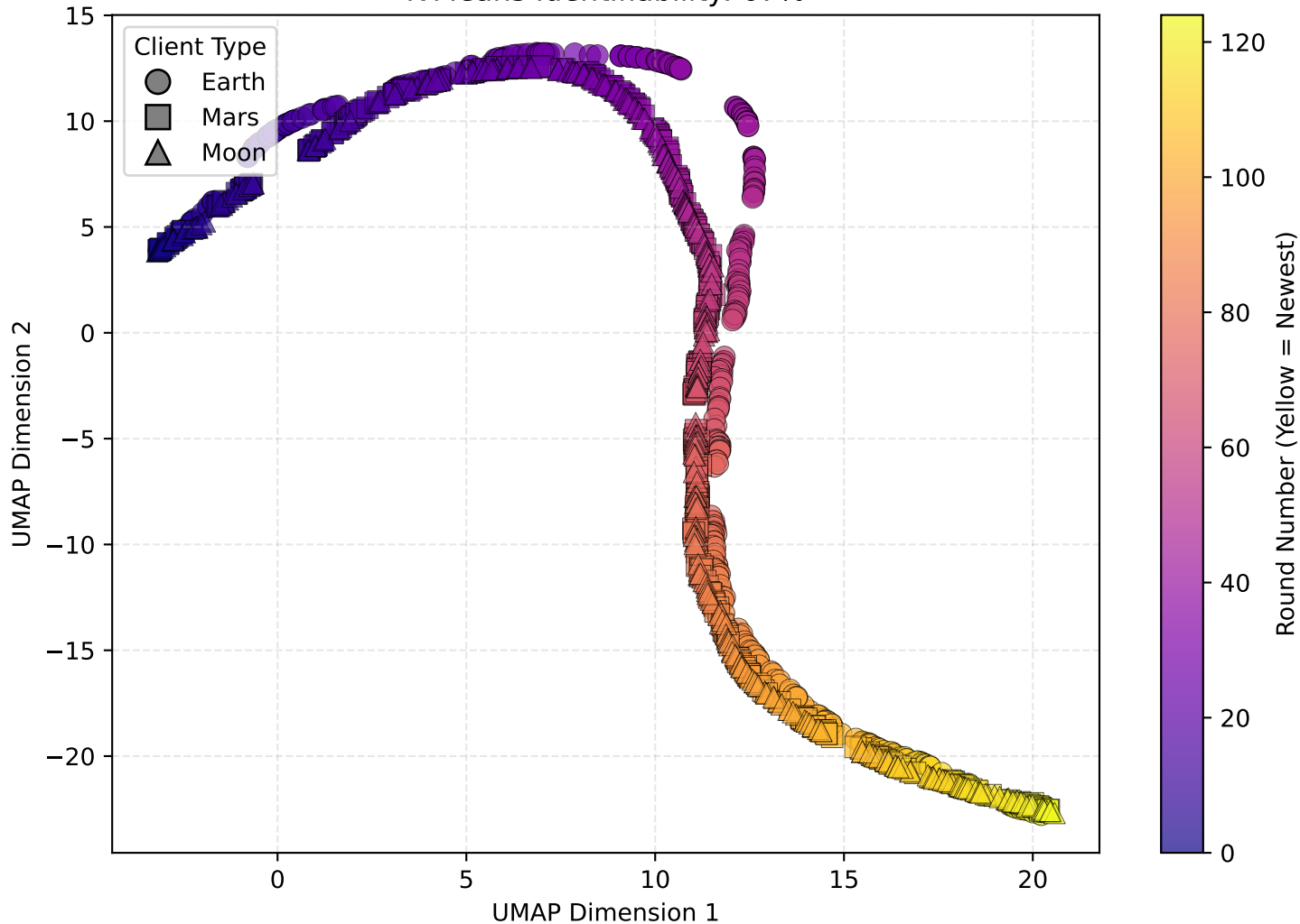
Standard FL: UMAP Trajectory K-Means Identifiability: 67%
