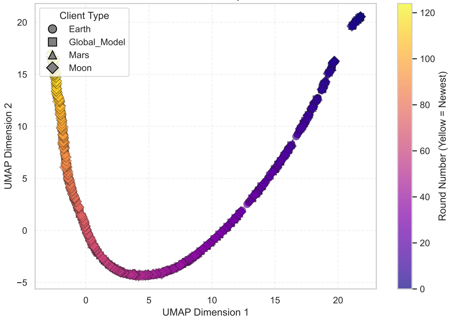
Differentially Private FL EPS=5000: UMAP Trajectory K-Means Identifiability: 33%
