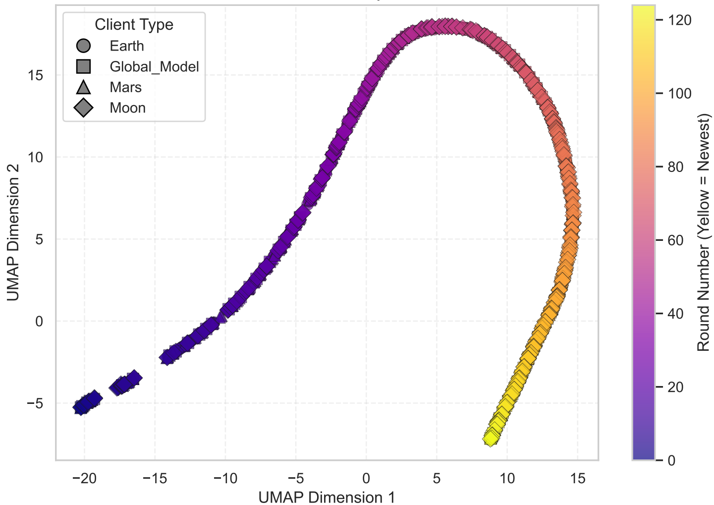
Differentially Private FL EPS= 500: UMAP Trajectory K-Means Identifiability: 32%
