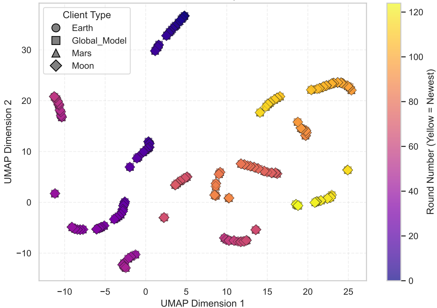
Differentially Private FL EPS=100: UMAP Trajectory K-Means Identifiability: 28%
