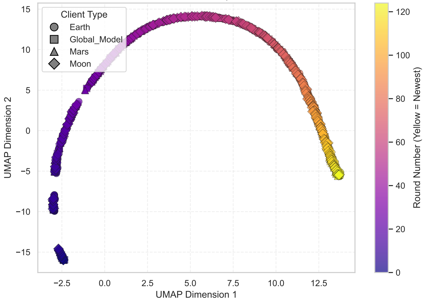
Standard FL: UMAP Trajectory K-Means Identifiability: 36%
