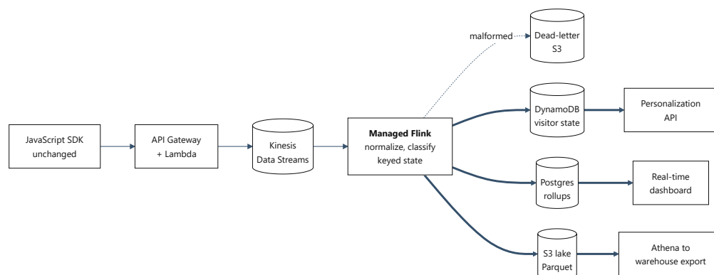
Figure 1. SDK to dashboard. The dead-letter branch is drawn deliberately: a malformed record must never stop the consumer.
