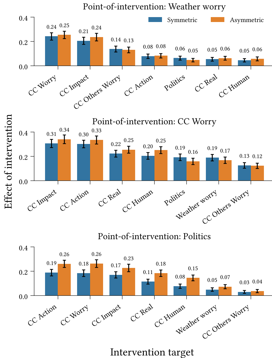
Figure 7.4: Outbound effect of intervention (Definition 6.5.1) at each target spin for interventions targeting Weather Worry , CC Worry , and Politics , in symmetric and asymmetric belief system models calibrated to the climate beliefs dataset. Intervention strength: \delta_h = 2.5 . Confidence intervals display 1.96 standard deviations around the mean effect, measured across 500 repeated simulations.
