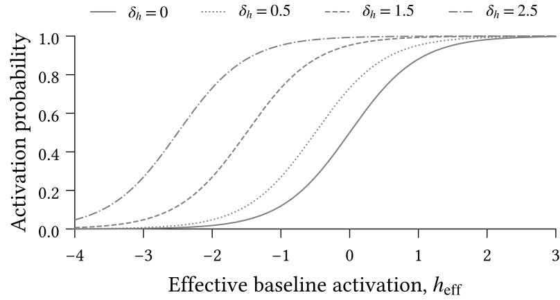
Figure 6.3: Impact of different intervention strengths ( \delta_h \in \{0, 0.5, 1.5, 2.5\} ) on activation probability for the intervention spin. Activation probability is calculated using Equation 3.5.
