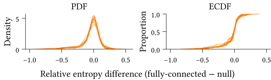
Figure 5.9: Probability density function (left) and empirical cumulative distribution function (right) of the mean difference in relative entropy between the fully-connected and null (only self-interaction) models across survey participants. Negative values indicate lower relative entropy for the fully-connected model.
