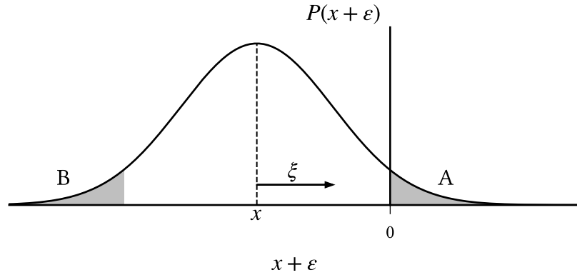
Figure 4.1: Soft thresholding maps x \in \mathbb{R} to \{-1, +1\} by sign-thresholding x' = (x + \varepsilon) where (x + \varepsilon) \sim \mathcal{N}(x, \xi) . Negative values are mapped to +1 with probability P(x' > 0) = A = B = P(\varepsilon < x) , which increases with \xi and |x|^{-1} .
