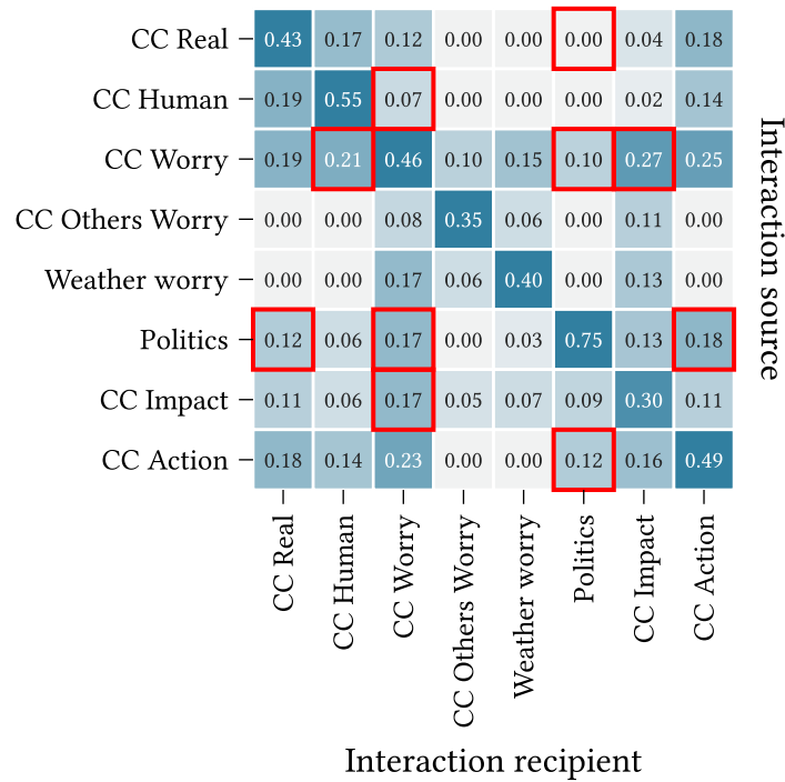
Figure 7.2: Interaction effect matrix ( \mathbf{J} ) for the asymmetric belief system model calibrated to the full climate beliefs dataset. Red borders indicate significant asymmetric pairs. The matrix is otherwise identical to the asymmetric interaction matrix in Figure 5.4.
