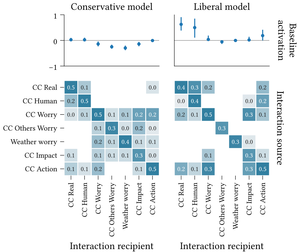
Figure 8.3: (Top) Baseline activations, \mathbf{h} , and (Bottom) interaction effect matrices ( \mathbf{J} ) for asymmetric belief systems calibrated to the conservative ( n = 507 ) and liberal ( n = 375 ) subsets of the climate beliefs dataset (Chapter 12) using the parameter estimation method in Section 4.2.
