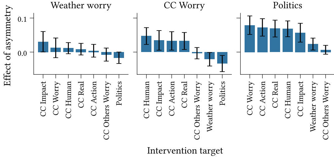
Figure 7.5: Outbound effect of asymmetry (Definition 6.5.2) at each target spin for interventions on Weather Worry , CC Worry , and Politics , for models calibrated to the climate beliefs dataset. Intervention strength: \delta_h = 2.5 . Confidence intervals display 1.96 standard deviations around the mean effect of asymmetry ( n = 500 ).
