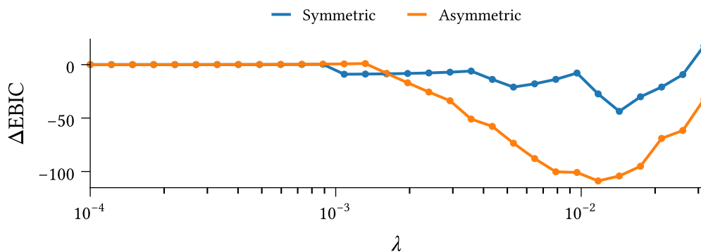
Figure 5.3: Effect of regularisation strength \lambda on Extended Bayesian Information Criterion for symmetric and asymmetric belief system models optimised to the climate beliefs dataset using Equation 4.6. The vertical axis measures the difference in EBIC compared to the no-regularisation case ( \lambda = 0 ); smaller is better.
