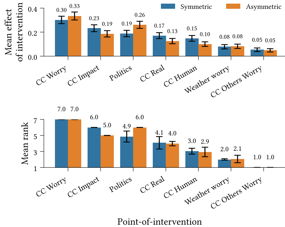
Figure 7.6: Inbound mean effect of intervention (Definition 6.5.1) ( Top ) and mean rank ( Bottom ) for interventions targeting CC Action. Ranks are calculated per-repeat with respect to the average effect of intervention—higher values are assigned higher ranks. Confidence intervals display 1.96 standard deviations ( n = 500 ).
