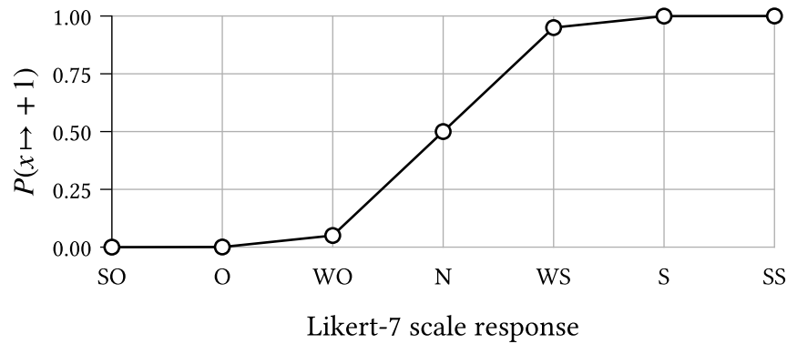
Figure 5.2: The probability of binarisation to +1 for each possible Likert-7 scale survey response, 4 using a soft thresholding function b_\xi as defined in Equation 4.2 with \xi \approx 0.2 .
