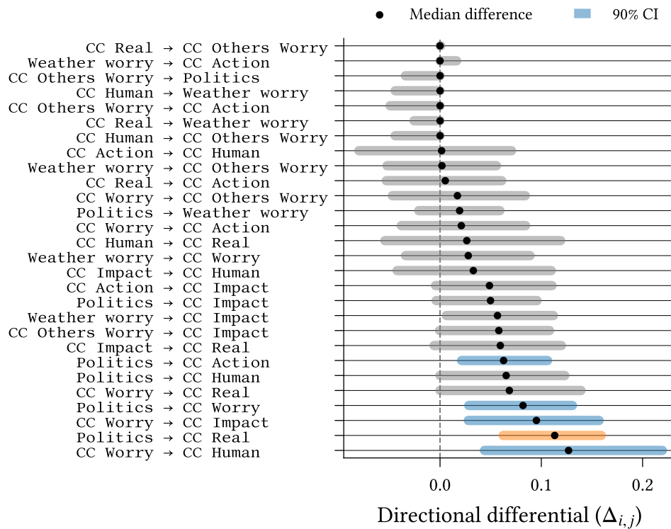
Figure 7.1: Directional differentials—the difference between directed interaction effects for a pair of spins—in reverse order of median value. Confidence intervals are calculated using the percentile method on models calibrated using bootstrapping ( n = 500 ). Grey confidence intervals indicate absence of significant asymmetry. For cases with significant asymmetry, the colour indicates that one (orange) or both (blue) of the directed interaction effects are nonzero.
