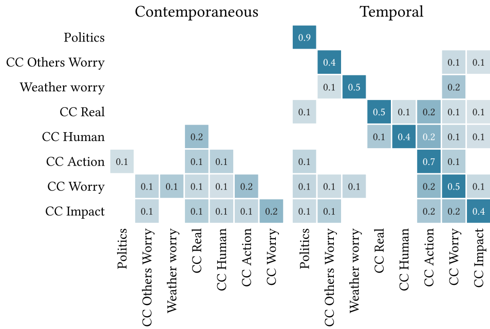
Figure 12.8: Contemporaneous and temporal network matrices for the climate beliefs dataset. Entries in row i of the temporal matrix are the regression predictors for the subsequent value of variable X_i . Rows and columns are ordered using hierarchical clustering on the temporal matrix: d_{\mathbf{K}}(X, Y) = 1 - |\mathbf{K}| .
