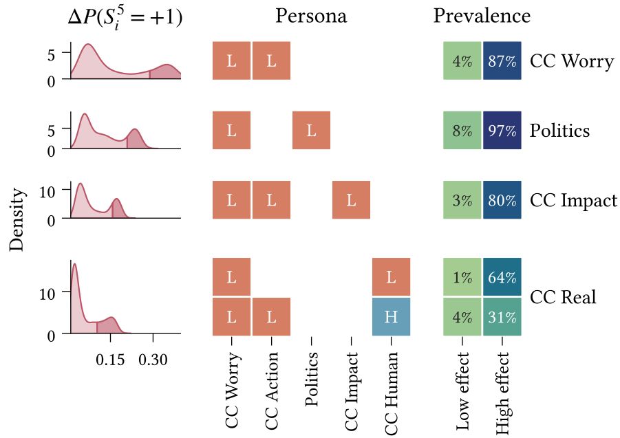
Figure 8.2: Pre-intervention states, or ‘personas’, for which interventions on different beliefs (rows) are most effective for changing attitudes toward climate action in the asymmetric KBS model calibrated to the climate beliefs dataset. The left panel shows the distribution of changes in activation probability for the CC Action belief at t = 5 (approximately two and a half years) using a strong intervention ( \delta_h = 2.5 ), with respect to the no-intervention scenario. The center panel shows the personas corresponding to those individuals in the upper quartile of effects (shaded region in the left panel). Rows are distinct personas. Cells correspond to intervals in the initial state space dimensions, i.e., the different beliefs, with L = [-1, 0] and H = [0, +1] . The right panel shows each persona’s prevalence within the upper quartile (‘High-effect’) and below the upper quartile (‘Low-effect’) of effects. Personas are identified using depth-3 regression decision trees fit with a mean-squared error objective and mean effect of intervention on influence as the response variable ( n = 500 ). R^2 > 0.9 for all decision trees, measured using 10-fold cross validation.
