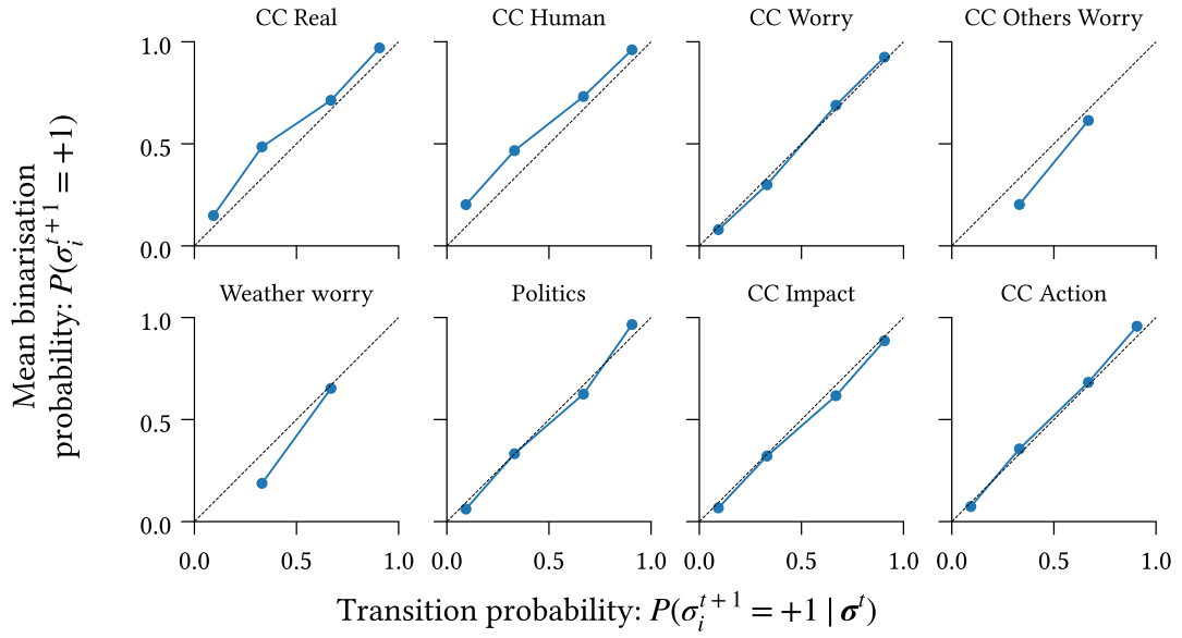
Figure 5.7: Reliability of transitions predicted by the model measured as the agreement between conditional probabilities under the model, P_{\mathcal{M}}(\sigma_i^{t+1} = +1 | \sigma^t) , and expected proportion of +1 values after binarisation, calculated as the average transition probability for survey participants in a given conditional probability bin.
