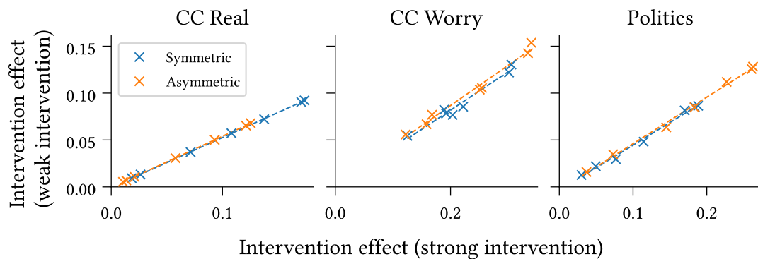
Figure 7.3: Weak ( \delta_h = 0.5 ) and strong ( \delta_h = 2.5 ) interventions exhibit strong positively correlated effects of intervention, consistently across points-of-intervention (panels) and intervention targets (scatterplots). This finding holds for both symmetric and asymmetric models calibrated to the climate beliefs dataset.
