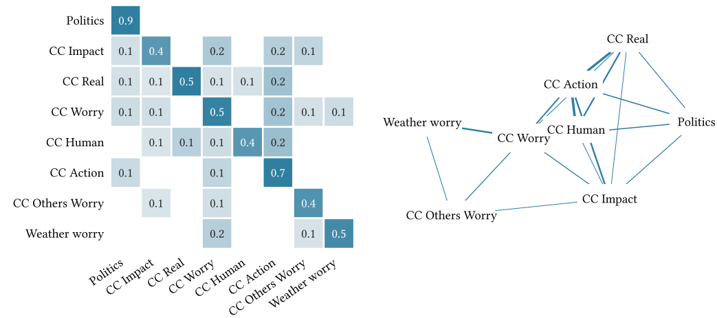
Figure 9.8: Temporal
