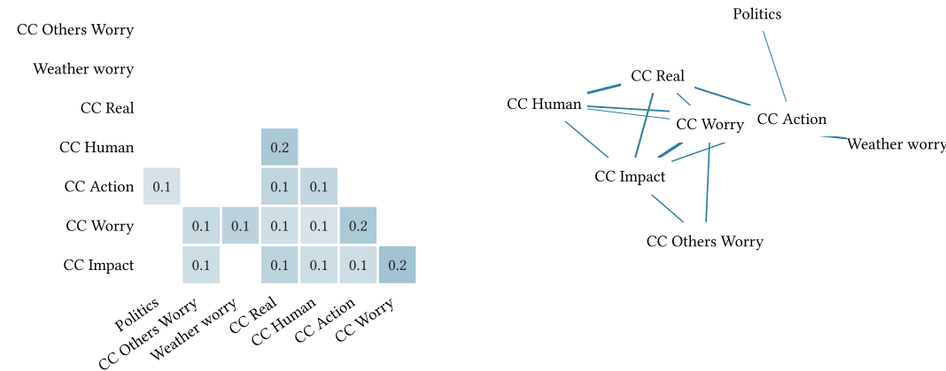
Figure 9.9: Contemporaneous
