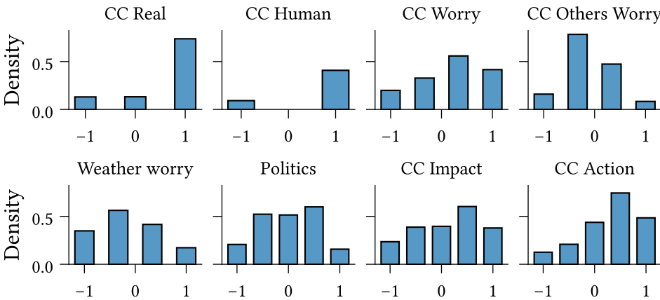
Figure 9.10: TODO
