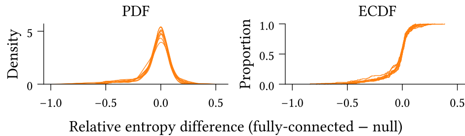
Figure 4.8: Probability density function (left) and empirical cumulative distribution function (right) of the mean difference in relative entropy between the fully-connected and null (only self-interaction) models across survey participants. Negative values indicate lower relative entropy for the fully-connected model.
