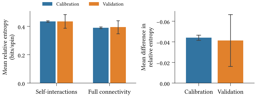
Figure 4.7: (Left) Mean absolute relative entropy of the binarised dataset with respect to the calibrated model, for the full-connected and null (only self-interactions) models, using 10-fold cross-validation. Average calculated across spins and survey participants. (Right) Mean difference in relative entropy. Confidence intervals display two standard deviations around the mean value.
