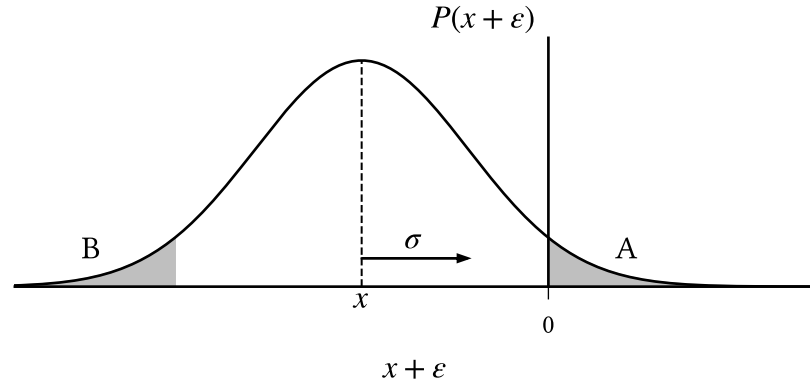
Figure 3.1: Soft thresholding maps x \in \mathbb{R} to \{-1, +1\} by sign-thresholding x' = (x + \varepsilon) where (x + \varepsilon) \sim \mathcal{N}(x, \sigma) . Negative values are mapped to +1 with probability P(x' > 0) = A = B = P(\varepsilon < x) , which increases with \sigma and |x|^{-1} .
