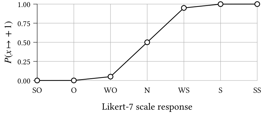
Figure 3.2: The probability of binarisation to +1 for each possible response to a Likert-7 scale survey question 1 , given \sigma \approx 0.2 .
