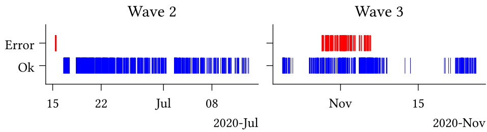
Figure 10.4: Systematic ( left ) and unresolved ( right ) null-value validation errors identified in Waves 2 and 3 of the Longitudinal Panel of Perceptions About Climate Change and Covid survey.
