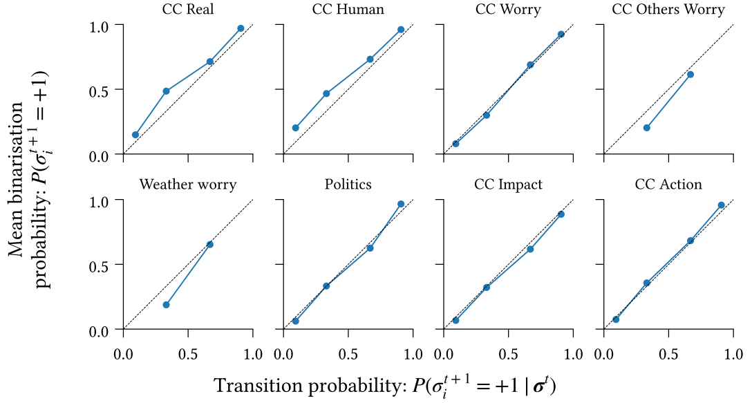
Figure 4.7: Reliability of transitions predicted by the model measured as the agreement between conditional probabilities under the model, P_{\mathcal{M}}(\sigma_i^{t+1} = +1 \mid \sigma^t) , and expected proportion of +1 values after binarisation, calculated as the average transition probability for survey participants in a given conditional probability bin.
