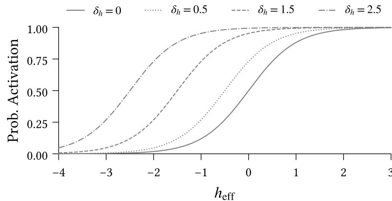
Figure 5.3: Impact of different intervention strengths ( \delta_h \in \{0, 0.5, 1.5, 2.5\} ) on activation probability for the intervention spin. Activation probability is calculated using Equation 2.5.
