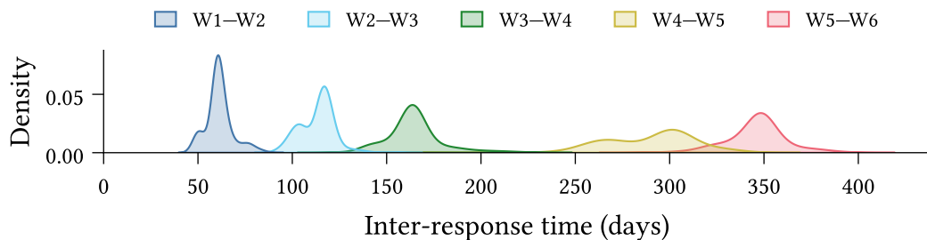
Figure 10.3: Inter-response time distribution between each pair of consecutive waves in the Longitudinal Panel of Perceptions About Climate Change and Covid dataset (prior to dataset cleaning). The inter-response time between two waves is calculated, for individuals present in both waves, as the number of days between their responses.
