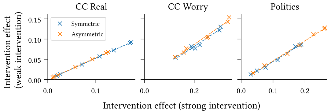
Figure 6.3: Weak ( \delta_h = 0.5 ) and strong ( \delta_h = 2.5 ) interventions exhibit strong positively correlated effects of intervention, consistently across points-of-intervention (panels) and intervention targets (scatterplots). This finding holds for both symmetric and asymmetric models calibrated to the climate beliefs dataset.
