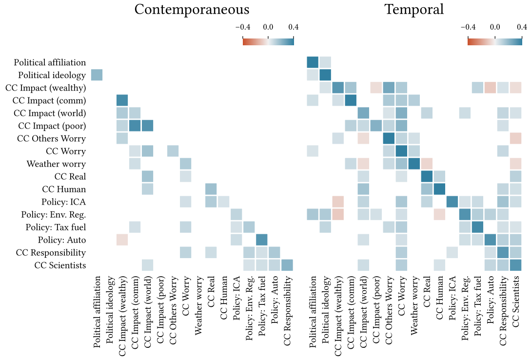
Figure 10.6: Contemporaneous (left) and temporal (right) network matrices for the filtered candidate set. Entries in row i of the temporal matrix are the regression predictors for the subsequent value of variable X_i . Rows and columns are ordered using hierarchical clustering on the temporal matrix: d_K(X, Y) = 1 - |\mathbf{K}| .
