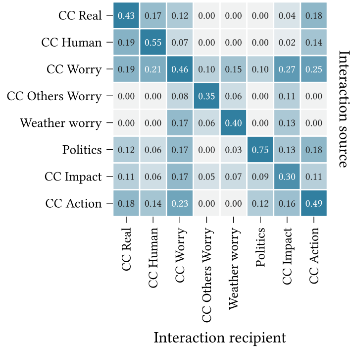
Figure 6.2: Interaction effect matrix ( \mathbf{J} ) for the asymmetric belief system model calibrated to the full climate beliefs dataset. This figure is identical to the asymmetric interaction matrix in the previous chapter (Figure 4.4).
