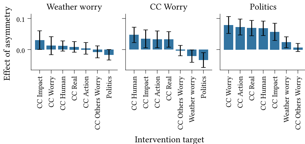
Figure 6.5: Outbound effect of asymmetry (Definition 5.5.2) at each target spin for interventions on Weather Worry , CC Worry , and Politics , for models calibrated to the climate beliefs dataset. Intervention strength: \delta_h = 2.5 . Confidence intervals display 1.96 standard deviations around the mean effect of asymmetry ( n = 500 ).
