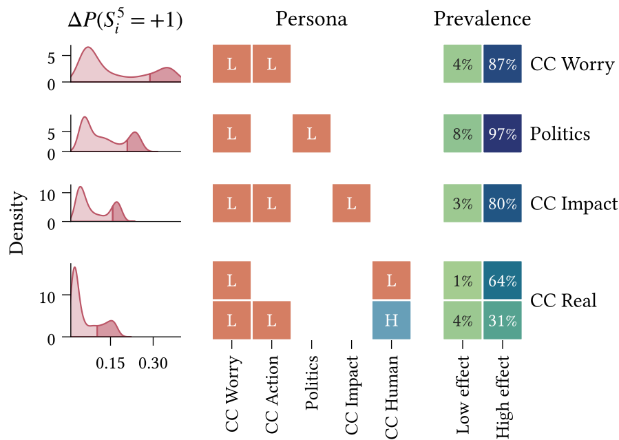
Figure 7.2: Pre-intervention states ('personas') for which interventions on different beliefs (rows) are most effective for changing attitudes toward climate action in the asymmetric KBS model calibrated to the climate beliefs dataset. The left panel shows the distribution of changes in activation probability for the CC Action belief at t = 5 (approximately two and a half years) using a strong intervention ( \delta_h = 2.5 ), with respect to the no-intervention scenario. The center panel shows the personas corresponding to those individuals in the upper quartile of effects (shaded region in the left panel), identified using a depth-3 regression decision tree. Rows are distinct personas. Cells correspond to intervals in the initial state space dimensions, i.e., the different beliefs, with L = [-1, 0] and H = [0, +1] . The right panel shows the prevalence of each persona within the upper quartile ('High-effect') and below the upper quartile ('Low-effect') of measured effects.
