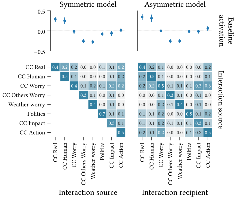
Figure 4.2: (Top) Baseline activations, \mathbf{h} , and (Bottom) interaction effect matrices, \mathbf{J} , for the symmetric and asymmetric belief system model variants, calibrated to the climate beliefs dataset (Chapter 10) using the parameter estimation method in Section 3.2. Error bars on the baseline activations display 95% confidence intervals, calculated over bootstrapped models ( n = 500 ) using the percentile method.
