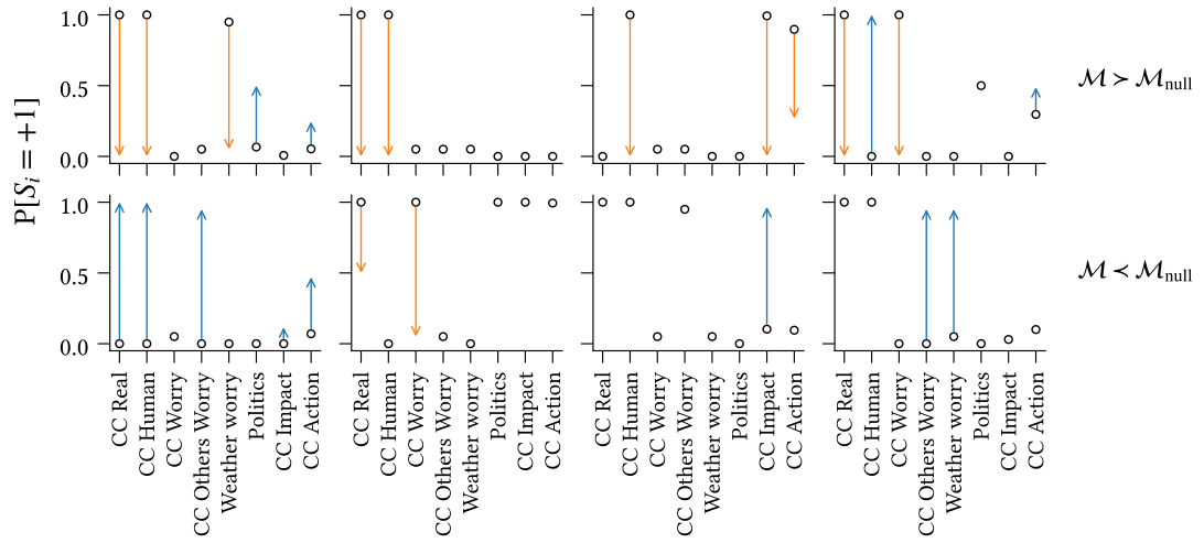
Figure 3.12: Observed transitions for sample survey participants in the left tail (top row) and right tail (bottom row) of Figure 4.7. Circles indicate the probability that participants' observations in the first wave are binarised to +1. Arrows denote the change in the second wave, colour-coded according to whether the change is toward the positive (blue) or negative (orange) state.
