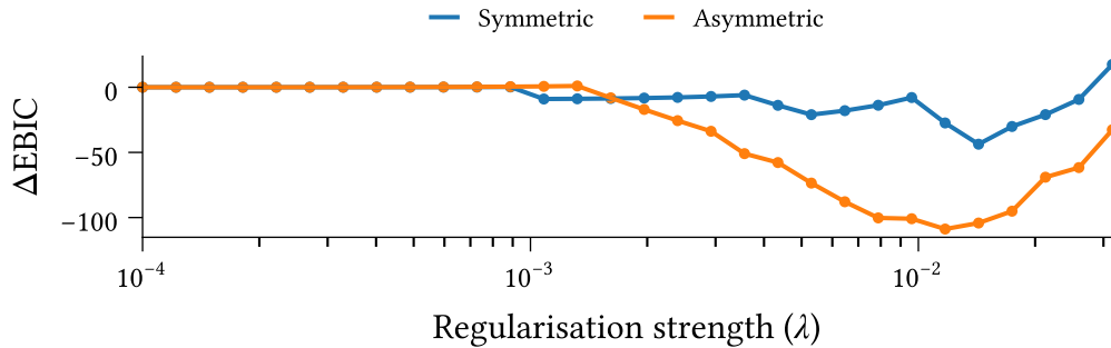
Figure 3.4: Effect of regularisation strength \lambda on Extended Bayesian Information Criterion for symmetric and asymmetric belief system models optimised to the climate beliefs dataset using Equation 3.6. The vertical axis measures the difference in EBIC compared to the no-regularisation case ( \lambda = 0 ).
