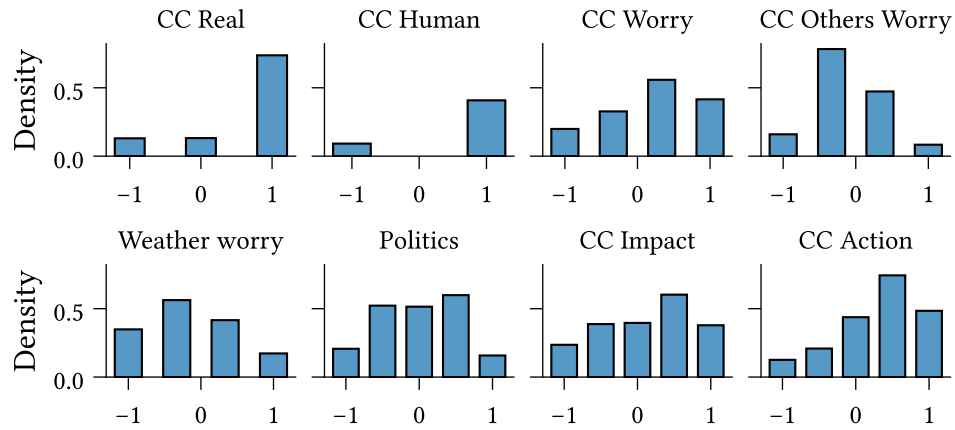
Figure 3.5: Marginal distribution for each of the eight variables in the climate beliefs dataset (Table 4.1). Note that this figure is identical to Figure 10.7 displayed in Chapter 10.
