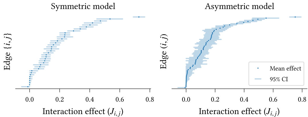
Figure 3.7: Interaction effect parameter accuracy for symmetric and asymmetric models calibrated to the climate beliefs dataset (Chapter 10). Mean parameter values are shown in increasing order. 95% confidence intervals are calculated using the percentile method over models calibrated to bootstrapped datasets (500 repeats).
