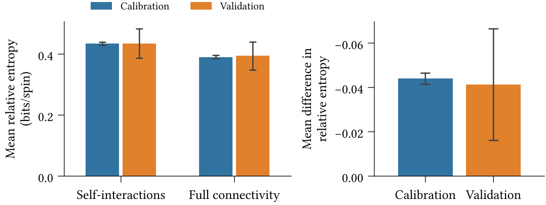
Figure 4.6: (Left) Mean absolute relative entropy of the binarised dataset with respect to the calibrated model, for the full-connected and null (only self-interactions) models, using 10-fold cross-validation. Average calculated across spins and survey participants. (Right) Mean difference in relative entropy. Confidence intervals display two standard deviations around the mean value.
