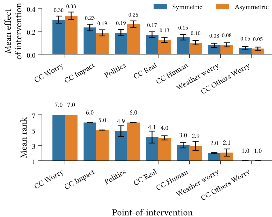
Figure 5.7: Inbound mean effect of intervention ( Definition 5.2.1 ) ( Top ) and mean rank ( Bottom ) for interventions targeting CC Action. Ranks are calculated per-repeat with respect to the average effect of intervention—higher values are assigned higher ranks. Confidence intervals display 1.96 standard deviations ( n = 500 ).
