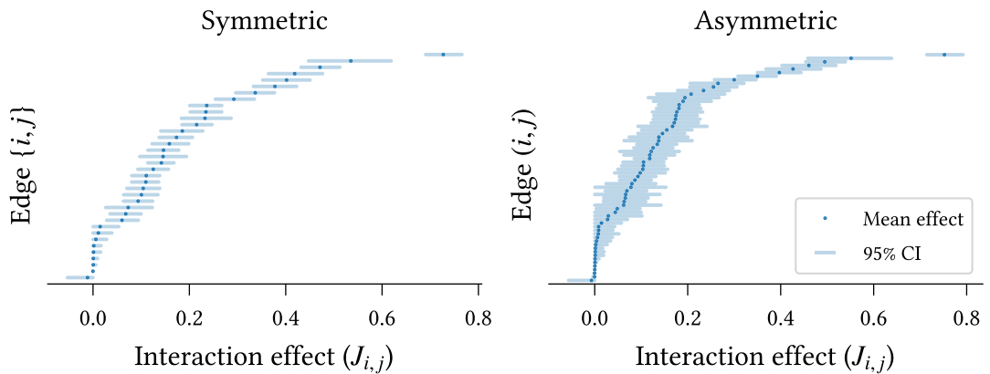
Figure 4.2: Interaction effect parameter accuracy for symmetric and asymmetric models calibrated to the climate beliefs dataset (Chapter 9). Mean parameter values are shown in increasing order. 95% confidence intervals are calculated using the percentile method over models calibrated to bootstrapped datasets (500 repeats).
