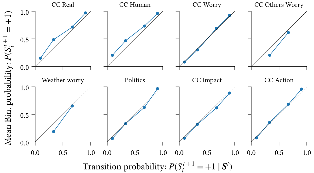
Figure 4.4: Reliability of transitions predicted by the model measured as the agreement between conditional probabilities under the model, P(S_i^{t+1} = +1 | S^t) , and expected proportion of +1 values after binarisation, calculated as the average transition probability for survey participants in a given conditional probability bin.
