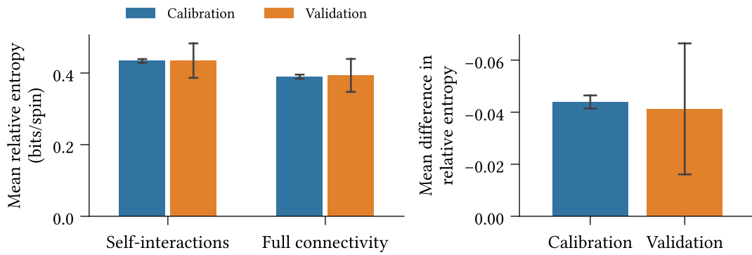
Figure 4.8: (Left) Mean absolute relative entropy of the binarised dataset under the calibrated model, for fully connected and null (only self-interactions) models, using 10-fold cross-validation. Average calculated across beliefs and participants. (Right) Mean difference in relative entropy. Confidence intervals are two standard deviations around the mean.
