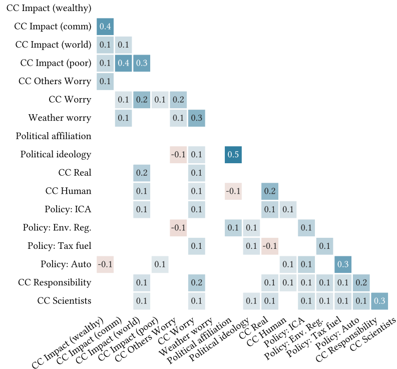
Figure 9.7: Pairwise partial correlation for the filtered candidate set. Cells with |\rho(X, Y)| < 0.05 are masked for visual clarity. Rows and columns are ordered using hierarchical clustering over the distance matrix: d_\rho(X, Y) = 1 - |\rho(X, Y)| .
