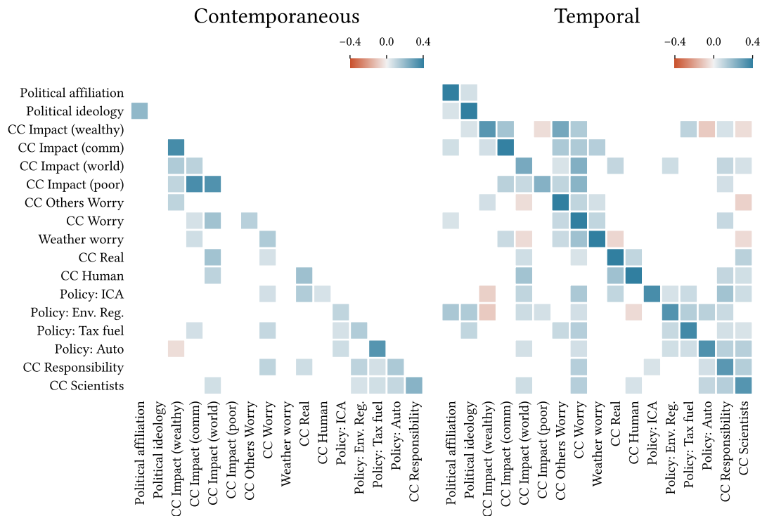
Figure 9.8: Contemporaneous (left) and temporal (right) network matrices for the filtered candidate set. Entries in row i of the temporal matrix are the regression predictors for the subsequent value of variable X_i . Rows and columns are ordered using hierarchical clustering on the distance matrix: d_{\mathbf{K}}(X, Y) = 1 - |\mathbf{K}| .
