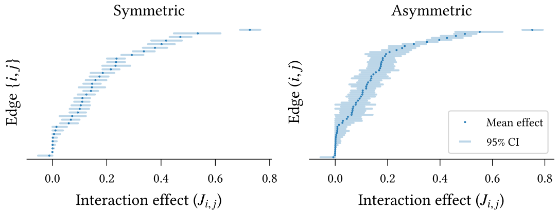
Figure 4.2: Interaction effect parameter accuracy for symmetric and asymmetric models calibrated to the climate beliefs dataset (Chapter 9). Mean parameter values are shown in increasing order. 95% confidence intervals are calculated using the percentile method over models calibrated to bootstrapped datasets (500 repeats).
