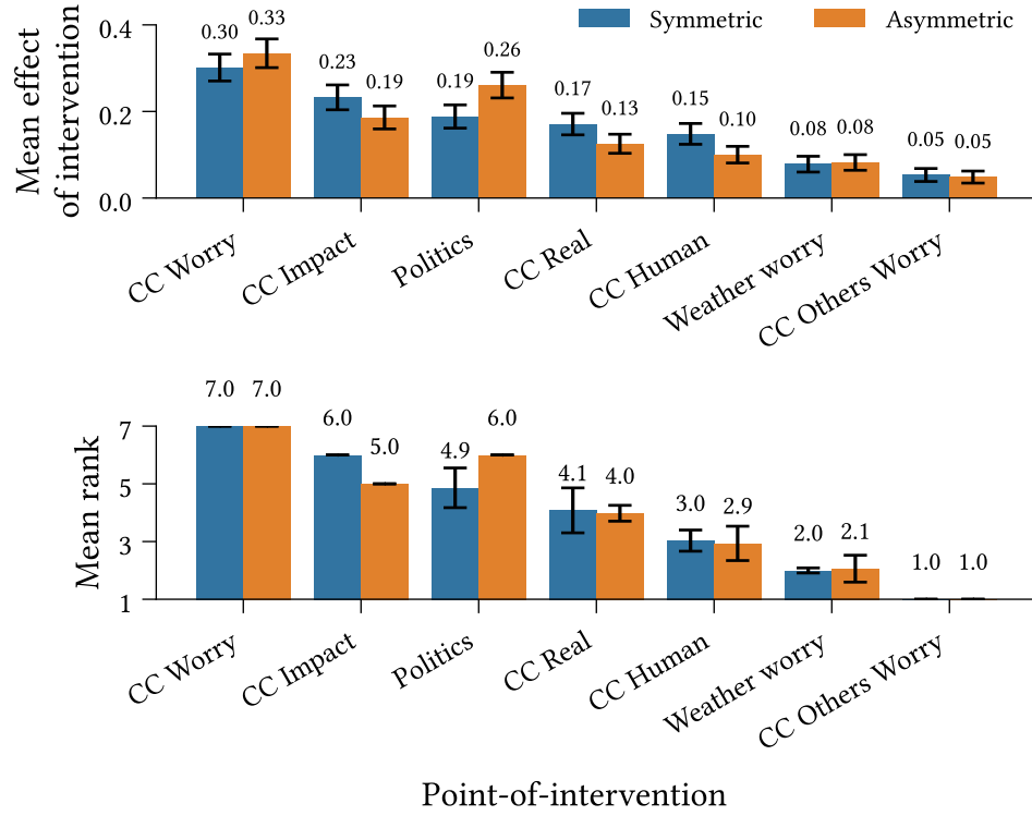
Figure 7.6: Inbound mean effect of intervention (Definition 6.5.1) (Top) and mean rank (Bottom) for interventions targeting CC Action. Ranks are calculated per-repeat with respect to the average effect of intervention—higher values are assigned higher ranks. Confidence intervals display 1.96 standard deviations ( n = 500 ).
