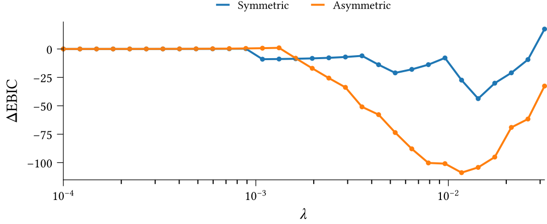
Figure 4.3: Effect of regularisation strength \lambda on Extended Bayesian Information Criterion for symmetric and asymmetric belief system models optimised to the climate attitudes dataset using Equation 4.3. The vertical axis measures the difference in EBIC compared to the no-regularisation case ( \lambda = 0 ).
