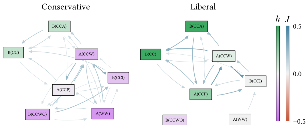
Figure 8.9: Prefixes: A (attitude), B (belief); node labels: CC (climate change), CCA (climate change anthropogenic), CCW (climate change worry), CCWO (climate change worry others), CCI (climate change impacts), CCP (climate change policies), WW (weather worry).
