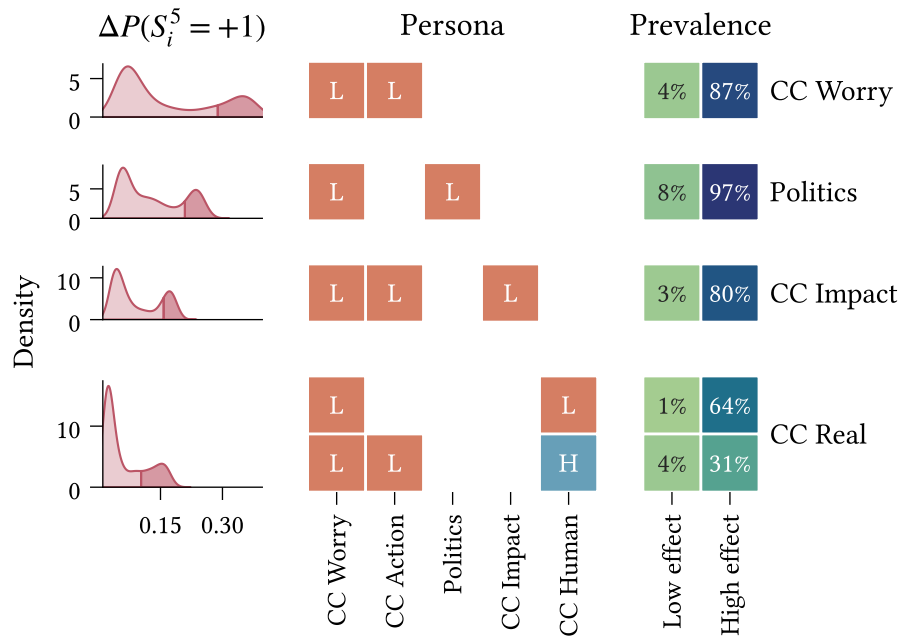
Figure 8.2: Pre-intervention states ('personas') for which interventions on different beliefs (rows) are most effective for changing attitudes toward climate action in the asymmetric KBS model calibrated to the climate beliefs dataset. The left panel shows the distribution of changes in activation probability for the CC Action belief at t = 5 (approximately two and a half years) using a strong intervention ( \delta_h = 2.5 ), with respect to the no-intervention scenario. The center panel shows the personas corresponding to those individuals in the upper quartile of effects (shaded region in the left panel), identified using a depth-3 regression decision tree. Rows are distinct personas. Cells correspond to intervals in the initial state space dimensions, i.e., the different beliefs, with L = [-1, 0] and H = [0, +1] . The right panel shows the prevalence of each persona within the upper quartile ('High-effect') and below the upper quartile ('Low-effect') of measured effects.
