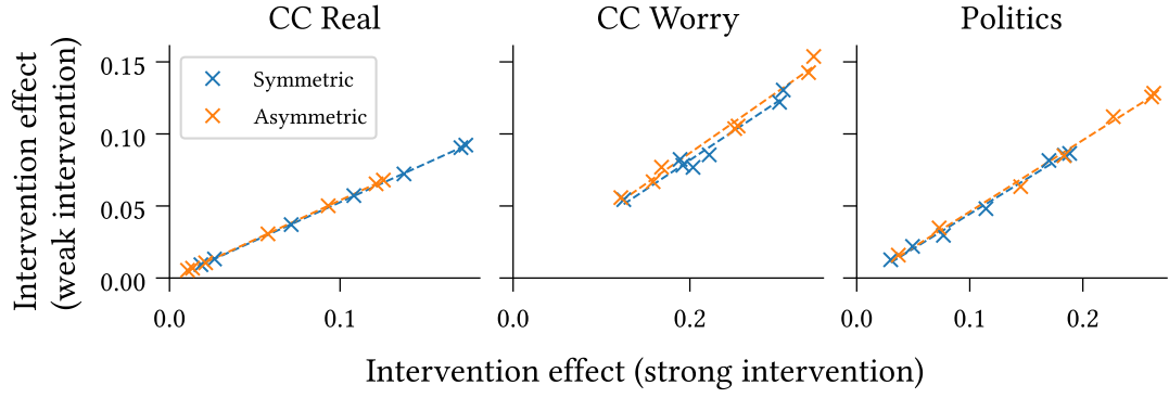
Figure 7.3: Weak ( \delta_h = 0.5 ) and strong ( \delta_h = 2.5 ) interventions exhibit strong positively correlated effects of intervention, consistently across points-of-intervention (panels) and intervention targets (scatterplots). This finding holds for both symmetric and asymmetric models calibrated to the climate beliefs dataset.
