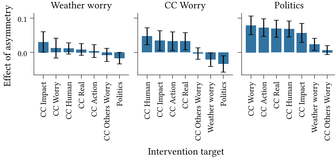
Figure 7.5: Outbound effect of asymmetry (Definition 6.6.2) at each target spin for interventions on Weather Worry , CC Worry , and Politics , for models calibrated to the climate beliefs dataset. Intervention strength: \delta_h = 2.5 . Confidence intervals display 1.96 standard deviations around the mean effect of asymmetry ( n = 500 ).
