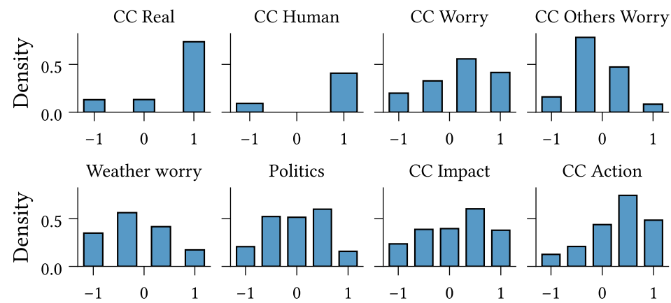
Figure 9.9: TODO
