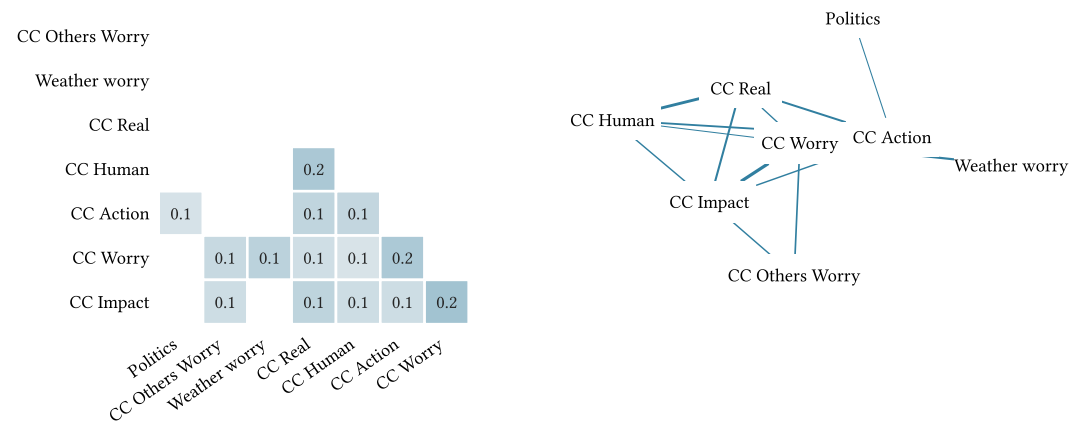
Figure 9.8: Contemporaneous
