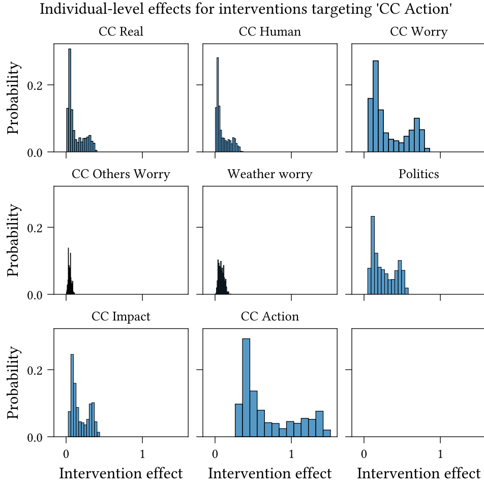
Figure 6.1: The expected effect of intervention for strong interventions ( \delta_h = 2.5 ) targeting ‘Climate Action’ exhibits substantial variation between individuals.
