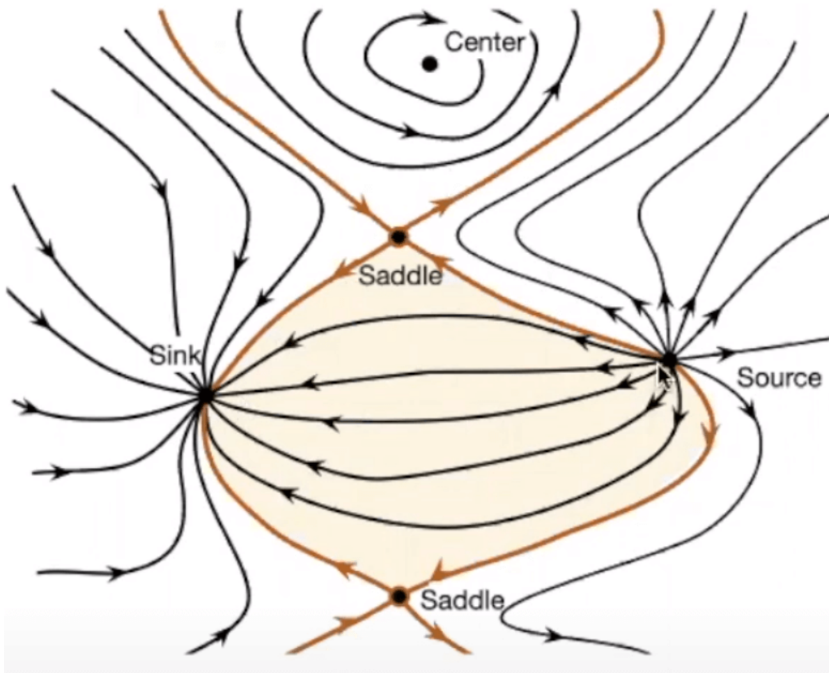
Figure 19.6: Identification of separatrices in 2D.
