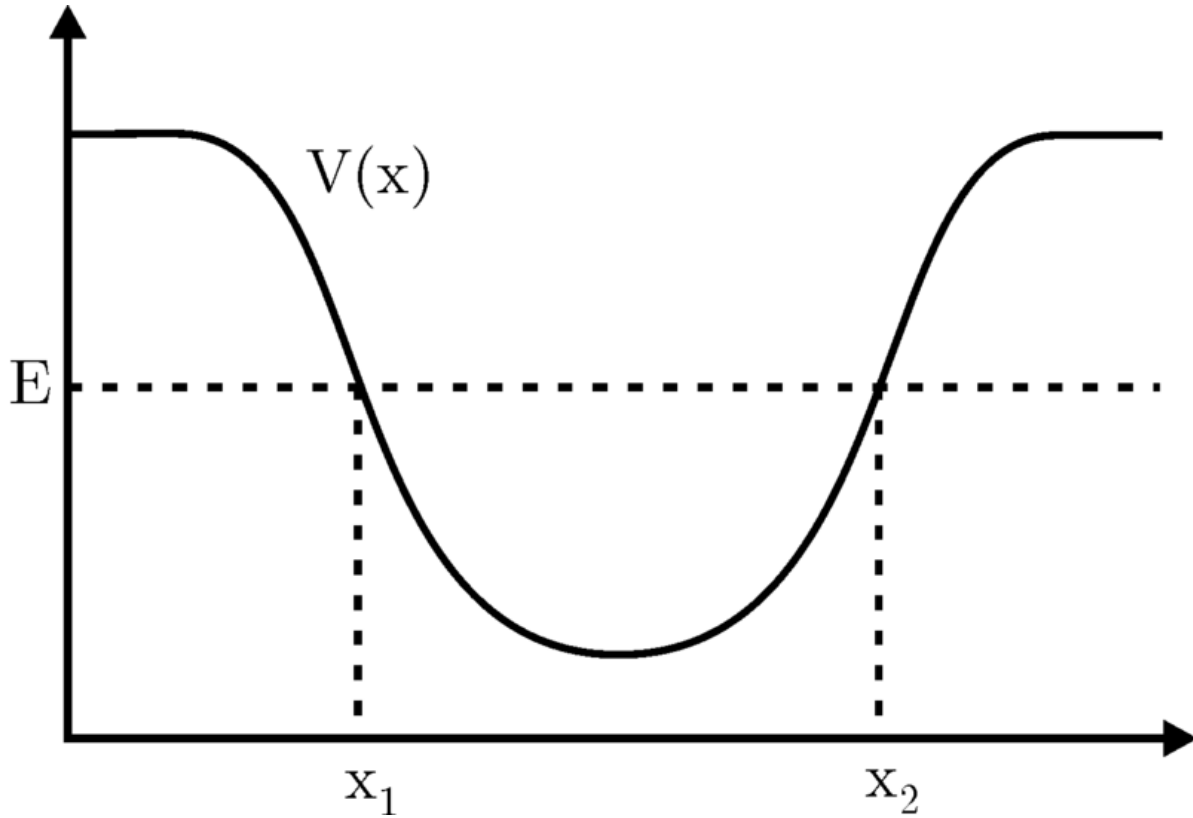
Figure 3.6: Potential well.
