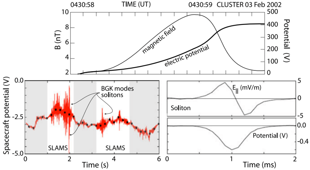
Figure 22.34: Observation of electric field structures in large magnetic pulsations (SLAMS) in the quasi-parallel shock transition region [Behlke et al, 2003, 2004]. Structures on three different time scales are shown, corresponding also to three different spatial scales. Top: CLUSTER passage across on (moderately large amplitude) magnetic pulsation in the shock transition. The (smoothed) magnetic field structure is a slightly steepened magnetic bump. The stationary parallel electric potential field across this structure shows a potential ramp with steep gradient at the leading edge of the pulsation. The potential drop of 400 V corresponds to an electric field of \sim 0.47 \text{ V m}^{-1} . Note that the time scale in this panel is 90 s. Bottom left: Six seconds of a CLUSTER passage through the shock transition. The black dots show the spacecraft potential variation which maps the local density variation. Overlaid is the high frequency WHISPER trace of the plasma frequency. In the magnetic pulsation regions (white) the plasma frequency exhibits huge excursions to both sides similar to those on wave observations. These excursions trace the BGK (non-symmetric) modes and (symmetric) solitons. Bottom right: One example of one of the solitons on a 2 ms time scale. It is nicely seen how symmetric the parallel potential trough and the corresponding bipolar parallel electric field shape look like in the solitary wave structure.
