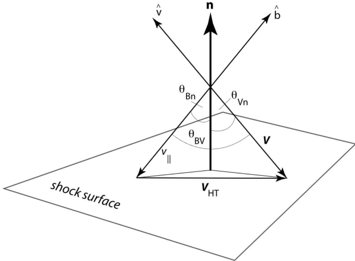
Figure 22.3: The shock coordinate system showing the shock normal \hat{n} , velocity and magnetic field directions \hat{v} , \hat{b} , the three angles \theta_{Bn} , \theta_{Vn} , \theta_{BV} between \hat{b} and \hat{n} , velocity \mathbf{U} and \hat{n} , and velocity \mathbf{U} and \hat{b} , respectively. The velocity \mathbf{V}_{HT} in the shock plane is the deHoffmann-Teller velocity (after Schwartz et al. 1983).
