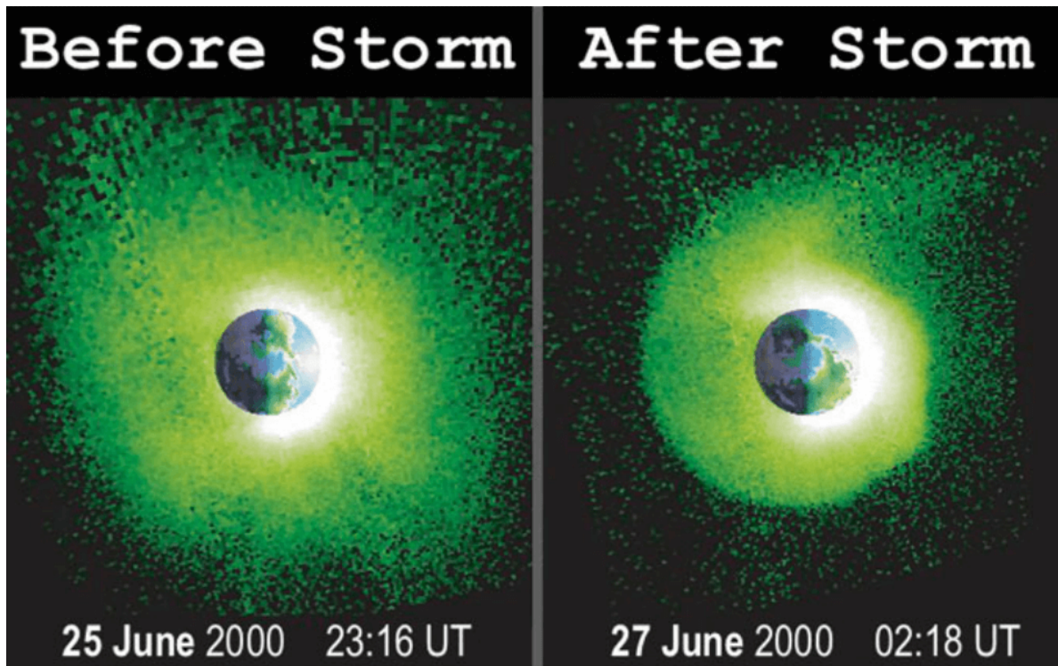
Figure 23.8: Plasmapheric plume and plasmaspheric erosion as observed by the IMAGE EUV instrument. The picture is taken from above the northern hemisphere and the Sun is to the right. (Goldstein+2004)
