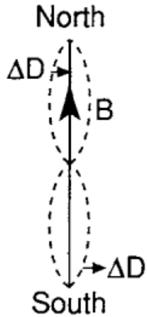
Figure 17.1: Cartoons showing the oscillation of a field line in the two lowest frequency toroidal modes (left) and poloidal modes (right). On the left the field line is drawn stretched out from north to south, and we look towards the Earth as the field line is displaced east and west. On the right, the dipolar field line is displaced within its meridian plane so all magnetic perturbations are radial. Note that for the toroidal mode, the magnetic perturbations ( \Delta D ) have the opposite sense north and south in the fundamental and the same sense in the second harmonic. The opposite is true of the \Delta H perturbation in the poloidal mode.
