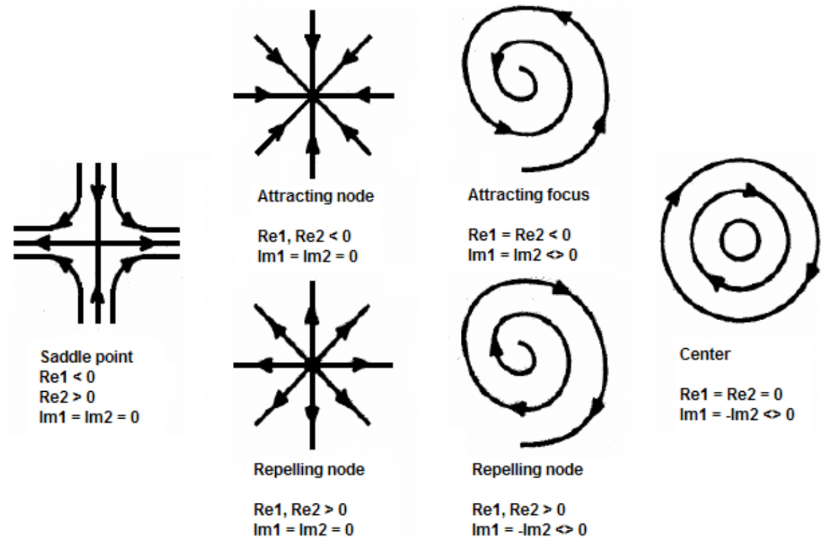
Figure 20.4: Classification of critical points, here Re1/Re2 is the real part of the first/second eigenvalue and Im1/Im2 is the imaginary part of the first/second eigenvalue.
