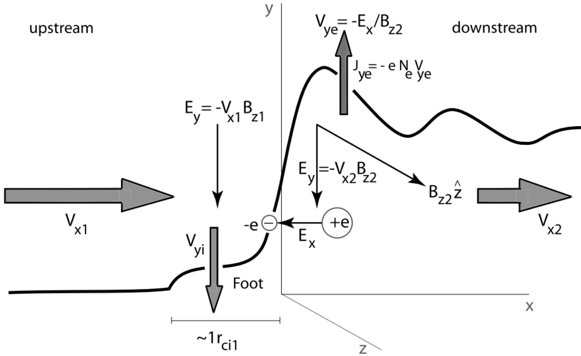
Figure 22.5: Geometry of an ideally perpendicular supercritical shock showing the field structure and sources of free energy. The shock is a compressive structure. The profile of the shock thus stands for the compressed profile of the magnetic field strength |B| , the density N , temperature T , and pressure P = Nk_B T of the various components of the plasma. The inflow of velocity \mathbf{V}_1 and outflow of velocity \mathbf{V}_2 is in the x direction, and the magnetic field is in the z direction. Charge separation over an ion gyroradius r_{ci} in the shock ramp magnetic field generates a charge separation electric field E_x along the shock normal which reflects the low-energy ions back upstream. These ions see the convection electric field E_y of the inflow, which is along the shock front, and become accelerated. The magnetic field of the current carried by the accelerated back-streaming ions causes the magnetic foot in front of the shock ramp. The shock electrons are accelerated antiparallel to E_x perpendicular to the magnetic field. The shock electrons also perform an electric field drift in y -direction in the crossed E_x and compressed B_{z2} fields which leads to an electron current J_y along the shock. These different currents are sources of free energy which drives various instabilities in different regions of the perpendicular shock. (Balogh and Treumann 2013)
