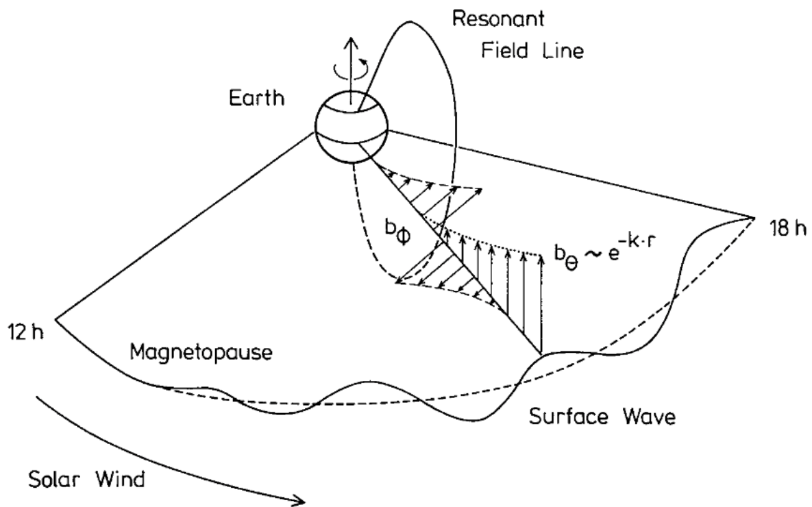
Figure 17.6: Schematic view of the field line resonance, driven by unstable surface wave.
