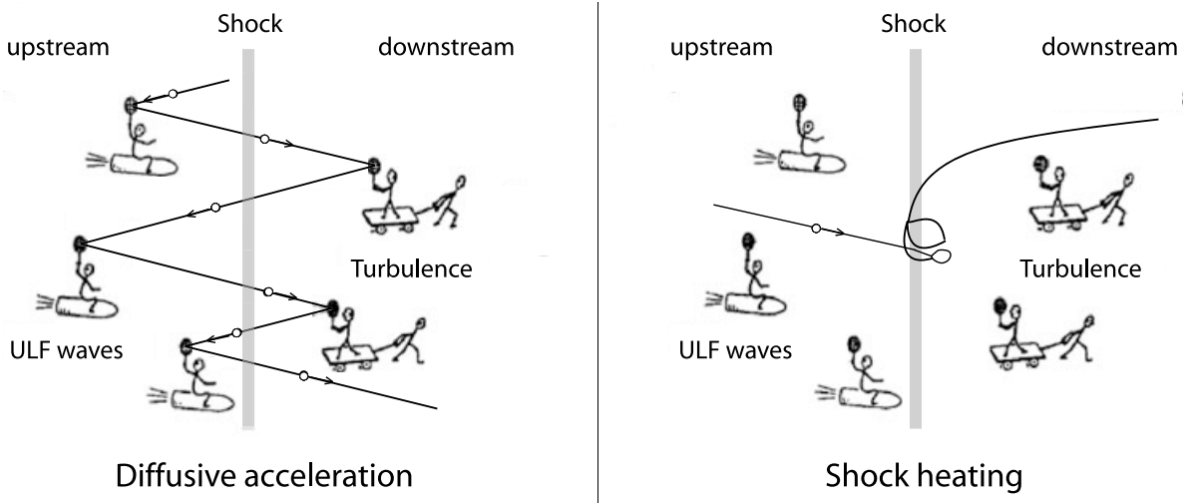
Figure 22.40: Cartoon of the diffusive shock acceleration (left) and shock heating mechanisms [after an sketch by M. Scholer and Hoshino]. In diffusive shock acceleration the particle is scattered around the shock being much faster than the shock. The requirement is the presence of upstream waves and downstream turbulence or waves. In shock heating the particle is a member of the main particle distribution, is trapped for a while at the shock and thereby thermalised and accelerated until leaving the shock.
