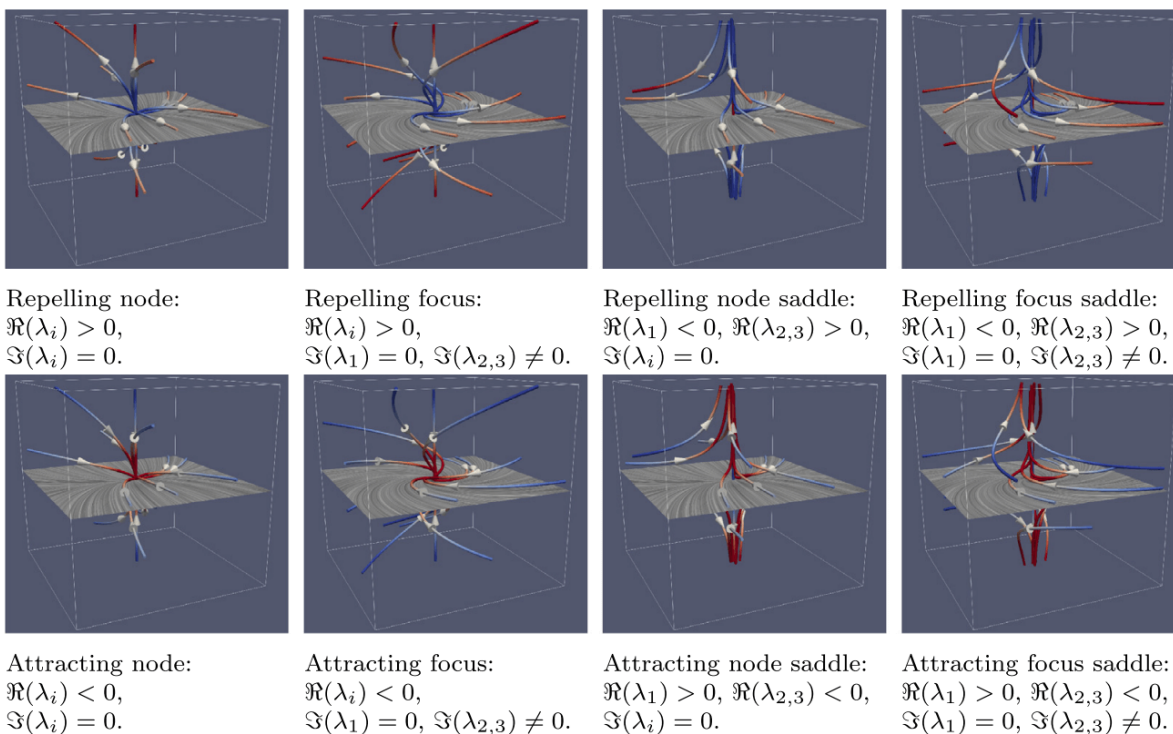
Figure 20.5: The different types of nondegenerate 3D critical points visualized with streamlines color coded in red/blue for forward/backward integration and line integral convolution in the plane of the common sign. Here the presence of the subscript i means all i \in (1, 2, 3) , and the order of the eigenvalues does not matter.
