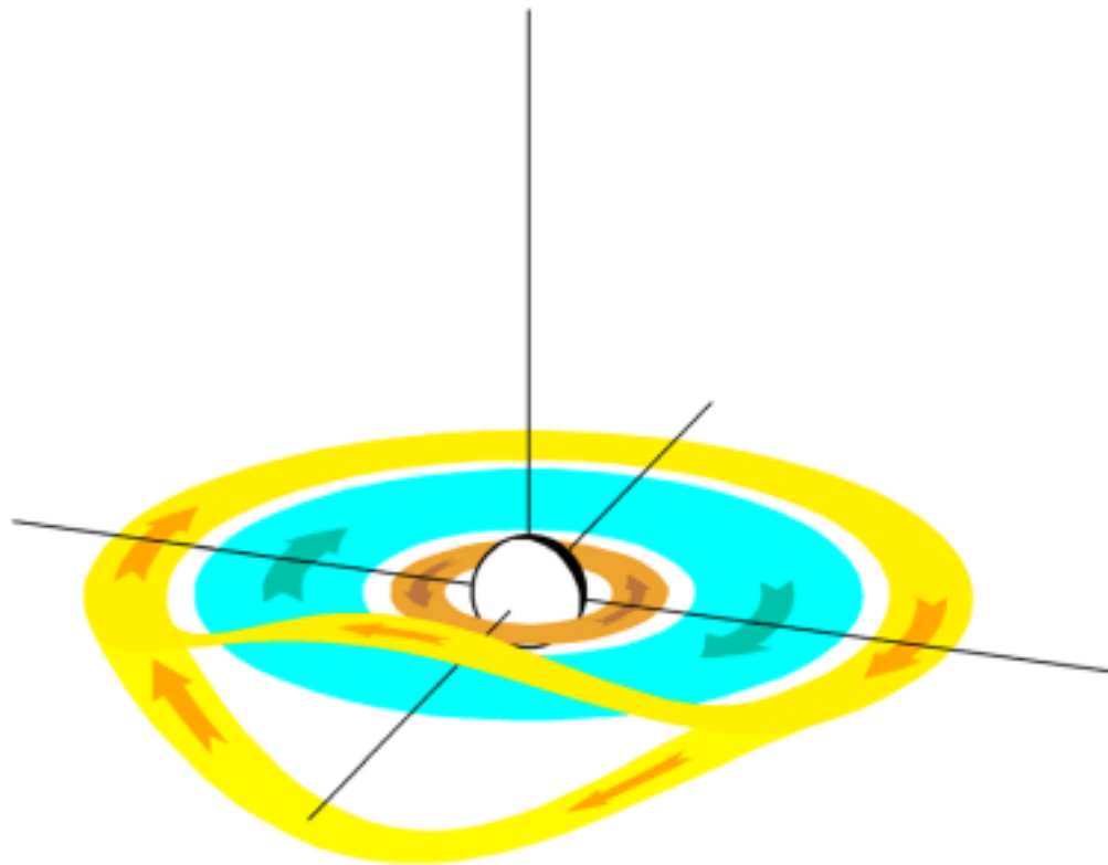
Figure 23.4: The symmetric ring current (eastward and westward, in brown and blue, respectively) including the cut ring currents on the dayside (in yellow). The viewing perspective is the same as in Figure 23.2 but now zoomed in closer to the Earth.
