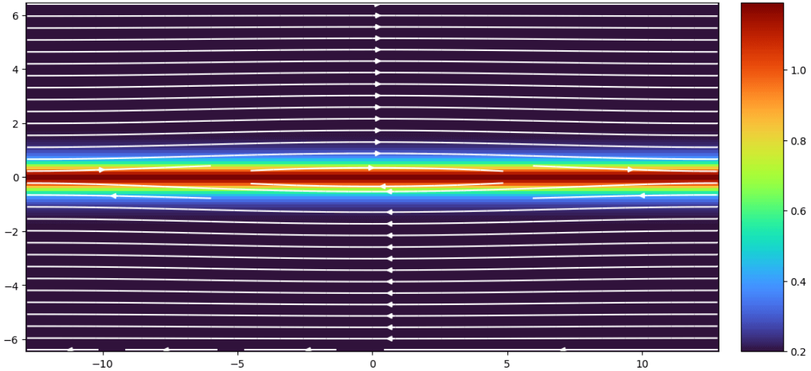
Figure 34.1: Initial density and magnetic field in the GEM current sheet setup.
