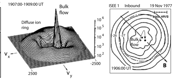
Figure 22.18: Left: A two-minute average pseudo-3D ion velocity-space profile in the (v_x, v_y) -plane showing the undisturbed and cold (narrow) plasma inflow in negative v_x -direction about centred and surrounded by a ring distribution of fast and warm (broad) diffuse ions that have been reflected from the shock but have been processed in the foreshock region when propagating from the foreshock boundary into the foreshock. These ions are hollow in the sense that they separate from the bulk distribution but have a nearly isotropic distribution function. Right: Contour plot of a similar ring a little earlier showing that the ring centre (star) is slightly displaced from the bulk flow (dot) on the magnetic field that connects to the shock and from the centre (cross) of the phase space frame.
