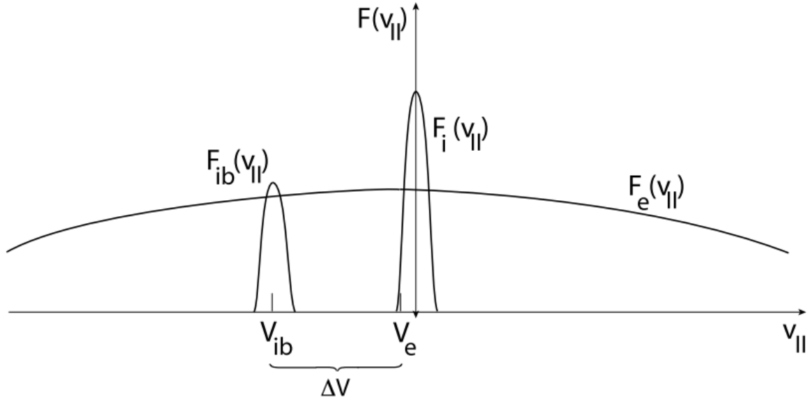
Figure 22.20: Reduced parallel distribution functions along the ion-foreshock boundary showing the cold main flow ion distribution F_i(v_{\parallel}) , the hot main flow electron distribution F_e(v_{\parallel}) shifted to the left into the direction of the foreshock ion beam for keeping zero-current conditions, and the ion-foreshock ion beam distribution F_{ib}(v_{\parallel}) . This configuration is unstable with respect to ion-ion beam instabilities and the ion-beam driven ion-acoustic instability.
