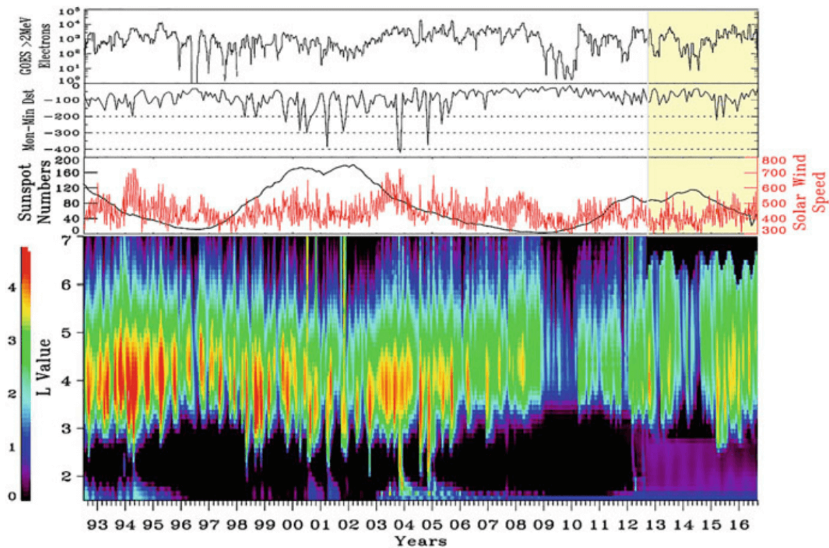
Figure 23.9: Outer radiation belt response to solar and magnetospheric activity from the SAMPEX satellite and Van Allen Probes observations over a period of more than two solar cycles. The uppermost panel shows 27-day window-averaged relativistic ( >2 MeV) electron fluxes at geostationary orbit, the second panel the monthly minimum of the Dst index, and the third panel the yearly window-averaged sunspot number (black) and weekly window-averaged solar wind speed (red). The spectrogram in the lowest panel is a composite of 27-day window-averaged SAMPEX observations of relativistic ( >2 MeV) electron fluxes until September 2012 and Van Allen Probes REPT observations of ( >2.1 MeV) electron fluxes after 5 September 2012. The shift from SAMPEX to Van Allen Probes is visible in the change of sensitivity to particle flux in the slot region (Li et al. 2017)
