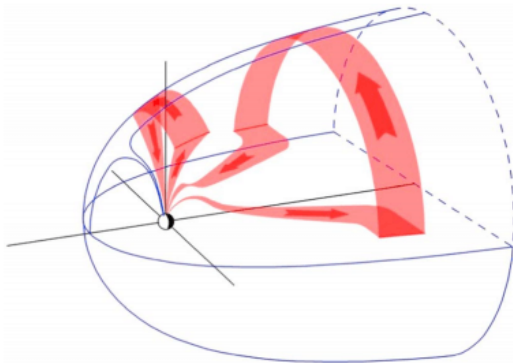
Figure 23.5: Region 1 field-aligned currents, shown as the red bands, including the two possible closure paths: directly to the magnetopause and via the far tail plasma sheet.
