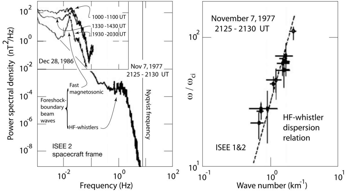
Figure 22.21: Left: The combined power spectral density of magnetic fluctuations excited by the ion foreshock boundary ion beam with central frequency around 1 Hz [lower part, data from Hoppe et al, 1982] and at <0.1 Hz [left upper part, data from Le & Russell, 1992] as measured by the ISEE spacecraft. This spectrum is obtained in the ISEE spacecraft frame. The low frequency spectrum is shown at three different times corresponding to (from below upward) increasing distance from inside the foreshock to the foreshock boundary. It is about five orders of magnitude more intense than the high-frequency waves. It is worth noting that the high frequency spectrum of Hoppe et al [1982] toward lower frequencies in the overlap with the Le & Russell [1992] spectrum does not show any indication of the lower frequency peak. As indicated by the thin straight line, it would smoothly continue into the 1930 UT branch at 0.01 Hz. This lack of the low frequency peak is probably accidental and due to the particular conditions at the time of measurement. Right: The wave dispersion relation for the high frequency 1 Hz whistler-mode waves determined from a tentative estimate of the relevant wave numbers and transformed into the plasma rest frame. It is seen that these waves in the observation range have about linear dispersion and frequencies \omega \sim (20 - 100)\omega_{ci} , far above the ion-cyclotron frequency \omega_{ci} [data from Hoppe et al, 1982]
