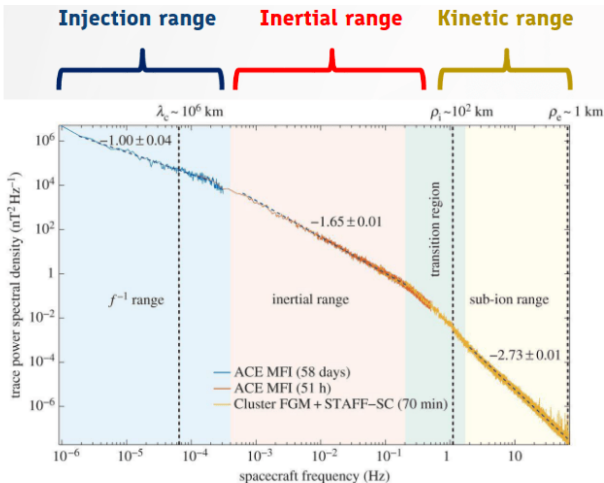
Figure 19.4: Solar wind power spectrum from Kiyoni+, 2015.
