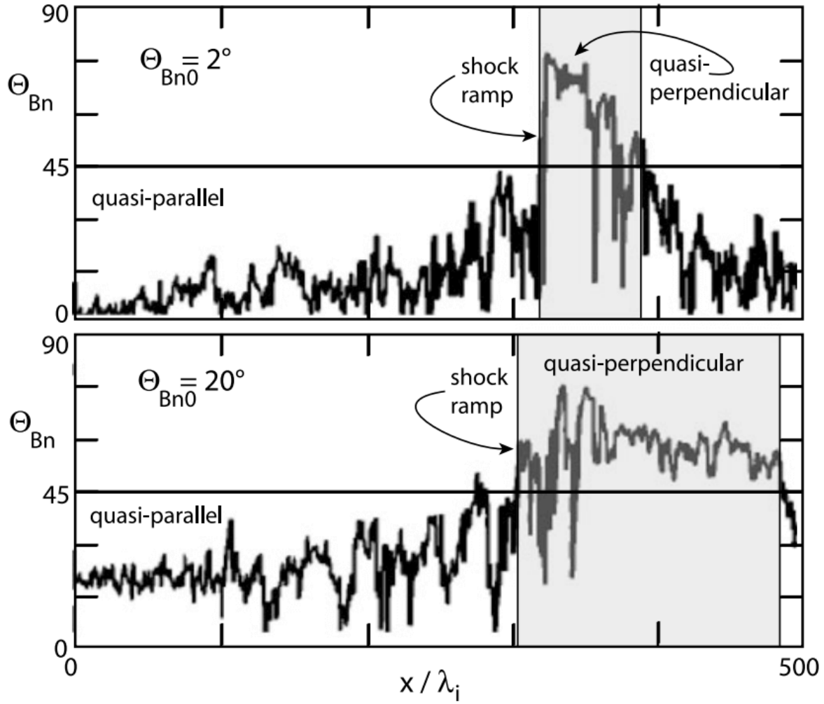
Figure 22.30: The evolution of the shock normal angle \theta_{Bn} on distance from the shock in two-dimensional hybrid simulations for two initial quasi-parallel shock-normal angles \theta_{Bn0} = 2^\circ and \theta_{Bn0} = 20^\circ , respectively [Scholer & Fujimoto, 1993]. The horizontal line at 45^\circ is the division between quasi-perpendicular and quasi-parallel shock normal angles. In both cases \theta_{bn} evolves from quasi-parallel direction into quasi-perpendicular direction. The shaded areas identify the quasi-perpendicular domains.
