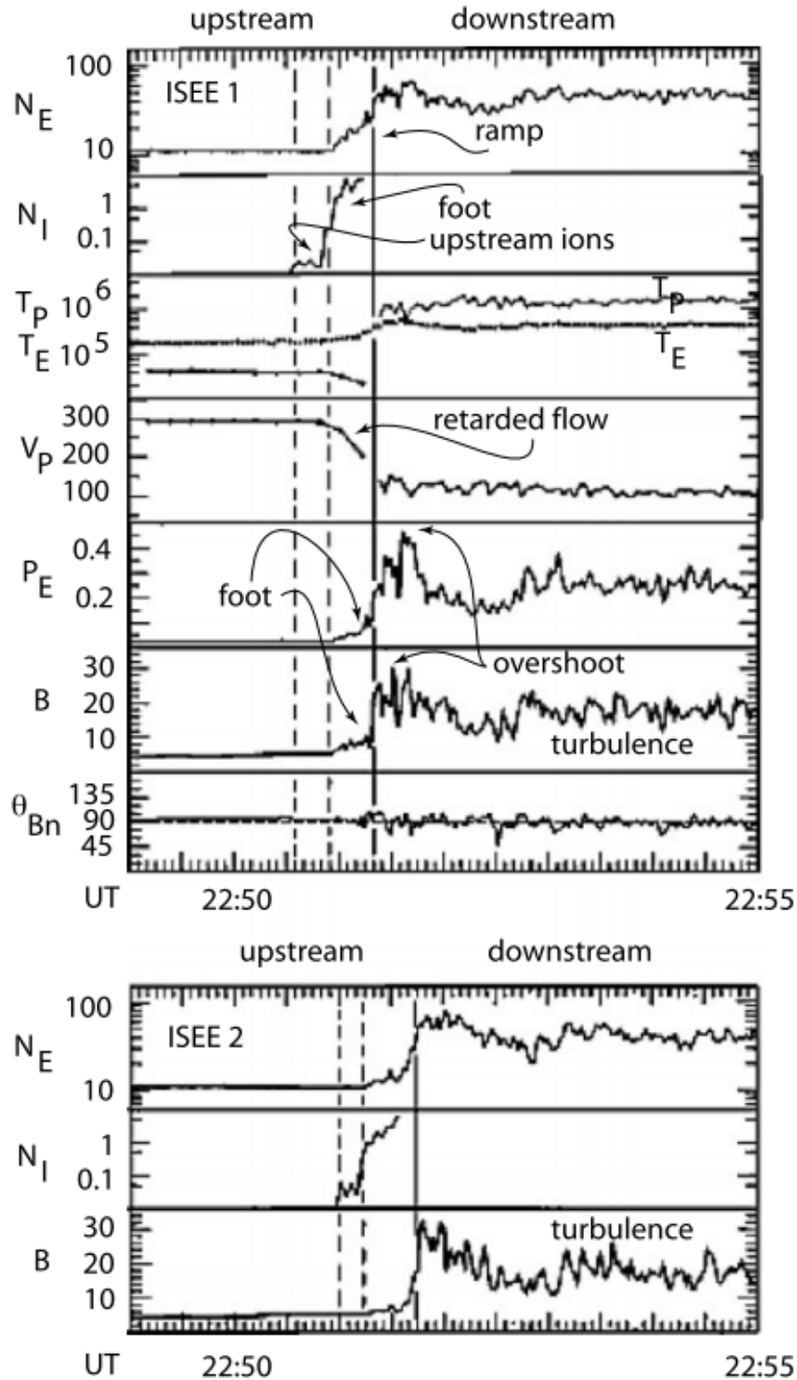
Figure 22.6: Time profiles of plasma and magnetic field parameters across a real quasi-perpendicular shock that had been crossed by the ISEE 1 and 2 spacecraft on November 7, 1977 in near-Earth space (Sckopke et al. 1983). N_E is the electron density, N_i the reflected energetic ion density, both in \text{cm}^{-3} , T_P , T_E are proton and electron in K. V_P is the proton (plasma) bulk velocity in \text{km s}^{-1} , P_e electron pressure in 10^{-9} \text{ N m}^{-2} , B the magnitude of the magnetic field in nT, and \theta_{Bn} . The vertical lines mark the first appearance of reflected ion, the outer edge of the foot in the magnetic profile, and the ramp in the field magnitude, respectively. The abscissa is the Universal Time UT referring to the measurements. The upper block are observations from ISEE 1, the lower block observations from ISEE 2.
