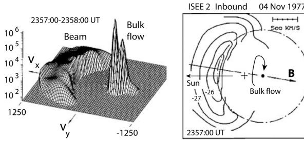
Figure 22.17: Left: A one-minute average pseudo-3D ion velocity-space profile in the (v_x, v_y) -plane showing the spreading of the beam in angle around the bulk flow without merging into the bulk flow. Right: Contour plot of the partial ring distribution.
