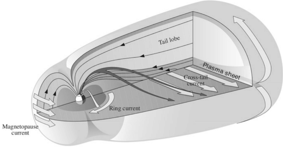
Figure 23.1: The magnetosphere and the large scale magnetospheric current systems.
