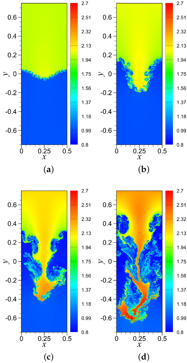
Figure 13.6: Simultaion of Rayleigh-Taylor instability (Rahman and San 2019).
