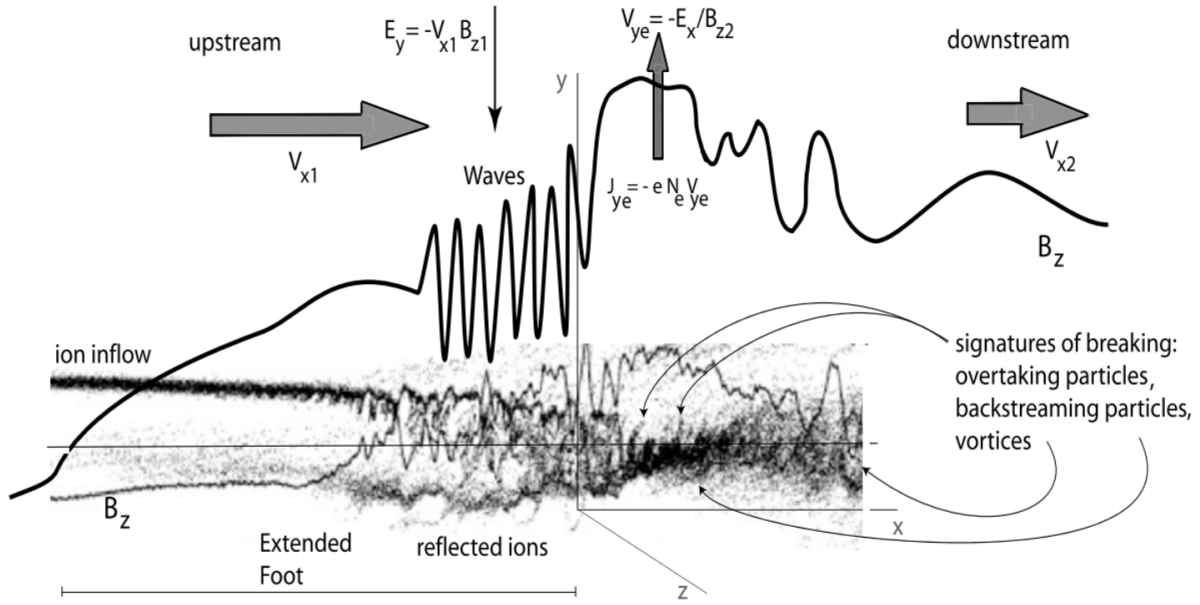
Figure 22.11: Schematic of the profile of a highly supercritical shock with waves just before shock reformation and signatures of beginning wave breaking (Balogh and Treumann 2013). It shows the structure of the ions in the ramp with the signatures of overtaking ions and backstreaming ions as well as ion vortices, all an indication of onset of breaking.
