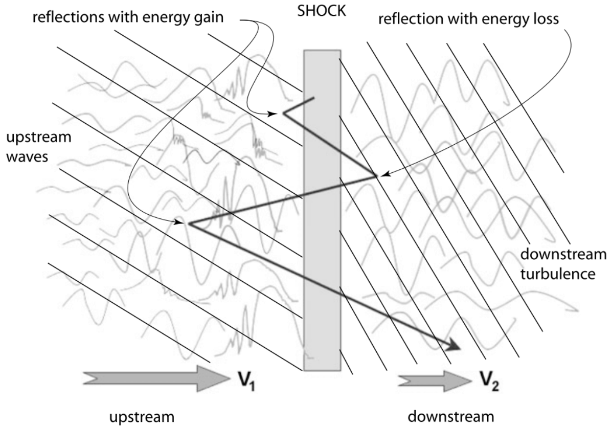
Figure 22.39: Schematic of the acceleration mechanism of a charged particle in reflection at a quasi-parallel ( \theta_{Bn} < 45^\circ ) supercritical shock. The upstream plasma flow (left, V_1 \gg V_2 ) contains the various upstream plasma modes: upstream waves, shocklets, whistlers, pulsations. The downstream (right) is turbulent. The energetic particle that is injected at the shock to upstream is reflected in an energy gaining collision with upstream waves, moves downstream where it is reflected in an energy losing collision back upstream. It loses energy because it overtakes the slow waves, but the energy loss is small. Returning to upstream it is scattered a second time again gaining energy. Its initially high energy is successively increased until it escapes from the shock and ends up in free space as an energetic Cosmic Ray particle. The energy gain is on the expense of the upstream flow which is gradually retarded in this interaction. However, the number of energetic particles is small and the energy gain per collision is also small. So the retardation of the upstream flow is much less than the retardation it experiences in the interaction with the shock-reflected low energy particles and the excitation of upstream turbulence.
