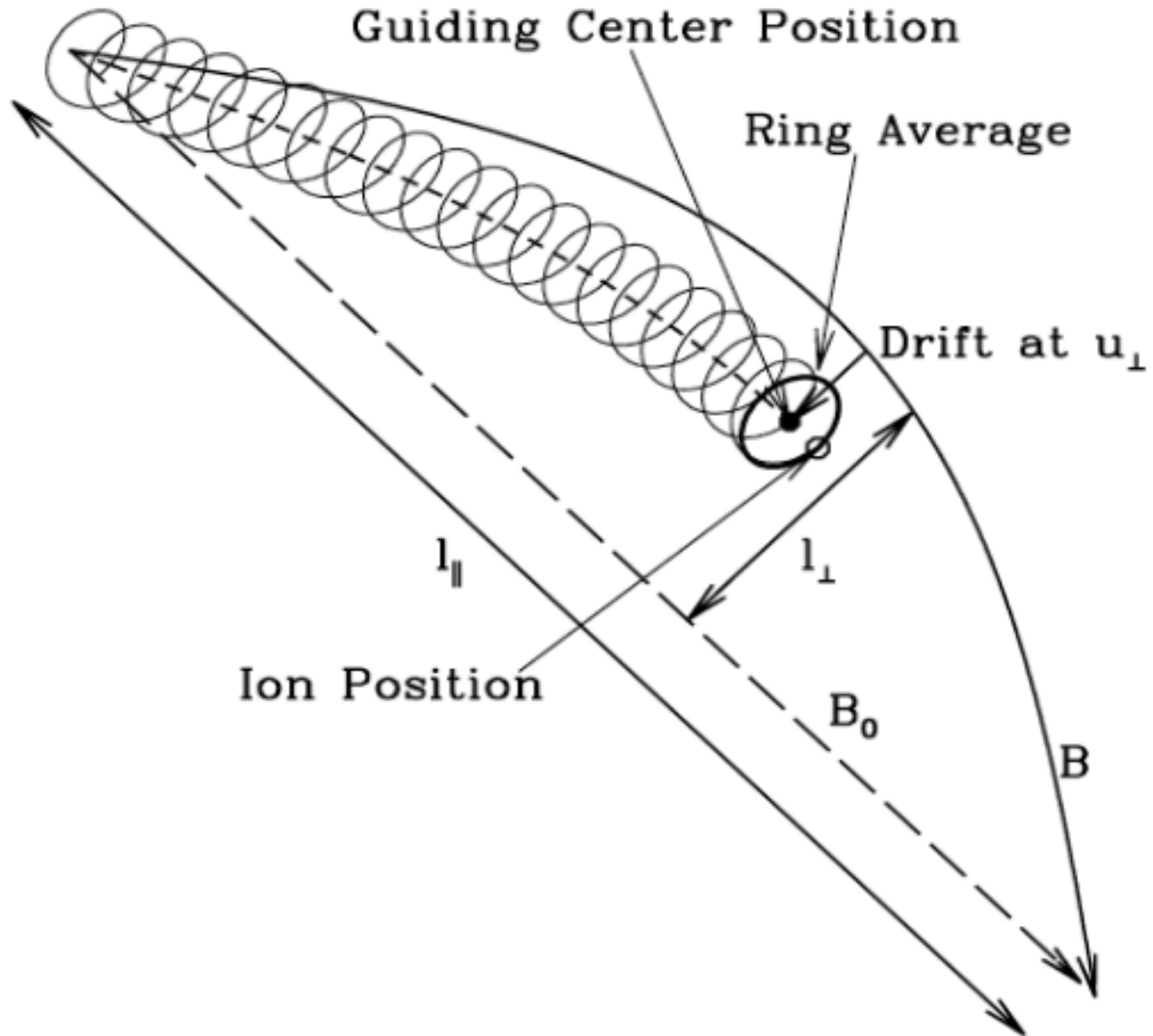
Figure 16.2: Gyrokinetic approximation.
