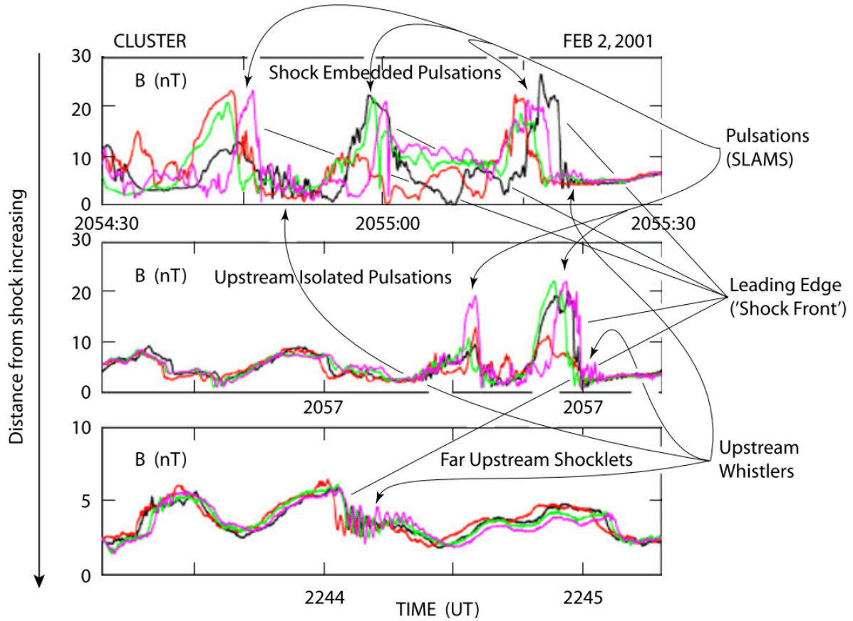
Figure 22.33: CLUSTER magnetic field measurements of magnetic pulsations (SLAMS) near and remote from a quasi-parallel shock on February 2, 2001 (Lucek et al. 2002). Only the magnetic field magnitude is shown for all four CLUSTER (colour coded) spacecraft. The spacecraft separation was between a few 100 km and 1000 km. Top: Clustered pulsations in the shock transition. Three events of large amplitudes are shown. These structures are very irregular with steep fronts. Note that in spite of the small spacecraft separation the shapes of the structures differ strongly from spacecraft to spacecraft. Moreover, determination of the pulsation fronts and normals (not shown) indicates high variability over the spacecraft separation distance. Thus the structures are of relatively small scale and large amplitude. Middle: Isolated pulsation at greater distance from shock outside compression region. The structures are seen almost simultaneously at the spacecraft and thus must be of larger size. Compared to the embedded pulsations the amplitudes are lower, and the structures are more regular. Bottom: A shocklet observed outside the pulsation region in the domain of ULF waves. The steep shock-like front is well expressed with the attached whistler waves it carries with it. Note the much lower amplitude than the pulsations.
