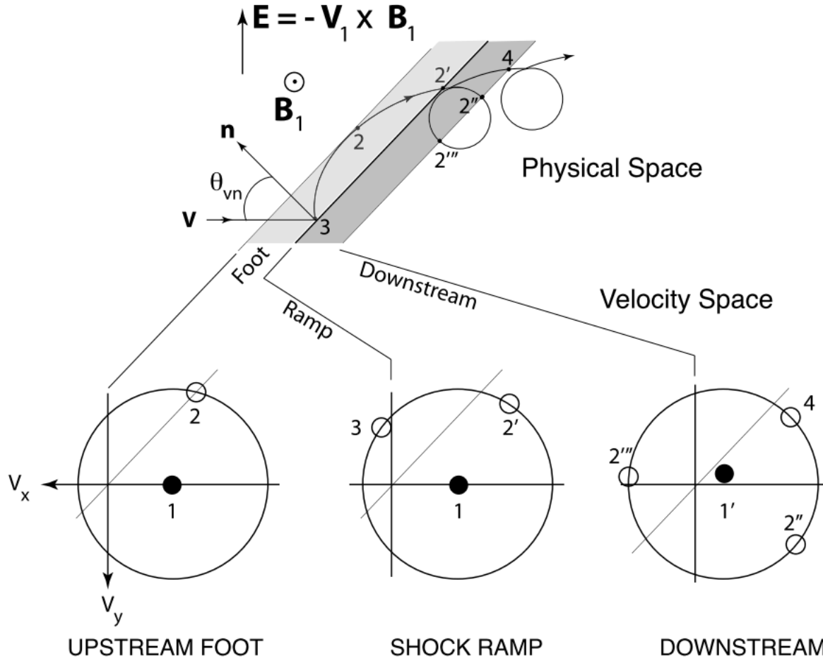
Figure 22.4: Top: Reflected ion orbits in the foot of a quasi-perpendicular shock in real space. The ion impacts under an instantaneous angle \theta_{vn} , is reflected from the infinitely thin shock, performs a further partial gyration in the upstream field \mathbf{B}_1 where it is exposed to the upstream convection electric field \mathbf{E} = -\mathbf{U}_1 \times \mathbf{B}_1 in which it is accelerated as is seen from the non-circular section of its orbit in the shock foot. It hits the shock ramp a second time now at energy high enough to overcome the shock potential, passing the ramp and arriving in the compressed downstream magnetic field behind the shock where it performs gyrations of reduced gyro-radius. Bottom: The ion distribution function mapped into velocity space v_x, v_y for the indicated regions in real space, upstream in the foot, at the ramp, and downstream of the shock ramp. Upstream the distribution consists of the incoming dense plasma flow (population 1, dark circle at v_y = 0 ) and the reflected distribution 2 at large negative v_y . At the ramp in addition to the incoming flow 1 and the accelerated distribution 2' there is the newly reflected distribution 3. Behind the ramp in the downstream region the inflow is decelerated 1' and slightly deflected toward non-zero v_y , and the energised passing ions exhibit gyration motions in different instantaneous phases, two of them (2'', 4) directed downstream, one of them (2''') directed upstream. (redrawn after Skopke et al. 1983).
