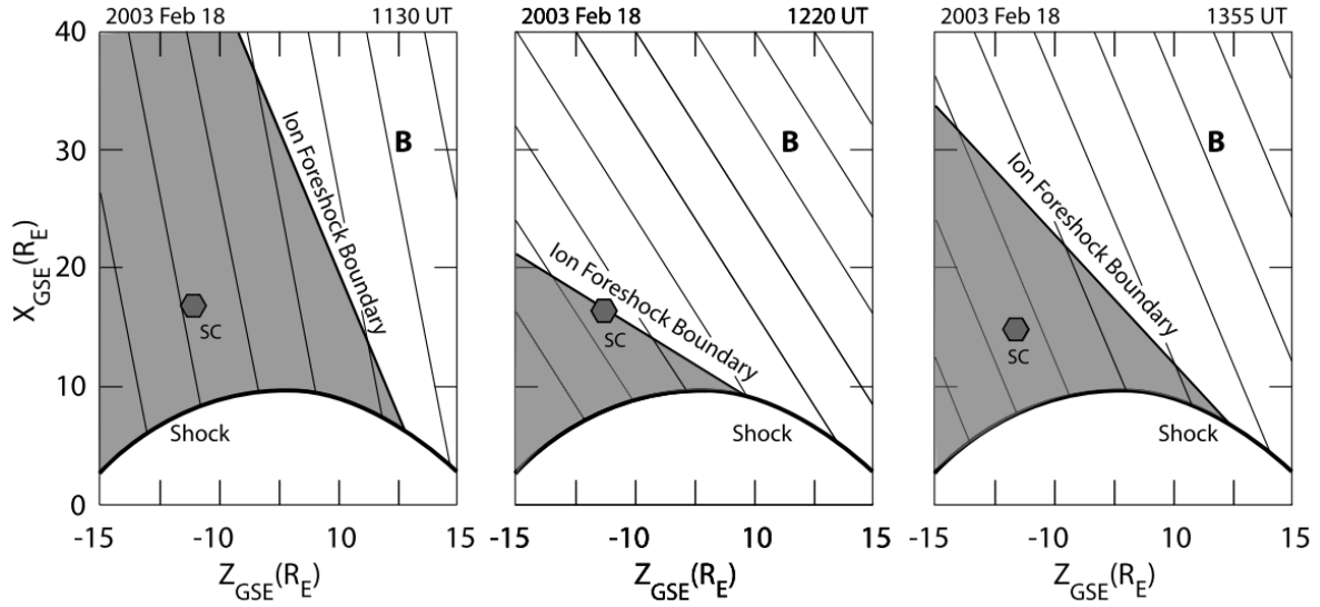
Figure 22.16: Reconstruction of the shape and location of the ion-foreshock boundary from the measured upstream plasma properties (direction of magnetic field, speed and density) for three successive times in order to explain the ion-phase space observations in Figure 22.15. The cold magnetic field-aligned ion beam is observed when the spacecraft is located in the vicinity of the ion-foreshock boundary at 1220 UT, while at 1130 UT and 1355 UT no beam was detected. It is assumed that the beam is generated along the foreshock boundary at the position where at the quasi-perpendicular shock surface the shock-normal angle is roughly about \theta_{Bn} \sim 60^\circ .
