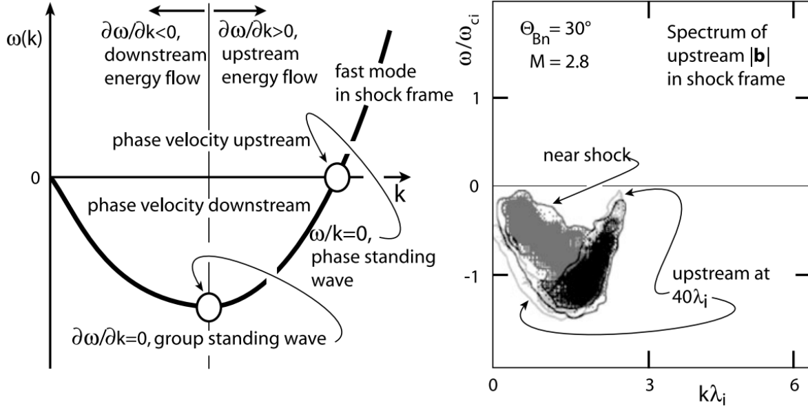
Figure 22.35: Fast mode dispersion relation in simulations in the shock frame. Left: The Doppler shifted fast mode dispersion relation in a supercritical flow in the shock frame. The Dispersion relation assumes negative frequencies corresponding to the downstream convection by the flow of Mach number M_A = 2.8 and at \theta_{Bn} = 30^\circ . Waves at zero group velocity have energy at rest in the shock frame. Negative group velocities imply downstream transport of energy, positive group velocities imply upstream transport. Right: Simulated upstream wave dispersion spectra near the shock and upstream of the shock. Near the shock wave energy accumulated around standing and downstream transport. Away from the shock the wave energy still moves upstream [data from Krauss-Varban & Omidi, 1991].
