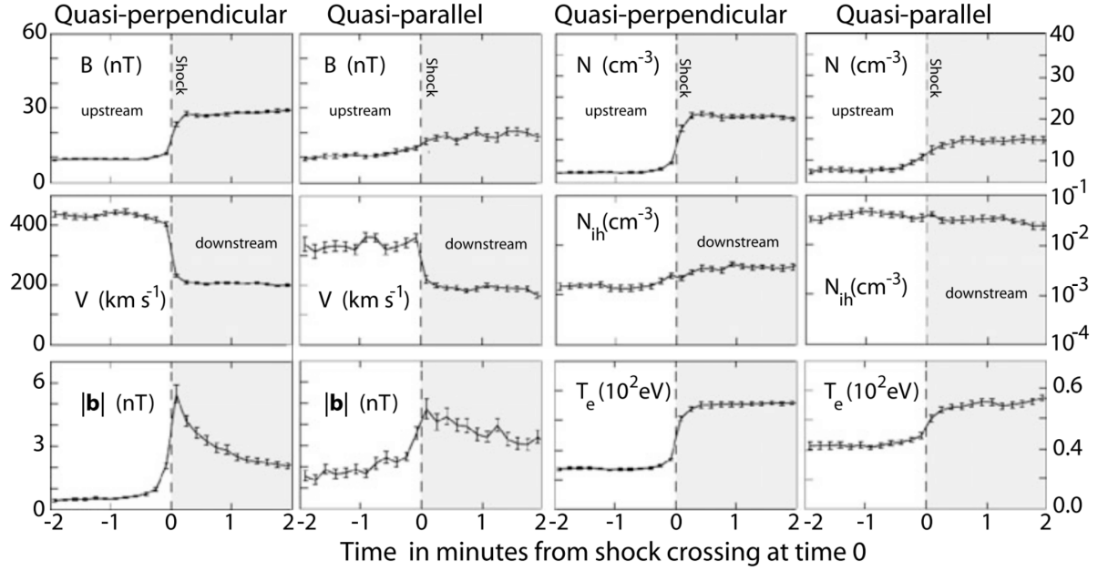
Figure 22.13: Comparison of average bulk plasma parameters in quasi-perpendicular and quasi-parallel shocks [data from Czaykowska et al, 2000]. The figure shows (on the left) the mean magnetic field B , bulk flow velocity V , average magnetic fluctuation amplitude at ultra-low frequencies, and (on the right) plasma density N , density of high energy ions N_{ih} , and electron temperature T_e . The shaded regions are the downstream parts of the AMPTE IRM crossings of the bow shock. The data have been obtained by normalizing the time with respect to crossing the nominal shock ramp by using the measured normal component of the bulk flow velocity, which is not so well-defined in the case of quasi-parallel shocks.
