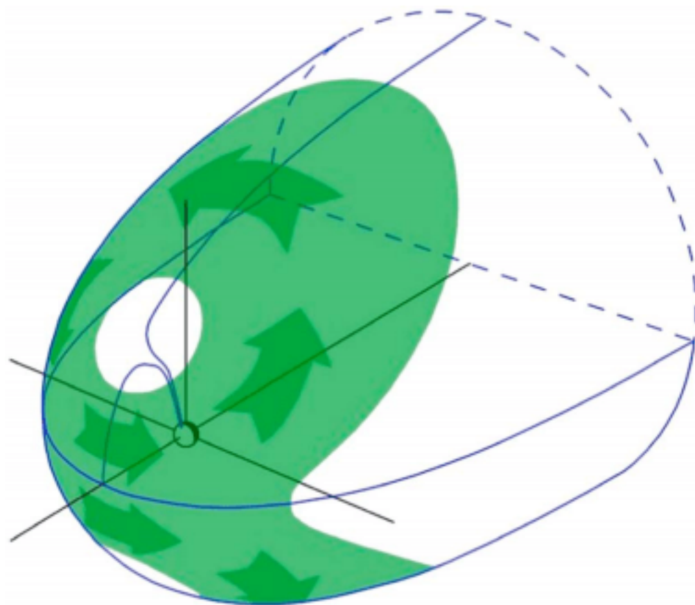
Figure 23.2: The Chapman-Ferraro dayside magnetopause currents are shown as a green-shaded surface on a simple wire diagram of the magnetopause. The Earth is the small sphere at the axis origin, and the Sun is to the lower left.
