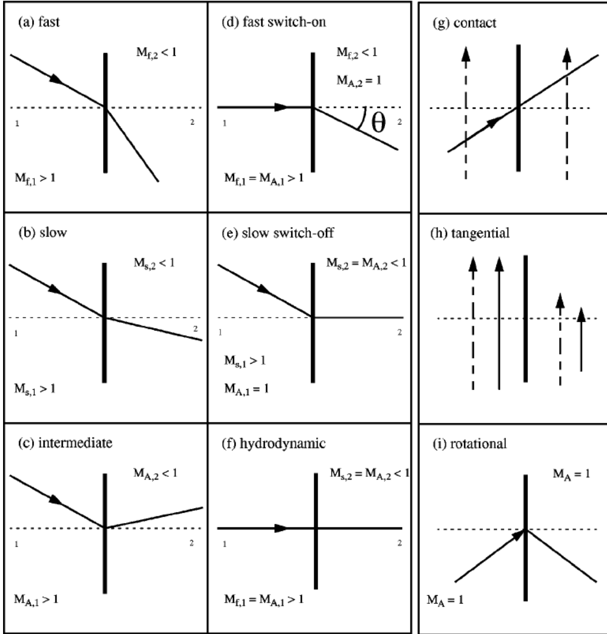
Figure 22.1: Some properties of MHD shocks and discontinuities. The thick vertical line is the shock surface. The shock normal is dotted. The full arrowed lines are magnetic field lines that are refracted through the shock surface. The dashed arrowed lines are velocity vectors. Region 1 is upstream, 2 is downstream. Reprinted from De Sterck et al. (1998).
