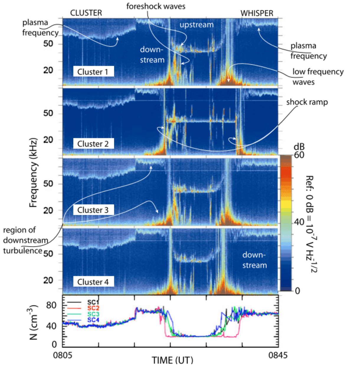
Figure 22.27: A CLUSTER spacecraft passage across the Earth's bow shock region on December 22, 2000. The spacecraft cross the downstream magnetosheath region (left) and the shock, enter the upstream solar wind region and back downstream. The figure shows broadband (0 kHz–80 kHz) plasma wave electric field spectra from all four CLUSTER spacecraft (Cluster 1–Cluster 4). The uppermost light blue emissions in each of the panels are at the electron plasma frequency f_{pe} which maps the local plasma density N estimates of which are shown in the lowest panel. Passages of the shock are signalled by intense broadband waves starting at low frequencies and being correlated with steep drops in N . In the low density upstream solar wind the spots of strong intensification of f_{pe} indicate contact with the electron foreshock boundary beam and excitation of Langmuir waves. These are highly structured, sometimes stretching above, sometimes hanging down below f_{pe} . Also seen are intermediate frequency emissions near the shock [data taken from Décréau et al, 2001].
