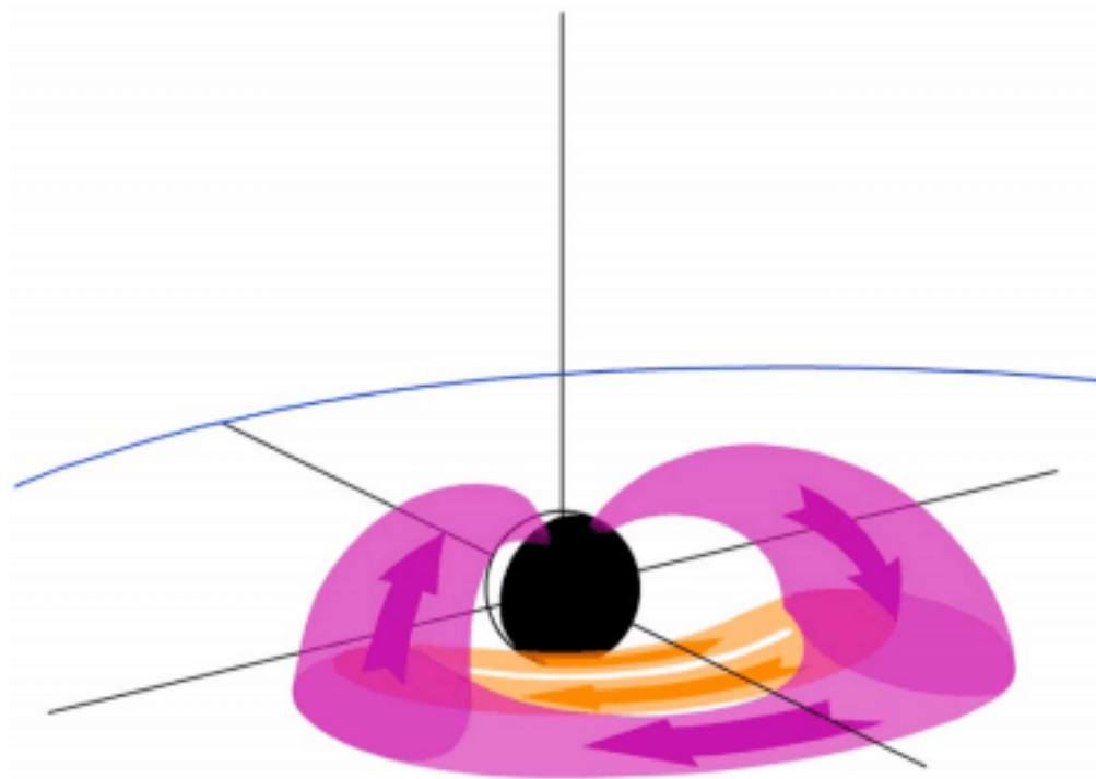
Figure 23.6: Region 2 field-aligned currents and partial ring current, shown in purple and the banana current, shown in orange. The view here is shifted to be from the evening sector.
