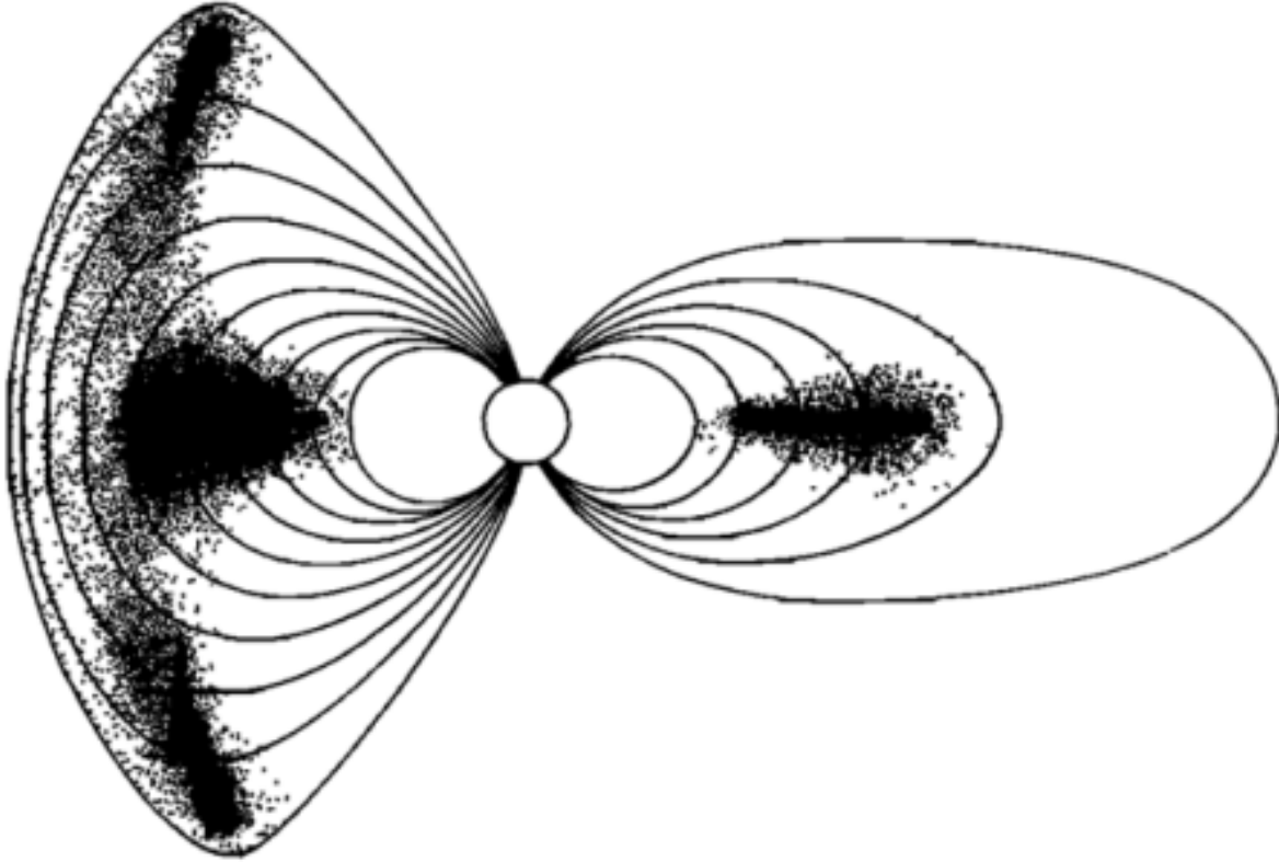
Figure 23.11: Schematic sketch of chorus/EMIC wave excitation regions, denoted by dots, on the noon-midnight meridian plane.
