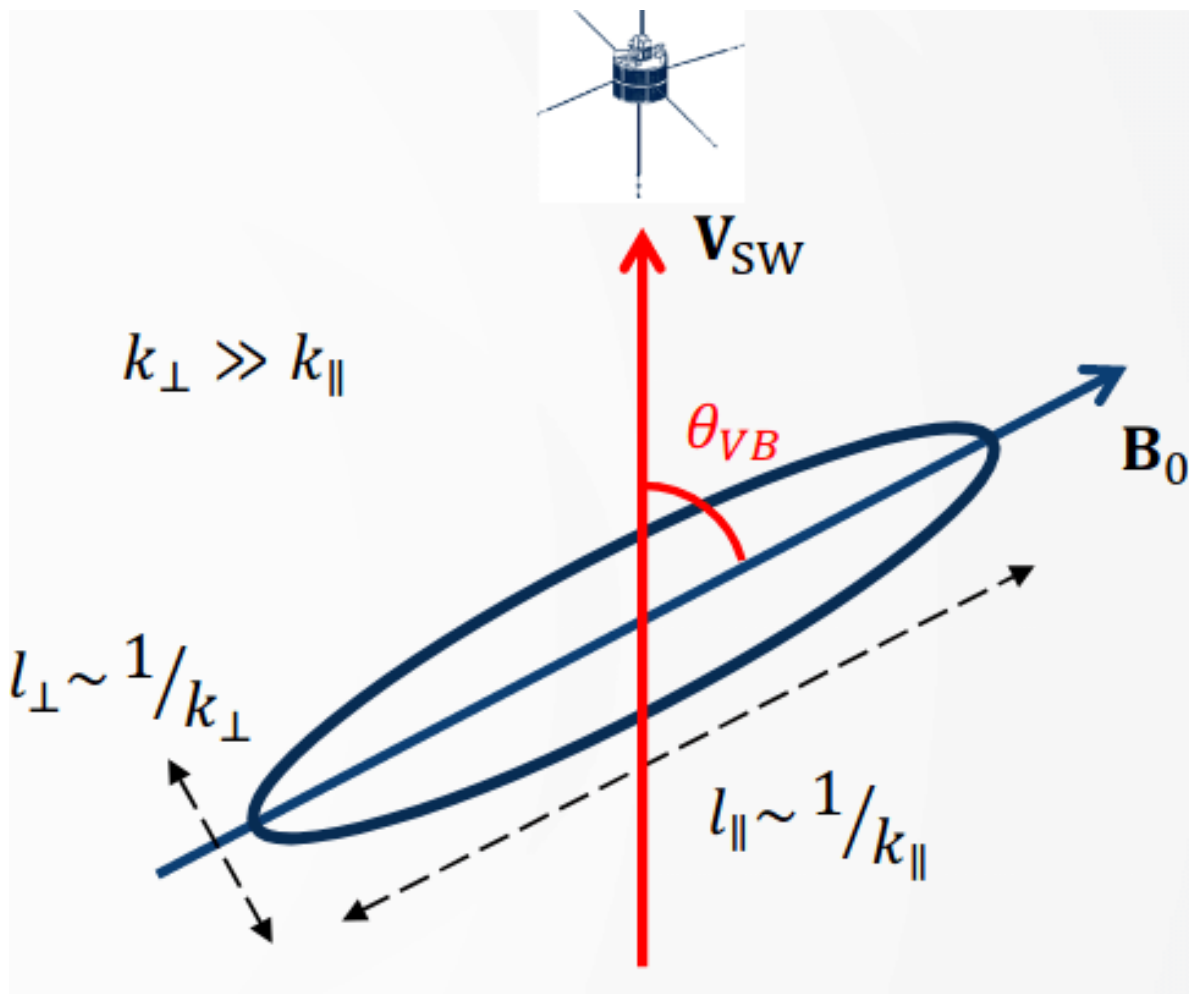
Figure 19.2: Wave scale from typical L1 satellite solar wind observation.
