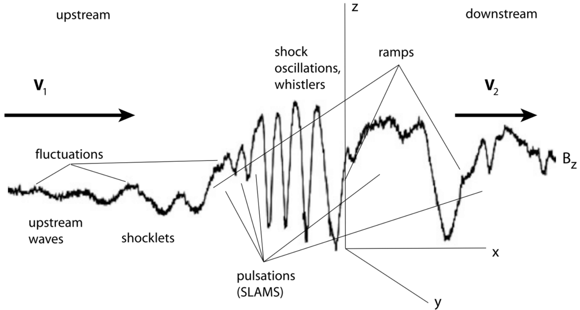
Figure 22.12: Schematic 1D profile taken along the nominal instantaneous shock normal of a supercritical quasi-parallel shock as seen in the magnetic field component B_z . This is the analogue to the quasi-perpendicular shock profile. It shows the main features in the vicinity of the quasi-parallel shock transition: the large amplitude upstream waves with the turbulent fluctuations on top of the waves, the formation of shocklets, i.e. steep flank formation on the waves exhibiting small-scale fluctuations on top of the wave, which act already like small shocks, very-large amplitude pulsations (magnetic pulsations or SLAMS) which turn out to be the building blocks of the shock, multiple shock-ramps at the leading edges of the pulsations belonging to diverse ramp-like steep transitions from upstream to downstream lacking a clear localization of the shock transition and any attached phase-locked whistlers. (Note that the entire figure is, in fact, the shock transition, as on this scale no clear decision can be made where the shock ramp is located.) Not shown here are the out of plane oscillations of the magnetic field that accompany the waves and the particle phase space.
