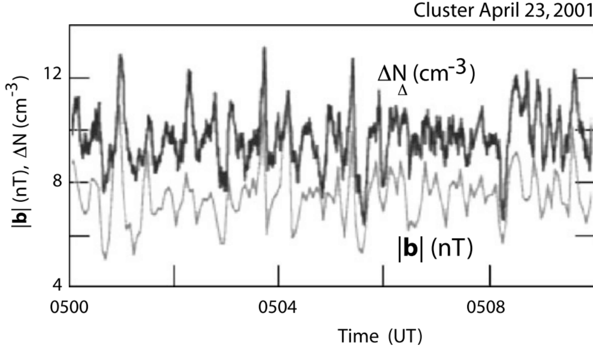
Figure 22.22: Left: The excellent correlation between the density and magnetic field variations in the ion-beam excited foreshock-boundary low-frequency waves as measured by CLUSTER [data from Eastwood et al, 2002]. The variations are practically in phase thus identifying the fluctuations as fast magnetosonic.
