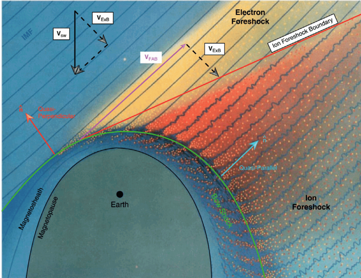
Figure 23.14: Foreshock configuration showing incident solar wind magnetic field (blue lines), impinging on the bow shock (green curved line), producing backstreaming ions (yellow dots), leaked magnetosheath ions (red dots), and upstream waves (wavy blue lines). The ion foreshock boundary is shown as the red line (Wilson III 2016). The foreshock boundary is the reflected ion trajectory tangent to the shock surface, taking into account the combination of a field-aligned motion and the solar wind convection electric field.
