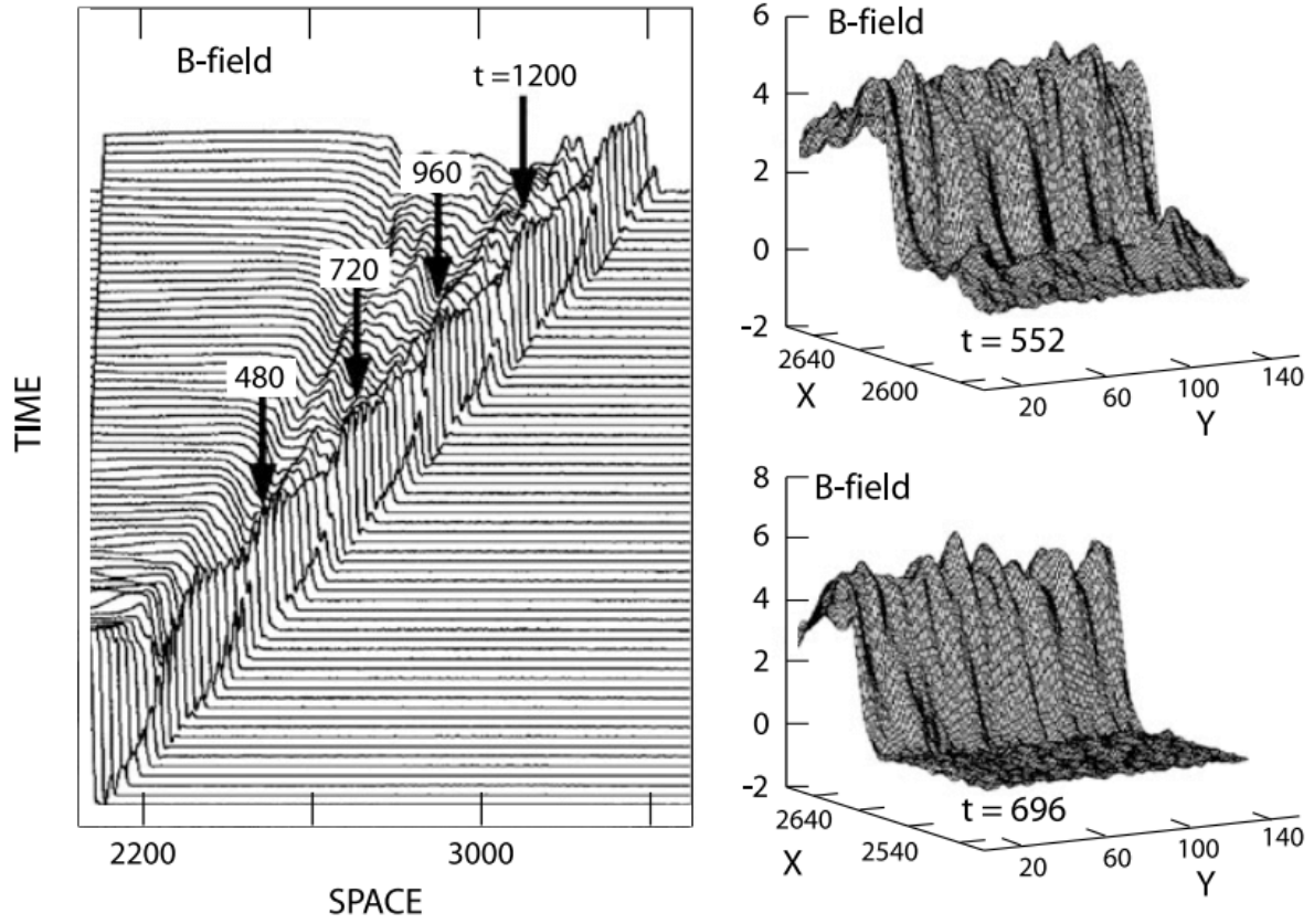
Figure 22.7: Magnetic field from full particle PIC simulations of shock reformation [Lembege & Savoini,2002]. Left: Reformation cycles of the magnetic field in the shock. Time is measured in inverse electron plasma frequencies \omega_{pe}^{-1} . The reformation times are indicated by the arrows in the plot with time given when the cycle is complete. Right: Two snapshots in time of the view of the shock front in the magnetic field at reformation. The interesting finding is that the front in this two-dimensional view is not a smooth plane but is quite distinctly structured in space and at the same time evolving.
