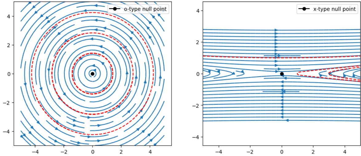
Figure 20.2: Example of (a) O-point and (b) X-point.
