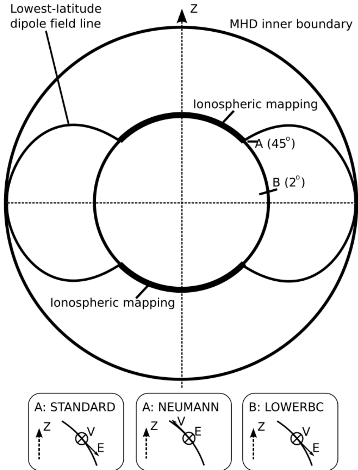
Figure 24.1: A schematic depiction of the inner boundary of the magnetosphere simulation and its ionospheric mapping. The location of the low-latitude boundary of the ionospheric grid is determined by the radius of the inner MHD boundary mapped along the dipole field from the equator. Point A (at 45^\circ ) denotes a typical location of the low-latitude boundary, where the STANDARD and NEUMANN boundary conditions are applied, while point B is where the LOWERBC boundary condition is applied. The three inset plots at the bottom depict schematically the configuration of velocity and electric field vectors with respect to the surface of the ionosphere in a meridional plane. The inset plot titles identify the type of the boundary condition and the point where it is applied. Adopted from (Merkin and
