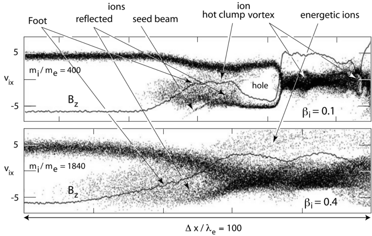
Figure 22.10: Ion phase space plot from 1D full PIC simulations Scholer et al. (2003) in the low- \beta regime with M_A = 4.2 .
