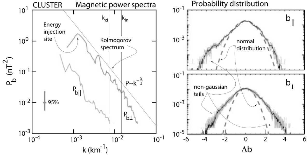
Figure 22.24: Left: Short wavelength spectra for the magnetic fluctuations measured by CLUSTER in the foreshock away from the foreshock boundary. These spectra are obtained by application of the “wave-telescope” analysis method. The perpendicular fluctuations are more than one magnitude more intense than the parallel fluctuations while the spectra decay about according to the Kolmogorov -5/3 -law of stationary inertial turbulence. Indication of a cut-off is seen at wave numbers larger than the inertial wave number k_{in} where strong dissipation sets on. From the maximum at k \sim 10^{-3} one concludes that in this wavelength range the spectral energy is injected by instability of fast and Alfvénic magnetosonic waves which cascade nonlinearly forward towards shorter wavelengths. Right: The probability distributions of the parallel and perpendicular magnetic fluctuations. The dashed distributions are log-normal of same maximum. These distributions exhibit extended tails and thus indicate non-stationary and probably intermittent not fully developed magnetic turbulence [after Narita et al, 2006].
