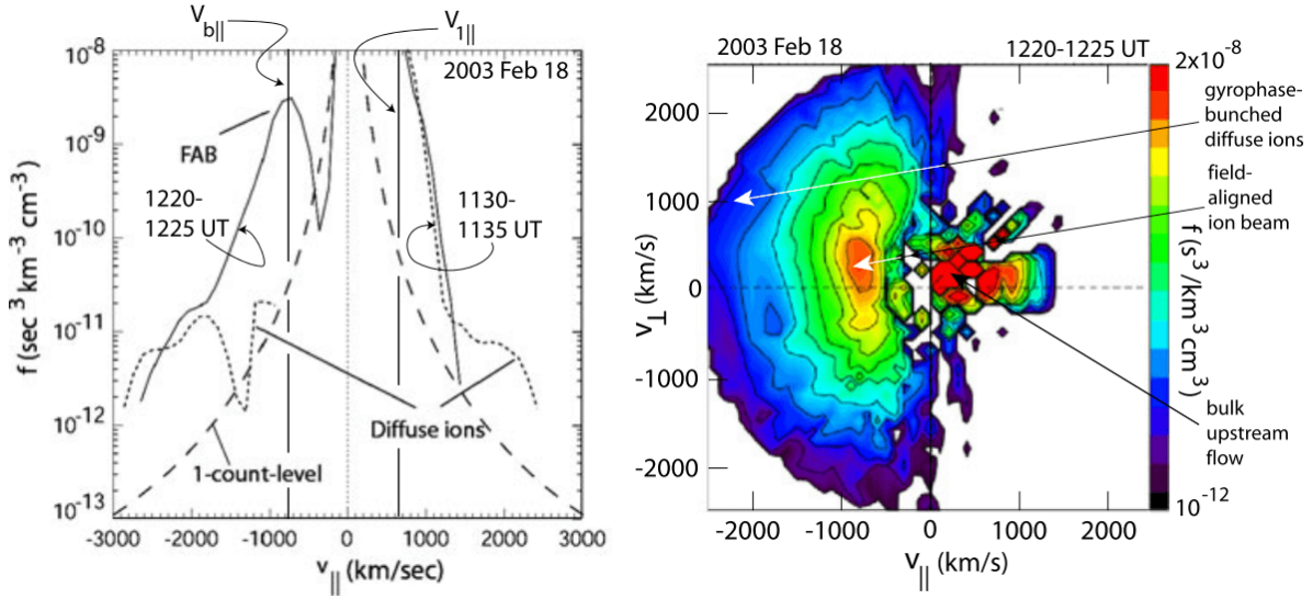
Figure 22.15: Left: The reduced field-aligned ion distribution functions in the foreshock region showing the field-aligned reflected ion beam (FAB) at 1220–1225 UT on February 18, 2003 which arrives at the spacecraft location along the magnetic field line that is connected to the quasi-perpendicular region of the Mach number M_A \sim 8 supercritical shock (smooth solid line). The upstream bulk velocity was V_1 \simeq 660 \text{ km s}^{-1} . Also shown is the reduced parallel distribution function (dashed) for the diffuse ion distribution observed at 1130–1135 UT the same day (for the geometry see Figure 6.7). It is clearly seen that the latter is about symmetric to the magnetic field direction indicating the symmetry of the ring of diffuse ions, while the foreshock-boundary field-aligned beam is flowing in the direction away from the shock into the upstream medium (negative velocities). Note also that the diffuse distribution appears as a smooth tail on the full ion distribution. The small gap on the left is uncertain as it dips into the 1-count level. Right: The two-dimensional phase space plot for the time interval 1220–1225 UT when the field-aligned beam was observed. Indicated are the bulk upstream flow, field-aligned ion beam, and the gyro-phase bunched residue of the diffuse upstream ions (data from Kis et al. 2004).
