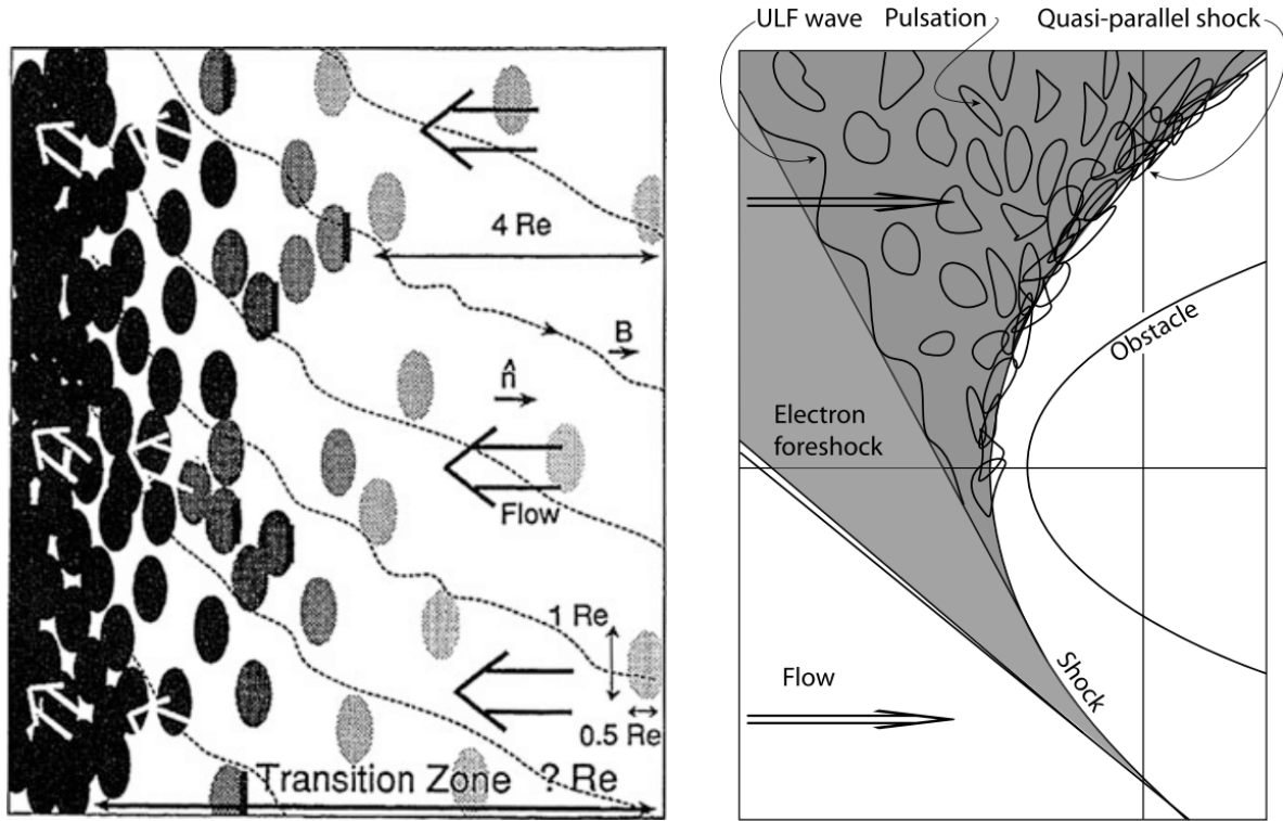
Figure 22.31: The patchwork model of Schwartz and Burgess (1991) of a quasi-parallel super-critical shock reformation. Left: Magnetic pulsations (SLAMS) grow in the ion foreshock and are convected toward the shock where they accumulate, thereby causing formation of an irregular shock structure. Note also the slight turning of the magnetic field into a direction that is more perpendicular to the shock surface with the shock surface itself becoming very irregular. Right: The same model with the pulsations being generated in the relatively broad ULF-wave-unstable region in greater proximity to the ion-foreshock boundary. When the ULF waves evolve to large amplitude and form localised structures these are convected toward the shock, grow, steepen, overlap, accumulate and lead to the build up of the irregular quasi-parallel shock structure which overlaps into the downstream direction.
