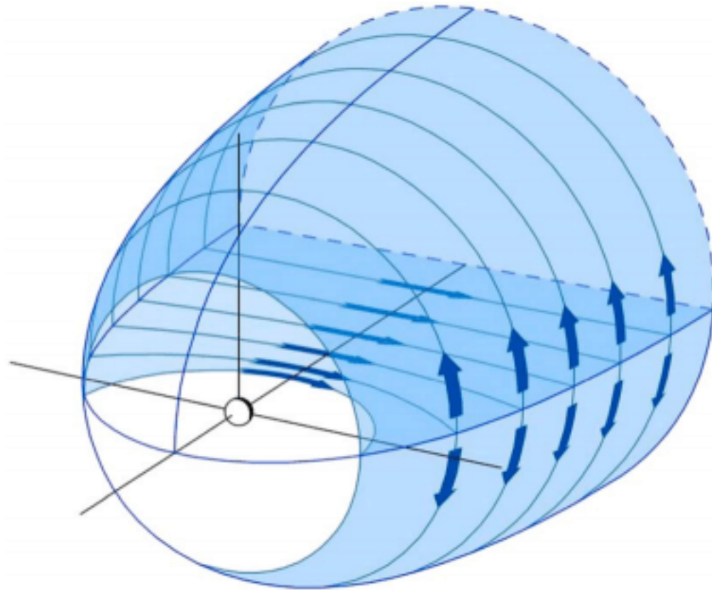
Figure 23.3: The tail current with closure via return current on magnetopause shown in light blue on the wire diagram of the magnetopause, as in Figure 23.2.
