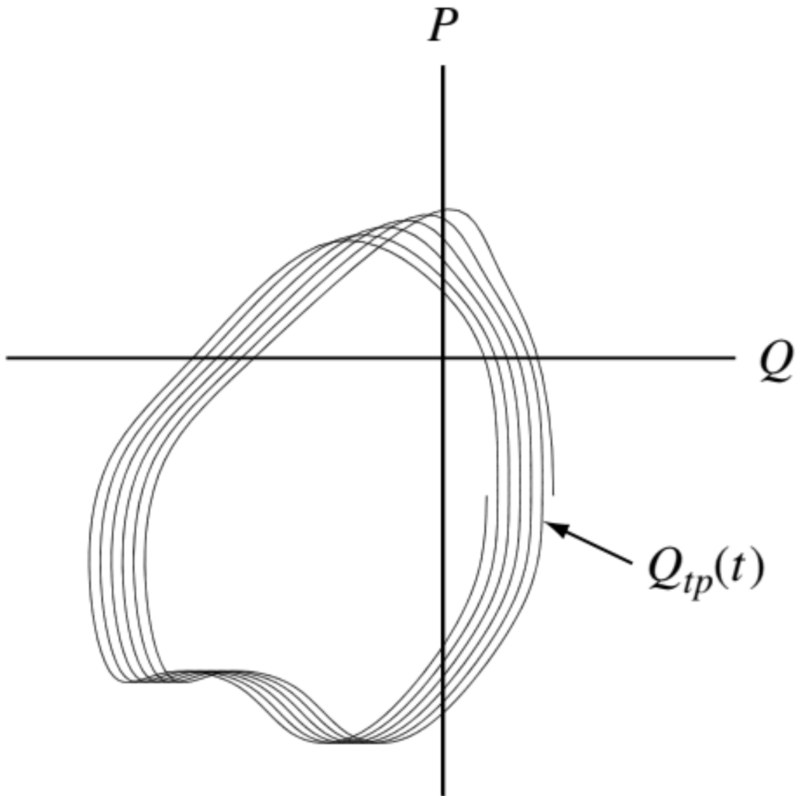
Figure 7.3: Nearly periodic-phase space trajectory for slowly changing Hamiltonian. The turning point Q_{tp}(t) is where Q is at its maximum.
