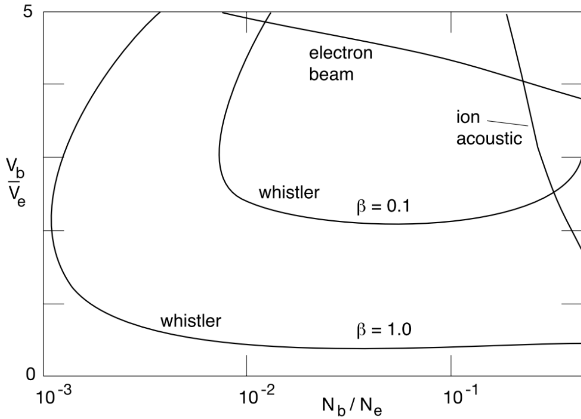
Figure 21.37: The regions of instability of the electron beam excited whistler mode in density and beam velocity space for two different \beta compared to the ion acoustic and electron beam modes. Instability is above the curves. The whistler instability has the lowest threshold in this parameter range (after Gary 1993).
