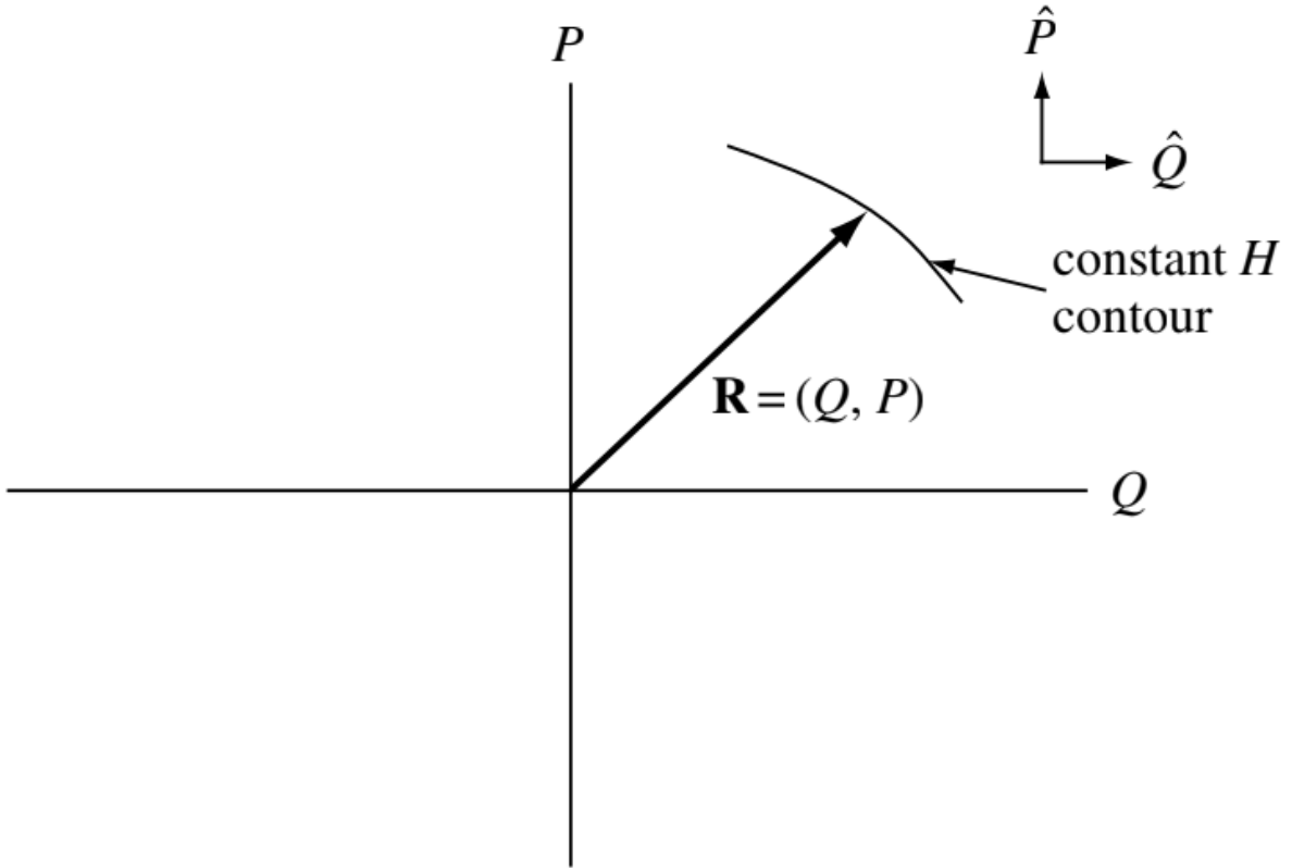
Figure 7.2: Canonical coordinate-momentum plane.
