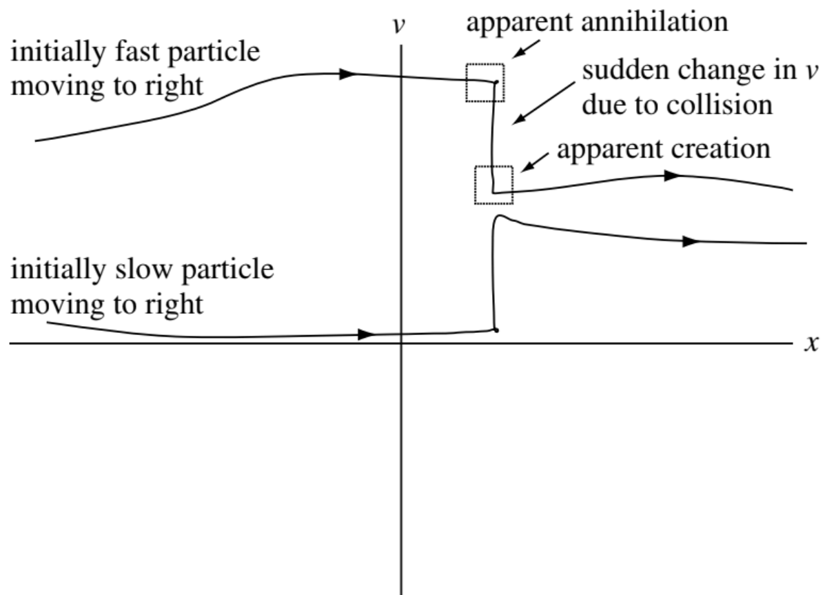
Figure 12.5: Detailed view of collisions causing “jumps” in phase-space.
