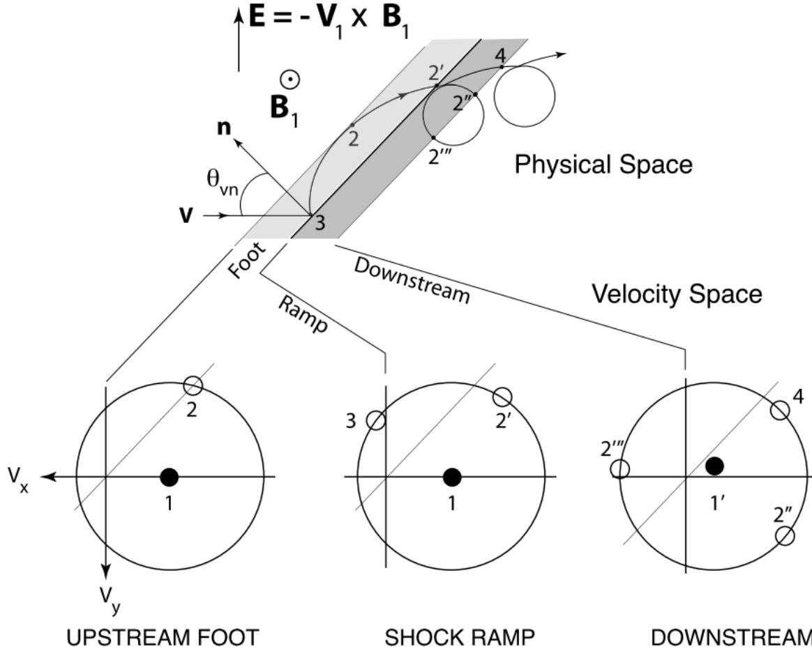
Figure 21.4: Top: Reflected ion orbits in the foot of a quasi-perpendicular shock in real space. The ion impacts under an instantaneous angle \theta_{vn} , is reflected from the infinitely thin shock, performs a further partial gyration in the upstream field \mathbf{B}_1 where it is exposed to the upstream convection electric field \mathbf{E} = -\mathbf{U}_1 \times \mathbf{B}_1 in which it is accelerated as is seen from the non-circular section of its orbit in the shock foot. It hits the shock ramp a second time now at energy high enough to overcome the shock potential, passing the ramp and arriving in the compressed downstream magnetic field behind the shock where it performs gyrations of reduced gyro-radius. Bottom: The ion distribution function mapped into velocity space v_x, v_y for the indicated regions in real space, upstream in the foot, at the ramp, and downstream of the shock ramp. Upstream the distribution consists of the incoming dense plasma flow (population 1, dark circle at v_y = 0 ) and the reflected distribution 2 at large negative v_y . At the ramp in addition to the incoming flow 1 and the accelerated distribution 2' there is the newly reflected distribution 3. Behind the ramp in the downstream region the inflow is decelerated 1' and slightly deflected toward non-zero v_y , and the energised passing ions exhibit gyration motions in different instantaneous phases, two of them (2'', 4) directed downstream, one of them (2''') directed upstream. (redrawn after Skopke et al. 1983).
