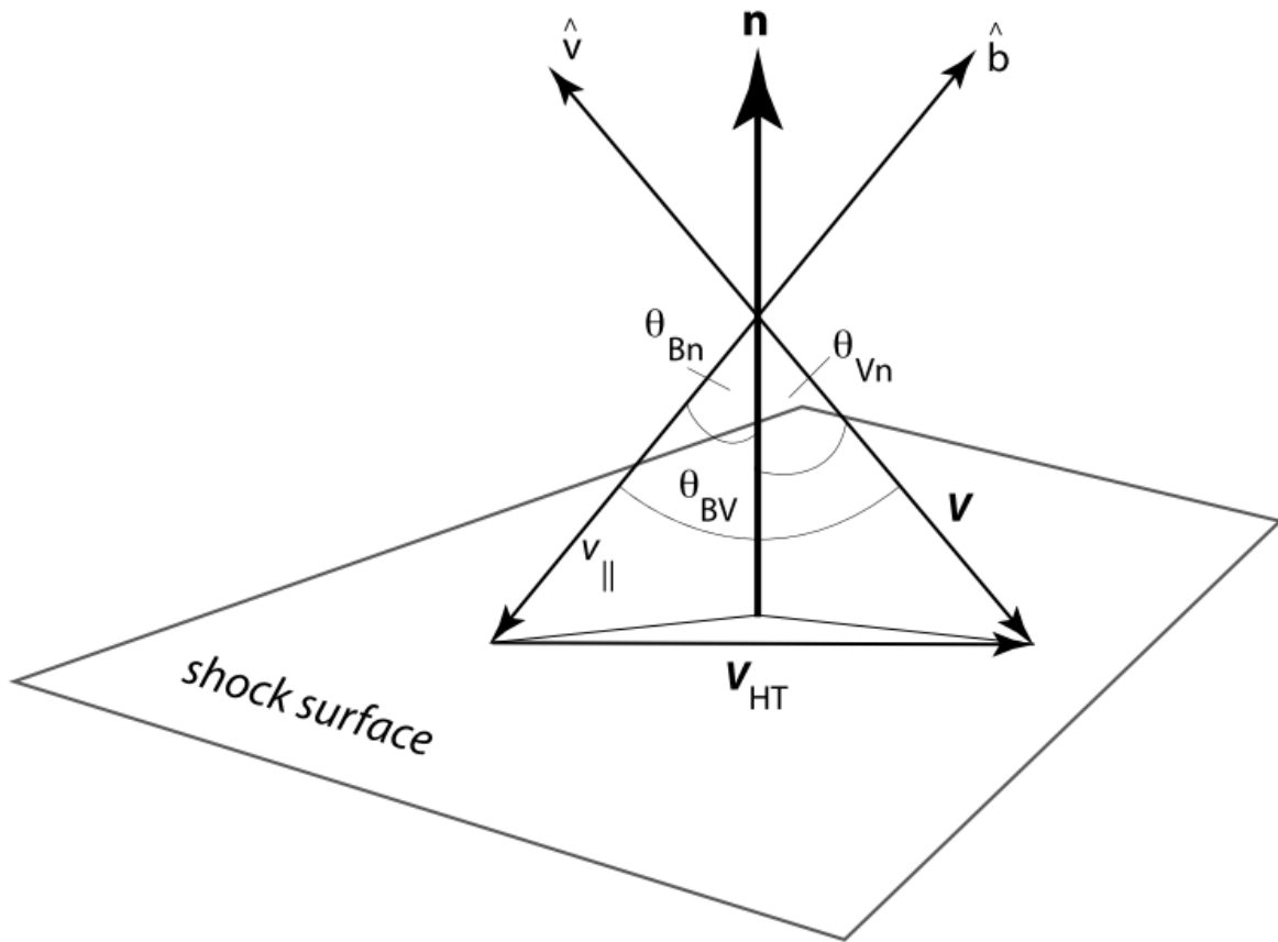
Figure 21.3: The shock coordinate system showing the shock normal \hat{n} , velocity and magnetic field directions \hat{v} , \hat{b} , the three angles \theta_{Bn} , \theta_{Vn} , \theta_{BV} between \hat{b} and \hat{n} , velocity \mathbf{U} and \hat{n} , and velocity \mathbf{U} and \hat{b} , respectively. The velocity \mathbf{V}_{HT} in the shock plane is the deHoffmann-Teller velocity (after Schwartz et al. 1983).
