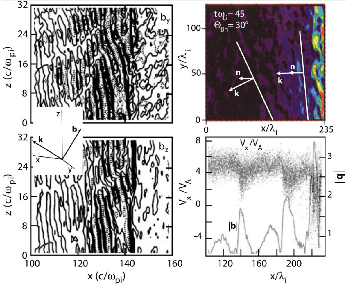
Figure 21.29: Two-dimensional hybrid simulations of the evolution of upstream waves. Left column: Upstream wave in a low-Mach number MA = 2.2 quasi-parallel shock [after Scholer & Fujimoto, 1993]. The nominal shock is in the (y, z) -plane. Ions escaping to upstream generate the oblique upstream magnetosonic waves. The contour plot of the two normalized to the upstream magnetic field components of the magnetic fluctuations shown is taken at relatively early times t\omega_{ci} = 68 . It shows the nearly plane magnetic wave fronts inclined against the shock in direction x and having wavelengths of \sim 10c/\omega_{pi} in z while being much shorter in x . In the vicinity of the shock the wave fronts turn more parallel to the shock and produce a non-coplanar magnetic component |b_y| which is of same order as the |b_z| . Moreover, even though the shock has relatively low Mach number, it is not completely stable but shows structure in z direction which is produced by the presence of the reflected upstream particles and the upstream waves. At places it is impossible to identify one single shock ramp. Right column: Two-dimensional hybrid simulations of the evolution of giant magnetic pulsations (SLAMS) in front of a quasi-parallel supercritical shock [after Dubouloz & Scholer]. Top: The simulation plane showing the structure of the (normalized) magnetic fluctuation field |b| at time t\omega_{ci} = 45 and shock normal angle \theta_{Bn} = 30^\circ . The accumulation of the growing wave fronts at the shock transition, their increasing amplitudes, and their turning towards becoming parallel to the shock is clearly visible from the rotation of the two wave fronts and their \mathbf{k} vectors shown in white. Away from the shock transition the angle between \mathbf{k} and the shock normal \hat{n} is large. Close to the shock the two vectors are about parallel. The magnetic field is in the wave front, so \theta_{Bn} is close to 90^\circ here. Bottom: Pulsation amplitude and ion phase space. The fluctuations evolve into large amplitude pulsations when approaching (and making over) the shock. The streamer velocity of the upstream
