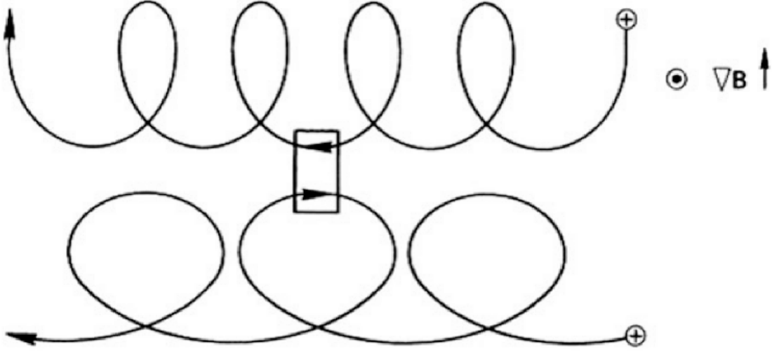
Figure 8.3: In a nonuniform B field the guiding centers drift but the fluid elements do not.
