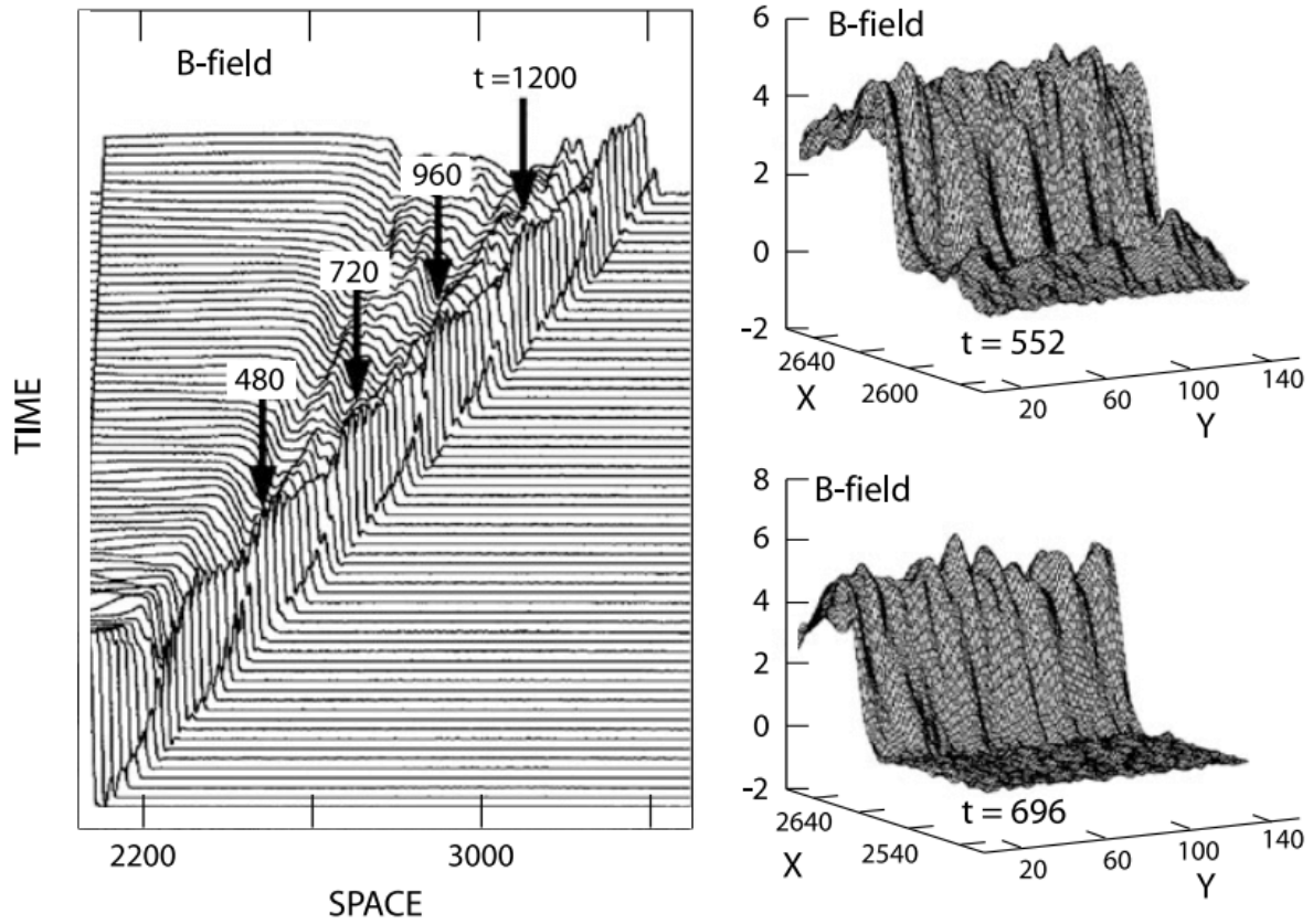
Figure 21.7: Magnetic field from full particle PIC simulations of shock reformation [Lembege & Savoini,2002]. Left: Reformation cycles of the magnetic field in the shock. Time is measured in inverse electron plasma frequencies \omega_{pe}^{-1} . The reformation times are indicated by the arrows in the plot with time given when the cycle is complete. Right: Two snapshots in time of the view of the shock front in the magnetic field at reformation. The interesting finding is that the front in this two-dimensional view is not a smooth plane but is quite distinctly structured in space and at the same time evolving.
