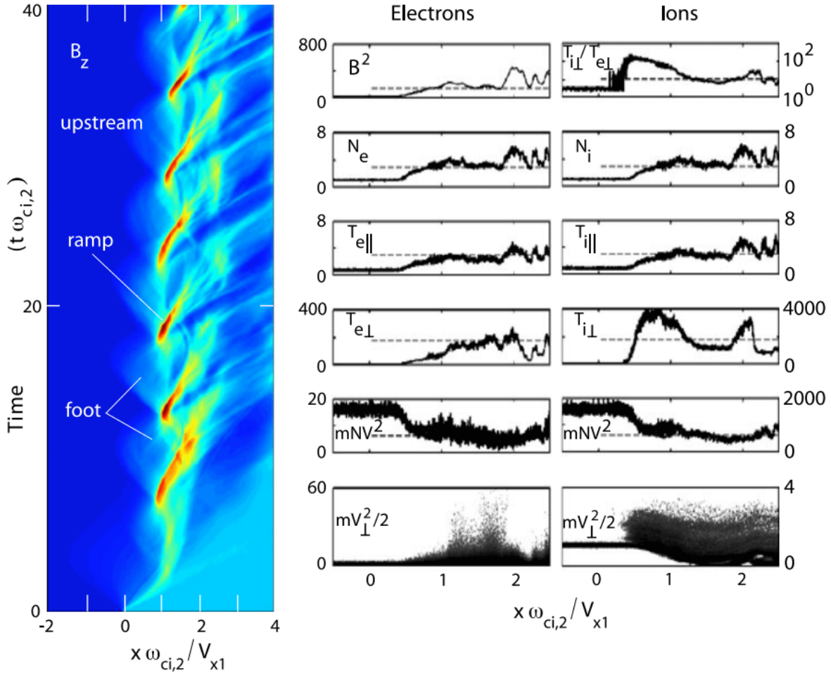
Figure 21.9: Left: Evolution of the magnetic field in a quasi-perpendicular high Mach number M_A = 10 PIC simulation (after Umeda and Yamazaki 2006). Here the presentation is in the shock frame of reference, and the shock has been initialised by assuming Rankine-Hugoniot initial jump conditions. The non-physical nature of this assumption is visible in the initial evolution and fast displacement of the shock to the right. After the initial unphysical disturbance has disappeared a self-consistent physical state is reached in which the shock quasi-periodically reforms itself. The competition between the shock foot and ramp formation is nicely seen in the colour plot of the magnetic field B_z . Right: Electron and ion plasma parameters in computational units. Of interest is only their relative behaviour, not the absolute values. The profiles are taken at time t\omega_{ci,2} = 38.1 (No 2\pi factor!). They show the compression of the plasma and heating of electrons and ions. Parallel electron and ion heating is comparable, but ions are heating much stronger than electrons in perpendicular direction causing a large perpendicular temperature anisotropy downstream of the shock.
