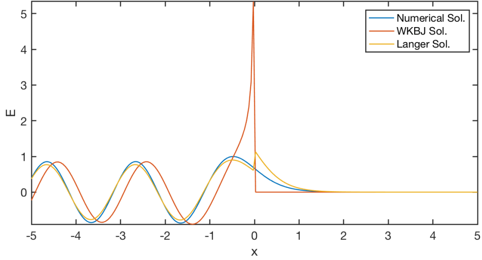
Figure 3.3: Comparison between the WKB solution, uniformly valid solution and numerical integral solution for the O-mode with monotonically increasing density with x .
