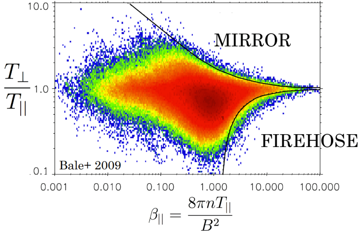
Figure 14.2: Collective solar wind observation data ( \sim 1e6 ) from Wind spacecraft. The lines represent the instability thresholds for mirror and firehose instability, respectively.
