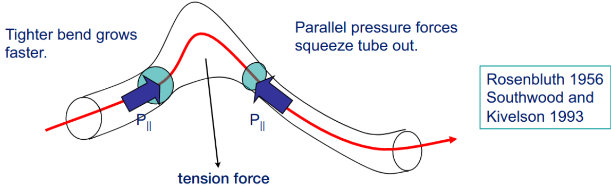
Figure 14.1: Along a flux tube, p_{\parallel} is the destabilizing force, the curvature force is the stabilizing force.
