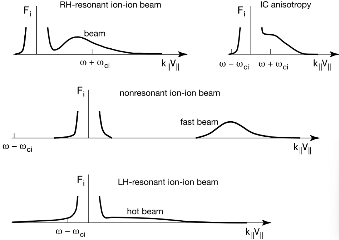
Figure 21.36: The three cases of ion beam-plasma interaction and the location of the unstable frequencies. Shown is the parallel (reduced) distribution function F_i(k_{\parallel} v_{\parallel}) , where for simplicity the (constant) parallel wavenumber k_{\parallel} has been included into the argument. Right handed resonant modes (RH) are excited by a cool not too fast beam. When the beam is too fast the interaction becomes nonresonant. When the beam is hot, a resonant left hand mode (LH) is excited. In addition the effect of temperature anisotropy is shown when a plateau forms on the distribution function (after Gary 1993).
