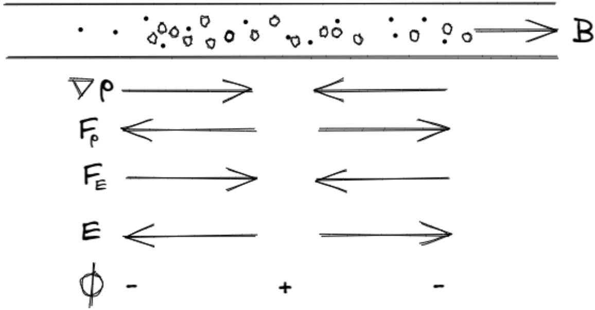
Figure 8.4: Physical reason for the Boltzmann relation between density and potential.
