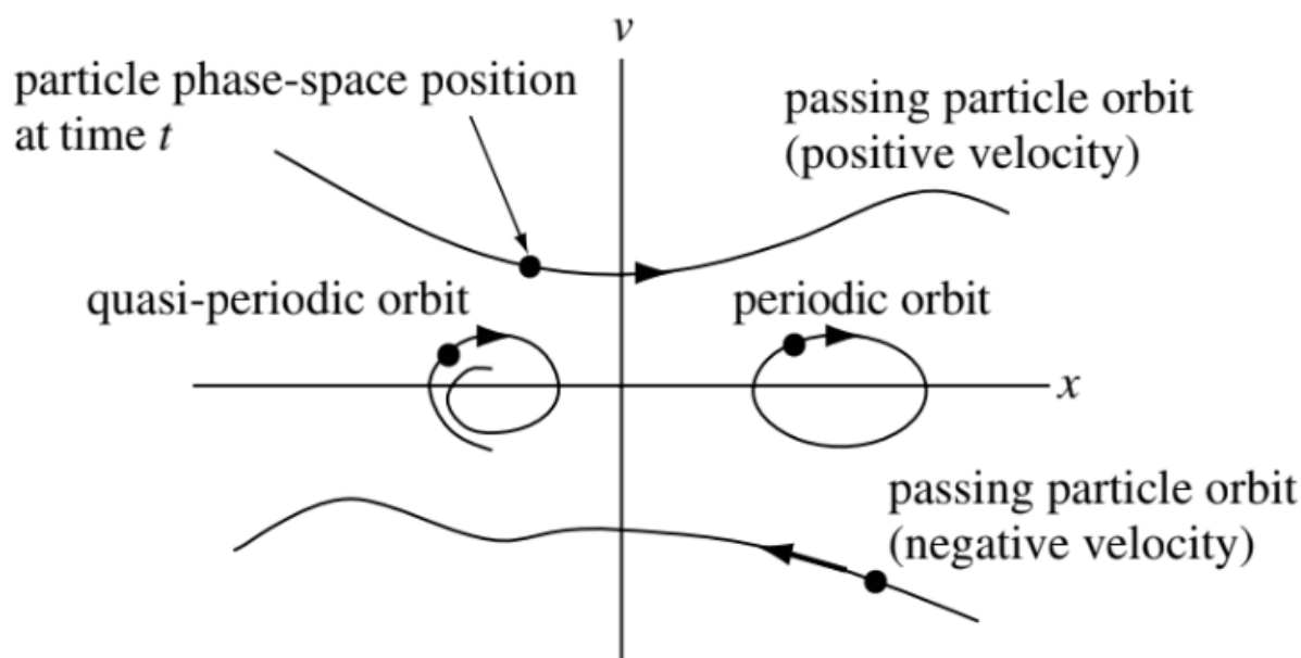
Figure 12.1: Phase-space showing different types of possible particle orbits.
