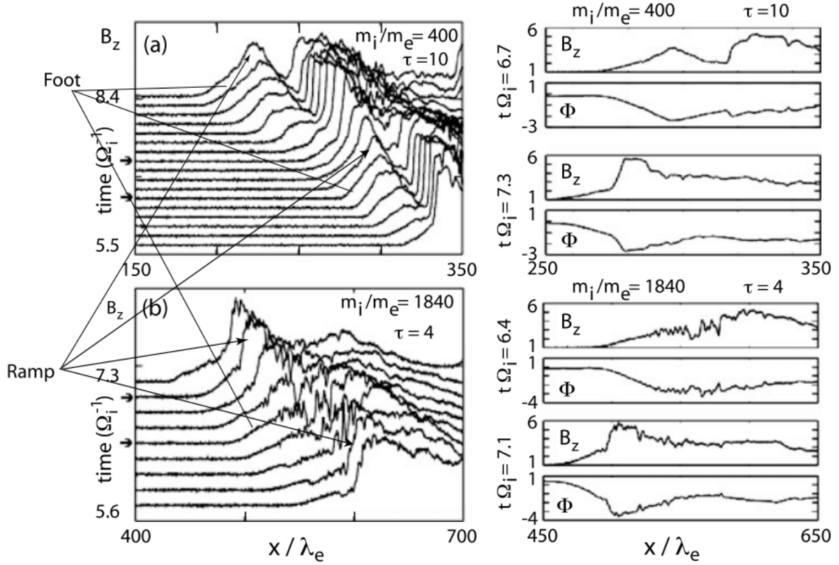
Figure 21.8: Left: One-dimensional PIC simulations (after Scholer et al. 2003) of quasi-perpendicular \theta_{Bn} = 87^\circ shock reformation for mass ratios m_i/m_e = 400 and 1840 . Time is in \Omega_i^{-1} = \omega_{ci}^{-1} , space in d_e . The parameter \tau = \omega_{pe}^2/\omega_{ce}^2 is taken small in both cases. The higher mass ratio shows a violent time evolution because of the high electron mobility. Reformation of the shock is due to evolution of the shock feet. The original foot region builds up until becoming itself the shock assuming the role of the ramp. Afterwards a secondary foot evolves in front of this new ramp. Right: Spatial shock profiles at two time sections (see arrows on the left). The higher mass ratio run shows a more subtle structure in B_z and shock potential \phi , but the gross features are similar. The potential drop exists already in the foot but the main drop occurs in the ramp. The lower mass ratio has a more concentrated foot region.
