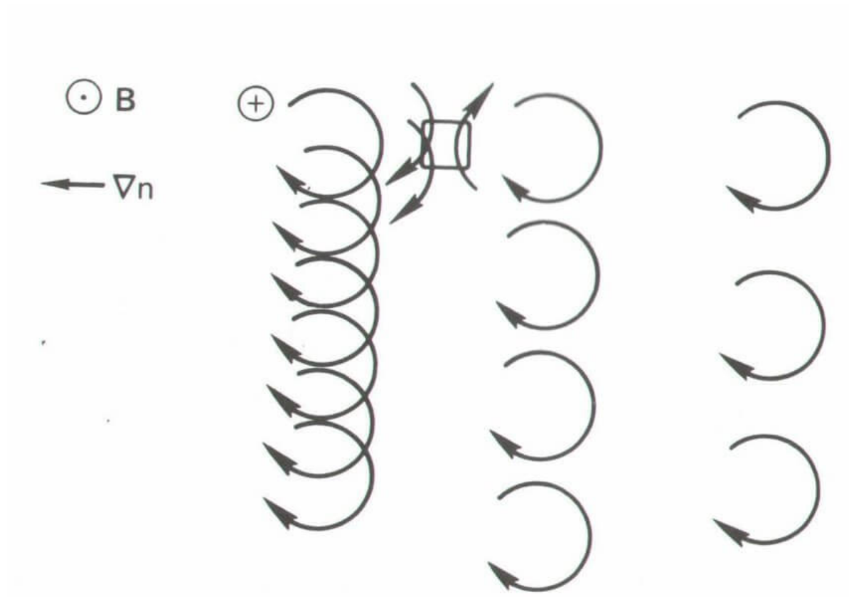
Figure 8.2: Origin of the diamagnetic drift.
