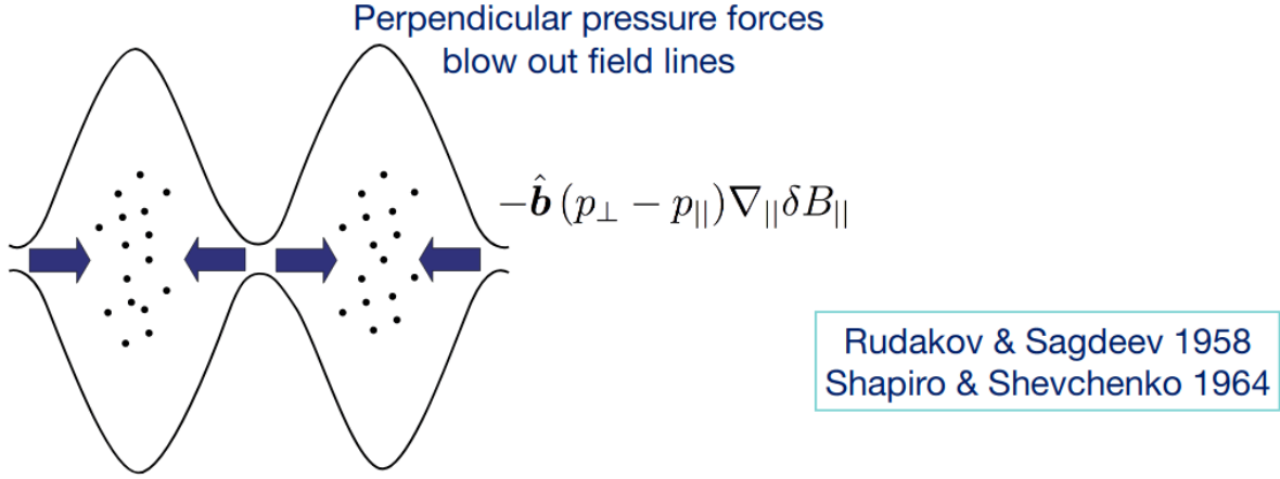
Figure 13.8: Illustration of mirror instability.
