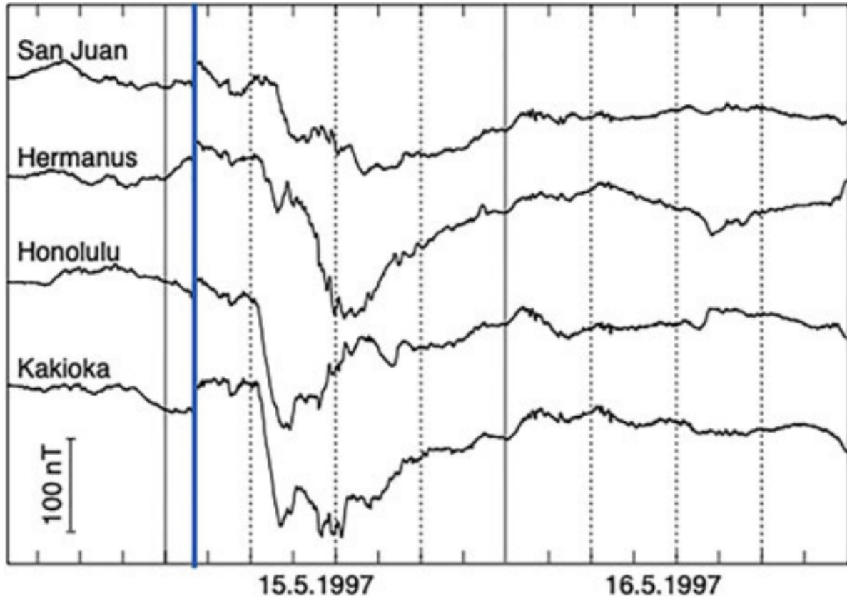
Figure 22.10: The horizontal component (H) of the magnetic field measured at four low-latitude stations during a magnetic storm on 15 May 1997. An ICME-driven solar wind shock hit the magnetosphere on 15 May at about 02 UT causing the storm sudden commencement which is indicated by a sudden positive jump of the H component at all stations (thick blue line). The main phase of the storm started after 06 UT as indicated by the strong negative deviation in the H component. The solid vertical lines give the UT midnight and the tick-marks on the horizontal axis are given for each 3 h.
