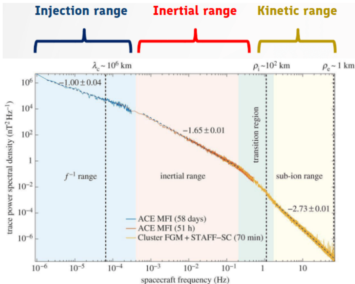
Figure 18.4: Solar wind power spectrum from Kiyoni+, 2015.
