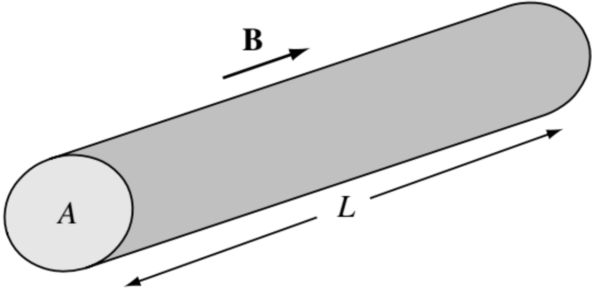
Figure 8.1: Magnetic flux tube with flux \Phi = BA .
