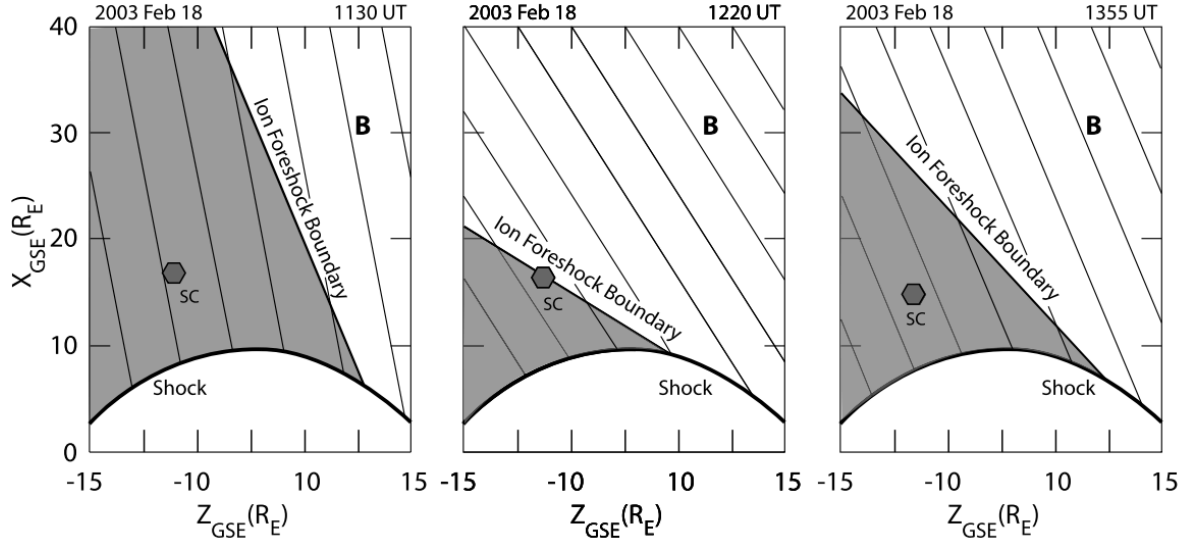
Figure 21.16: Reconstruction of the shape and location of the ion-foreshock boundary from the measured upstream plasma properties (direction of magnetic field, speed and density) for three successive times in order to explain the ion-phase space observations in Figure 21.15. The cold magnetic field-aligned ion beam is observed when the spacecraft is located in the vicinity of the ion-foreshock boundary at 1220 UT, while at 1130 UT and 1355 UT no beam was detected. It is assumed that the beam is generated along the foreshock boundary at the position where at the quasi-perpendicular shock surface the shock-normal angle is roughly about \theta_{Bn} \sim 60^\circ .
