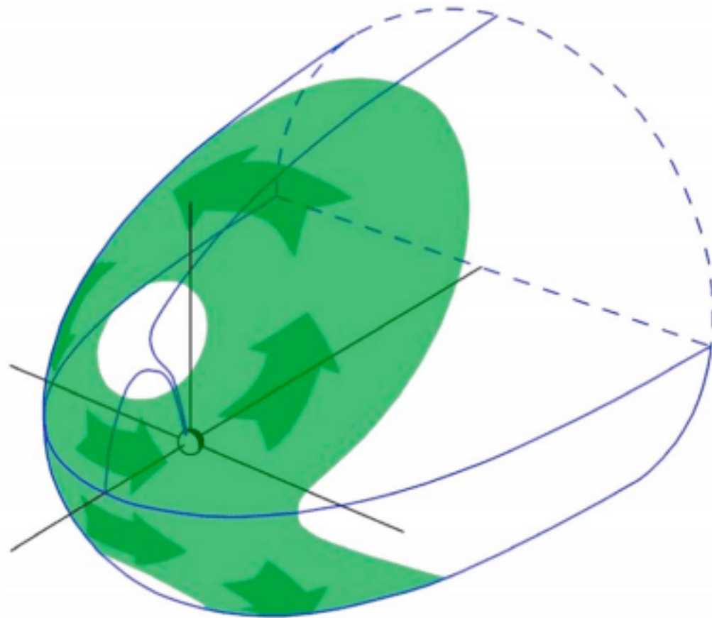
Figure 22.2: The Chapman-Ferraro dayside magnetopause currents are shown as a green-shaded surface on a simple wire diagram of the magnetopause. The Earth is the small sphere at the axis origin, and the Sun is to the lower left.
