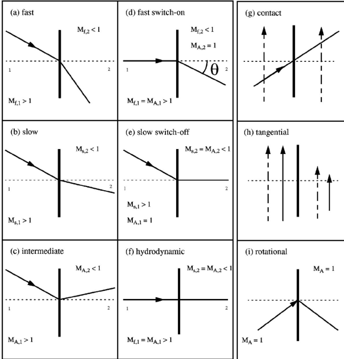
Figure 21.1: Some properties of MHD shocks and discontinuities. The thick vertical line is the shock surface. The shock normal is dotted. The full arrowed lines are magnetic field lines that are refracted through the shock surface. The dashed arrowed lines are velocity vectors. Region 1 is upstream, 2 is downstream. Reprinted from De Sterck et al. (1998).
