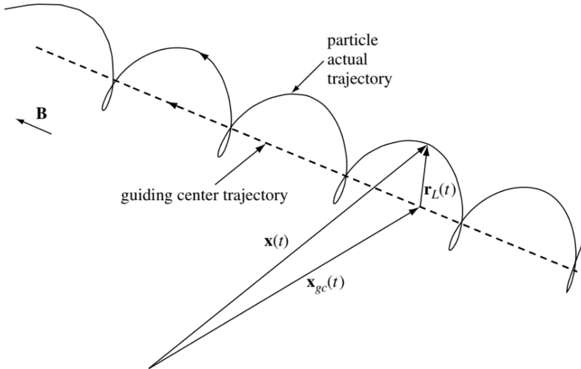
Figure 7.1: Drift in an arbitrarily complicated field.
