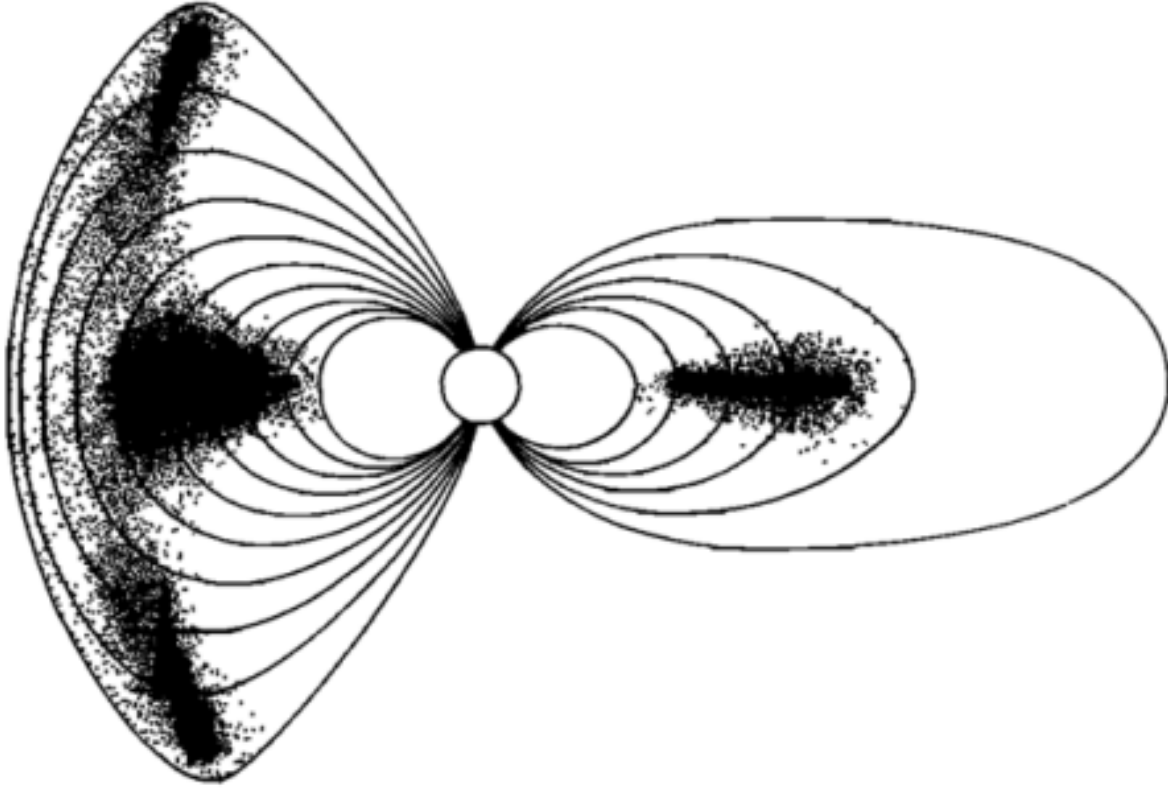
Figure 22.11: Schematic sketch of chorus/EMIC wave excitation regions, denoted by dots, on the noon-midnight meridian plane.
