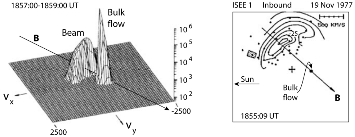
Figure 21.14: ISEE 1 observation of a reflected ion beam on November 19, 1977 propagating along a magnetic field line that was connected to the quasi-parallel Earth's bow shock. Left: A two-minute average pseudo-3D ion velocity-space profile in the (v_x, v_y) -plane showing the undisturbed and cold (narrow) plasma inflow in negative v_x -direction, and the fast and warm (broad) beam of reflected ions propagating in positive v_x -direction and spreading in v_y . This beam is quite anisotropic in temperature. Velocities are in \text{km s}^{-1} . The scale on the right is count rates, and background count rates were suppressed by choosing only values above 50 \text{ s}^{-1} . Right: Contour plot of a similar beam a little earlier showing that the beam is centred on the magnetic field that connects to the shock, is quite narrow along the field and about 2–3 times as broad perpendicular to the field [data from Paschmann et al, 1981]. The cross indicates the origin (zero velocity), the dot the bulk flow centre. The 10^{-25} \text{ s}^3 \text{ cm}^{-6} level flux contour has been marked.
