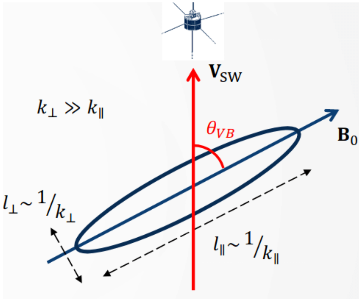
Figure 18.2: Wave scale from typical L1 satellite solar wind observation.
