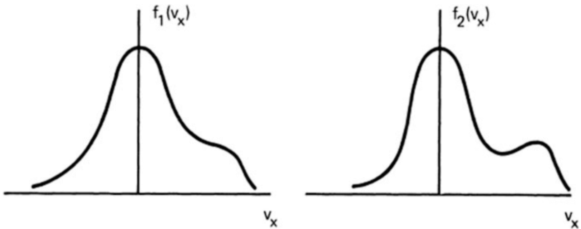
Figure 12.2: Examples of non-Maxwellian distribution functions
