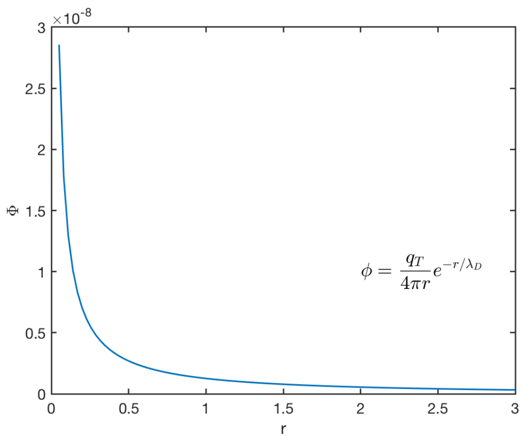
Figure 2.1: Electric potential.
