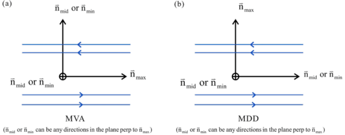
Figure 19.1: a) MVA (MGA) and b) MDD eigenvectors \vec{n}_{\text{max}}, \vec{n}_{\text{mid}}, \vec{n}_{\text{min}} , corresponding to largest, middle and minimum eigenvalues in a 1-D current sheet.
