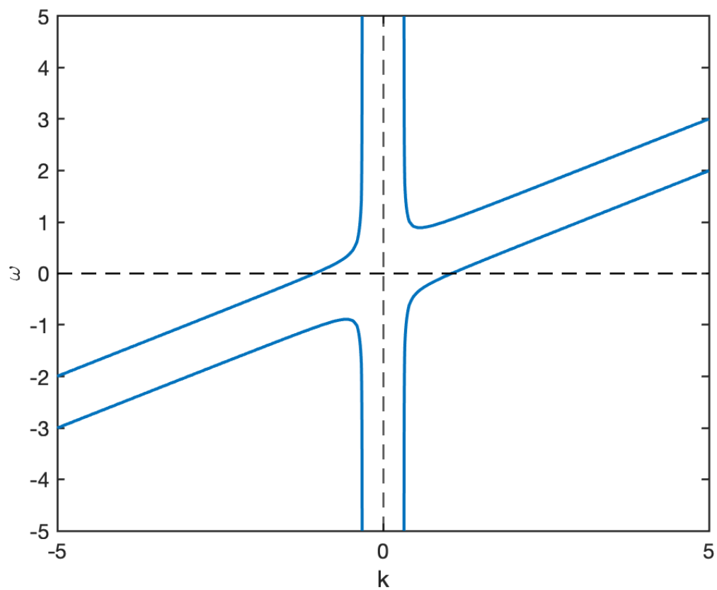
Figure 13.3: 2-stream dispersion relation.
