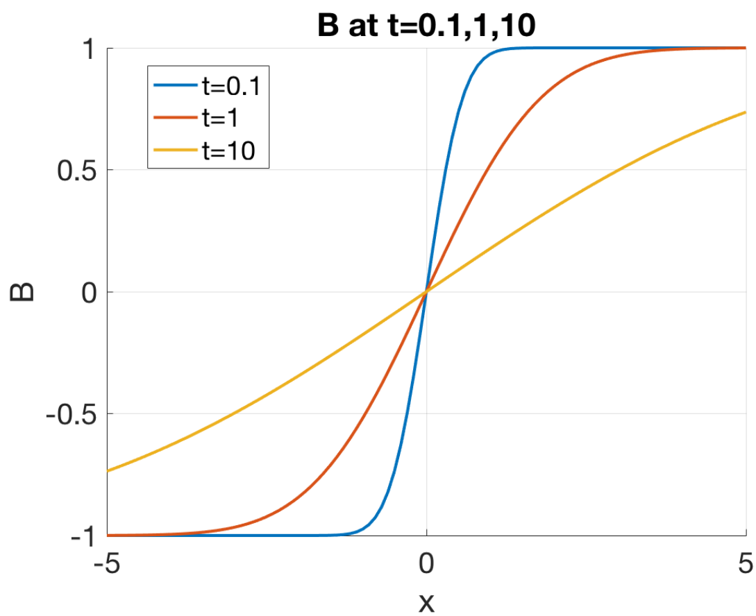
Figure 9.2: Magnetic field at t = 0.1, 1, 10 , respectively.
