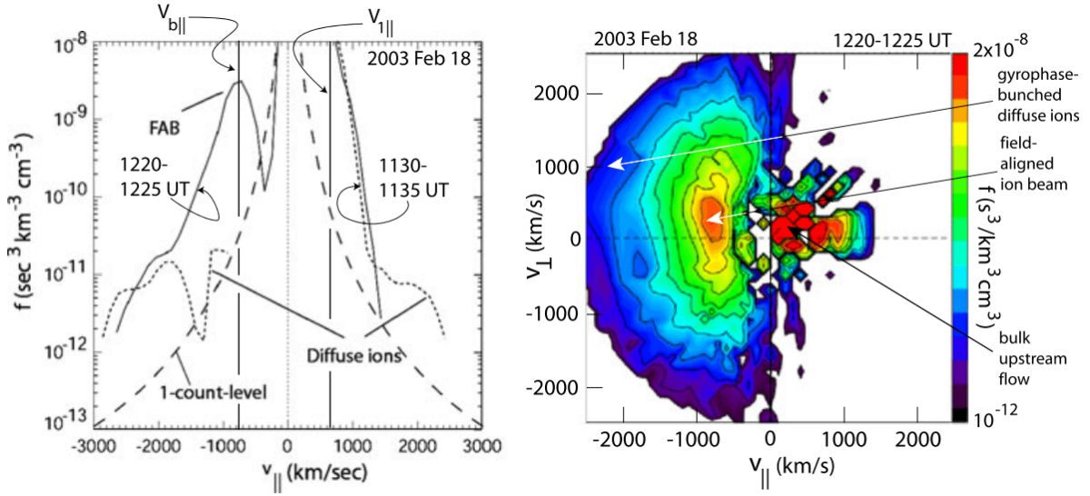
Figure 21.15: Left: The reduced field-aligned ion distribution functions in the foreshock region showing the field-aligned reflected ion beam (FAB) at 1220–1225 UT on February 18, 2003 which arrives at the spacecraft location along the magnetic field line that is connected to the quasi-perpendicular region of the Mach number M_A \sim 8 supercritical shock (smooth solid line). The upstream bulk velocity was V_1 \simeq 660 \text{ km s}^{-1} . Also shown is the reduced parallel distribution function (dashed) for the diffuse ion distribution observed at 1130–1135 UT the same day (for the geometry see Figure 6.7). It is clearly seen that the latter is about symmetric to the magnetic field direction indicating the symmetry of the ring of diffuse ions, while the foreshock-boundary field-aligned beam is flowing in the direction away from the shock into the upstream medium (negative velocities). Note also that the diffuse distribution appears as a smooth tail on the full ion distribution. The small gap on the left is uncertain as it dips into the 1-count level. Right: The two-dimensional phase space plot for the time interval 1220–1225 UT when the field-aligned beam was observed. Indicated are the bulk upstream flow, field-aligned ion beam, and the gyro-phase bunched residue of the diffuse upstream ions (data from Kis et al. 2004).
