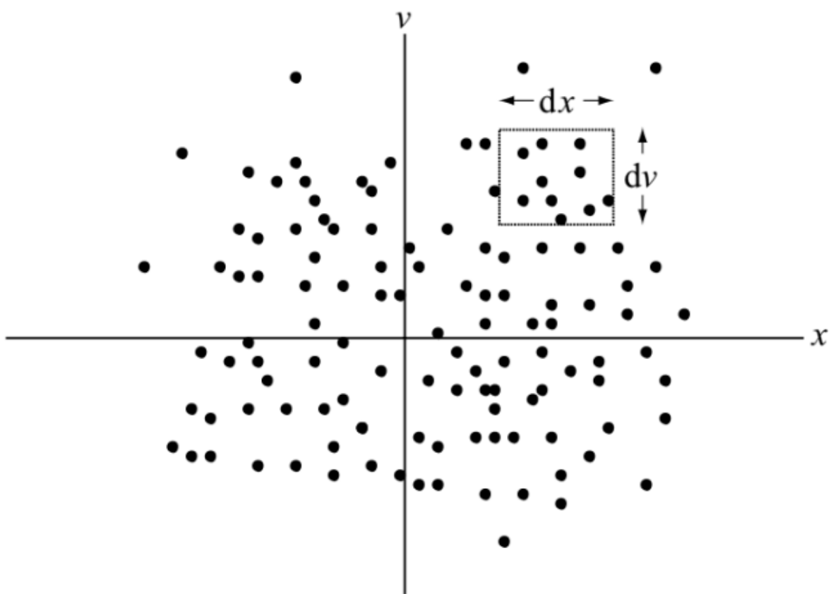
Figure 12.4: A box within phase-space having width dx and height dv .
