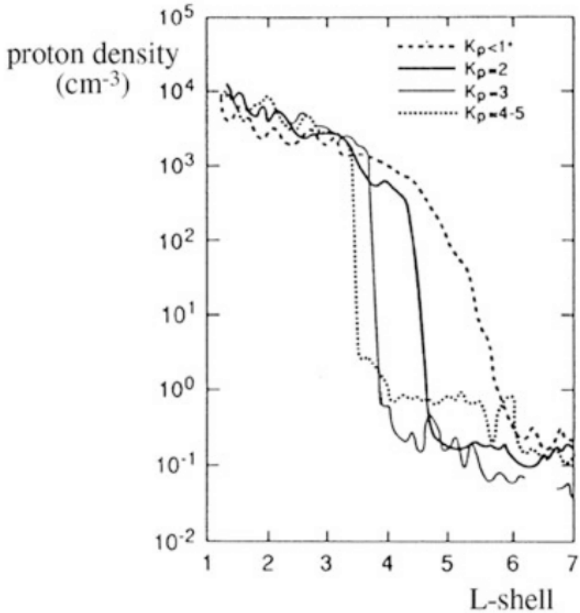
Figure 22.7: Plasma density in the night sector organized by the activity index K_p . K_p < 1+ corresponds to a very quiet magnetosphere, whereas K_p = 4-5 indicates a significant activity level, although not yet a big magnetic storm. The L-shell is defined in Equation 22.2. [Chappell (1972)]
