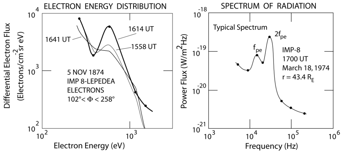
Figure 21.25: Left: The electron energy distribution as seen by IMP-8 at three times when crossing the foreshock boundary. Right: The high-frequency wave spectrum of the electromagnetic radiation as measured some distance away from the shock near the foreshock boundary. Two types of emissions are visible, the so-called ‘harmonic’ emission f = 2f_{pe} at twice the electron plasma frequency f_{pe} = \omega_{pe}/2\pi , and the weaker so-called ‘fundamental’ emission at f_{pe} [after Gurnett & Frank, 1975].
