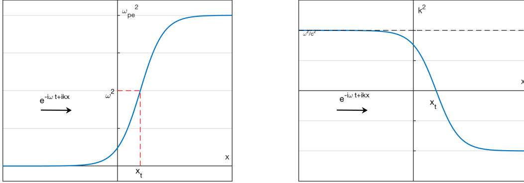
Figure 10.3: Plasma frequency and wave number as functions of x in a non-uniform plasma for O mode.
