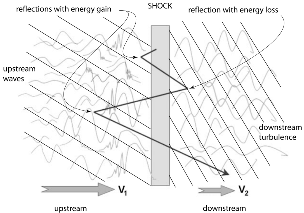
Figure 21.39: Schematic of the acceleration mechanism of a charged particle in reflection at a quasi-parallel ( \theta_{Bn} < 45^\circ ) supercritical shock. The upstream plasma flow (left, V_1 \gg V_2 ) contains the various upstream plasma modes: upstream waves, shocklets, whistlers, pulsations. The downstream (right) is turbulent. The energetic particle that is injected at the shock to upstream is reflected in an energy gaining collision with upstream waves, moves downstream where it is reflected in an energy losing collision back upstream. It loses energy because it overtakes the slow waves, but the energy loss is small. Returning to upstream it is scattered a second time again gaining energy. Its initially high energy is successively increased until it escapes from the shock and ends up in free space as an energetic Cosmic Ray particle. The energy gain is on the expense of the upstream flow which is gradually retarded in this interaction. However, the number of energetic particles is small and the energy gain per collision is also small. So the retardation of the upstream flow is much less than the retardation it experiences in the interaction with the shock-reflected low energy particles and the excitation of upstream turbulence.
