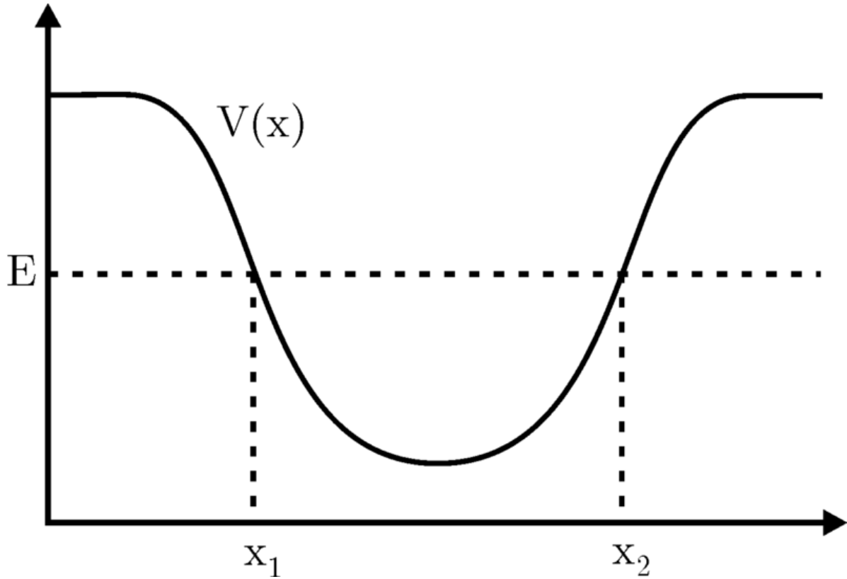
Figure 3.6: Potential well.
