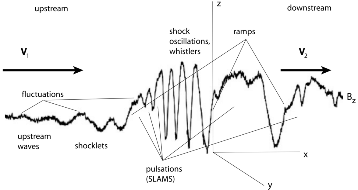
Figure 21.12: Schematic 1D profile taken along the nominal instantaneous shock normal of a supercritical quasi-parallel shock as seen in the magnetic field component B_z . This is the analogue to the quasi-perpendicular shock profile. It shows the main features in the vicinity of the quasi-parallel shock transition: the large amplitude upstream waves with the turbulent fluctuations on top of the waves, the formation of shocklets, i.e. steep flank formation on the waves exhibiting small-scale fluctuations on top of the wave, which act already like small shocks, very-large amplitude pulsations (magnetic pulsations or SLAMS) which turn out to be the building blocks of the shock, multiple shock-ramps at the leading edges of the pulsations belonging to diverse ramp-like steep transitions from upstream to downstream lacking a clear localization of the shock transition and any attached phase-locked whistlers. (Note that the entire figure is, in fact, the shock transition, as on this scale no clear decision can be made where the shock ramp is located.) Not shown here are the out of plane oscillations of the magnetic field that accompany the waves and the particle phase space.
