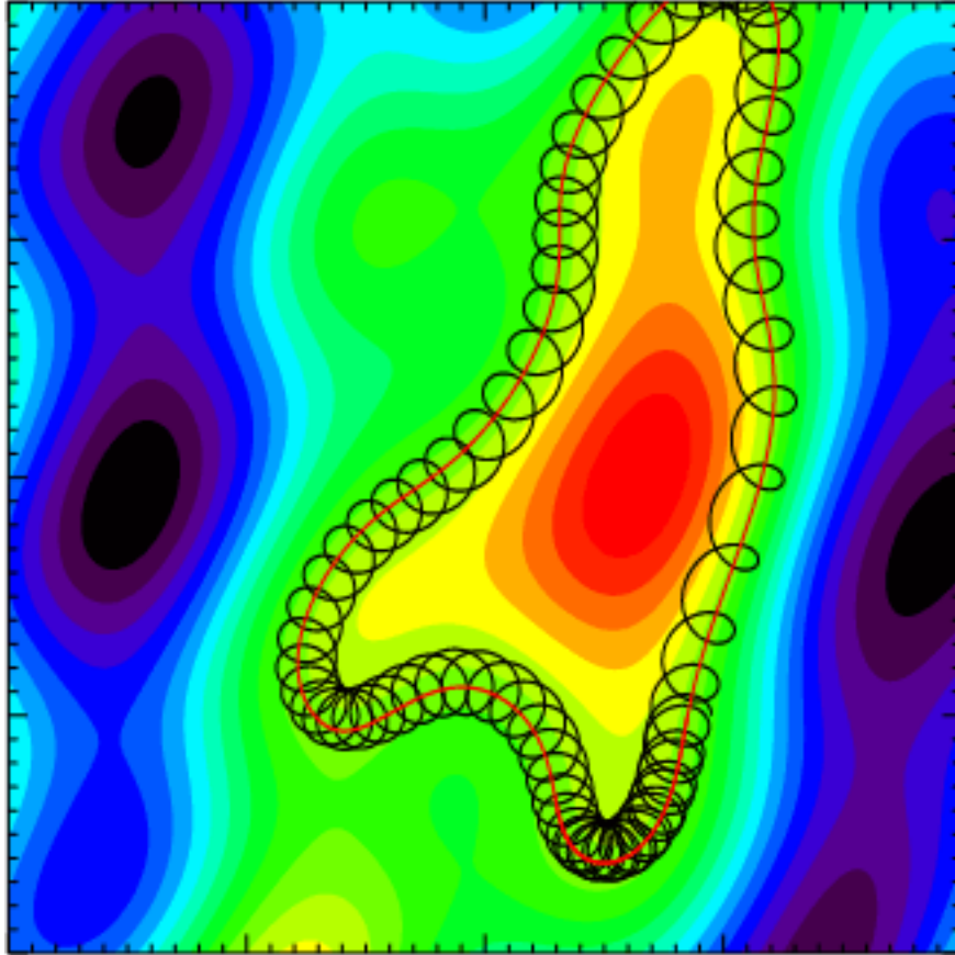
Figure 15.1: Charged particle orbit in a magnetic field pointing into the plane with electrostatic potential fluctuations.
