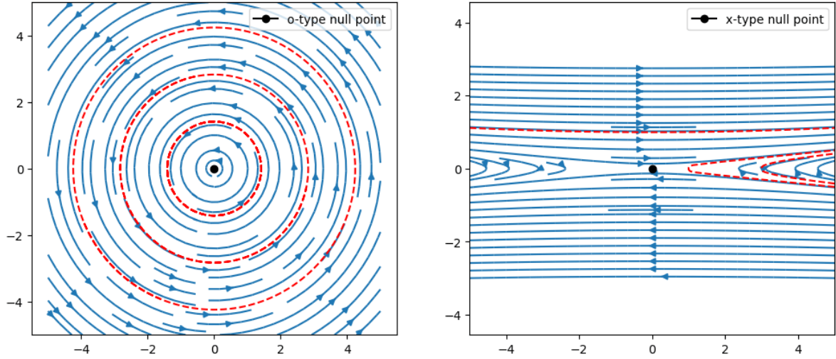
Figure 19.2: Example of (a) O-point and (b) X-point.
