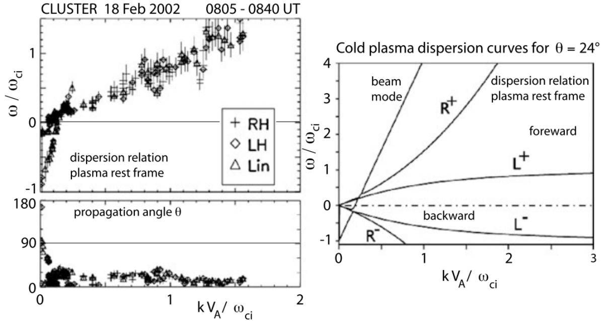
Figure 21.23: Left: The dispersion relation of low-frequency waves as measured by CLUSTER in the foreshock away from the foreshock boundary [data taken from Narita & Glassmeier, 2005], determined from the “wave-telescope” analysis method. The upper panel shows the dispersion relation \omega(k) consisting of several parts and distinguished by the sense of polarization as right-hand, left-hand and linear. The different branches cluster. There are forward (positive frequency parallel to the magnetic field) and backward (negative frequency antiparallel) branches. The lower panel shows the wave propagation angle for the shorter wavelengths being mostly oblique near \theta \approx (30 - 25)^\circ , for longer wavelengths being more perpendicular to the magnetic field. Right: The five low-frequency modes in a cold beam plasma system of similar conditions as the foreshock plasma and for the propagation angle \theta = 24^\circ showing similarity to the observed dispersion relation [data from Narita et al, 2003].
