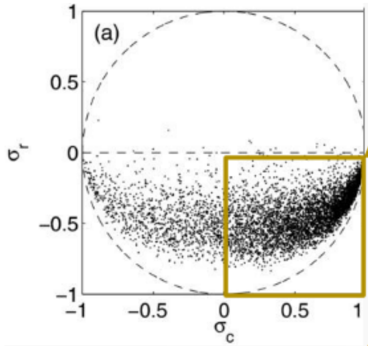
Figure 18.1: Solar wind normalized residual energy and cross helicity statistics from Chen+ 2013.
