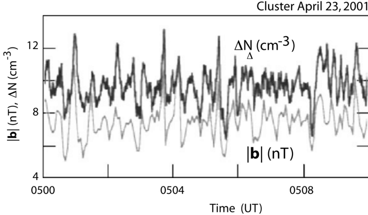
Figure 21.22: Left: The excellent correlation between the density and magnetic field variations in the ion-beam excited foreshock-boundary low-frequency waves as measured by CLUSTER [data from Eastwood et al, 2002]. The variations are practically in phase thus identifying the fluctuations as fast magnetosonic.
