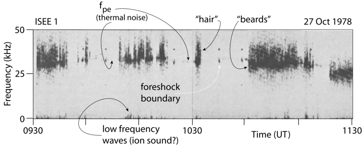
Figure 21.28: An example of ISEE 1 high frequency wave observations during contact and passage of the electron foreshock boundary. The thin faint spotty line around 30–40 kHz is the local plasma frequency f_{pe} \sim 30 kHz, seen here only as thermal noise with lesser instrumental sensitivity than in the CLUSTER observations. The occasional intense dark spots as the one marked by the white arrow are brief contacts with the foreshock boundary field line when the beam occurs. deeper in the foreshock the spectrum broadens nonsymmetrically, evolving ‘hair’ and ‘beards’. Some moving structures can be identified in the hair. The emissions deeper inside the foreshock are correlated with the occurrence of low frequency emissions below a few kHz which are probably ion-sound waves [after Etcheto & Faucheux, 1984].
