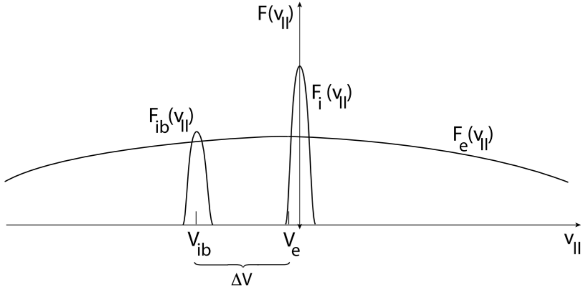
Figure 21.20: Reduced parallel distribution functions along the ion-foreshock boundary showing the cold main flow ion distribution F_i(v_{\parallel}) , the hot main flow electron distribution F_e(v_{\parallel}) shifted to the left into the direction of the foreshock ion beam for keeping zero-current conditions, and the ion-foreshock ion beam distribution F_{ib}(v_{\parallel}) . This configuration is unstable with respect to ion-ion beam instabilities and the ion-beam driven ion-acoustic instability.
