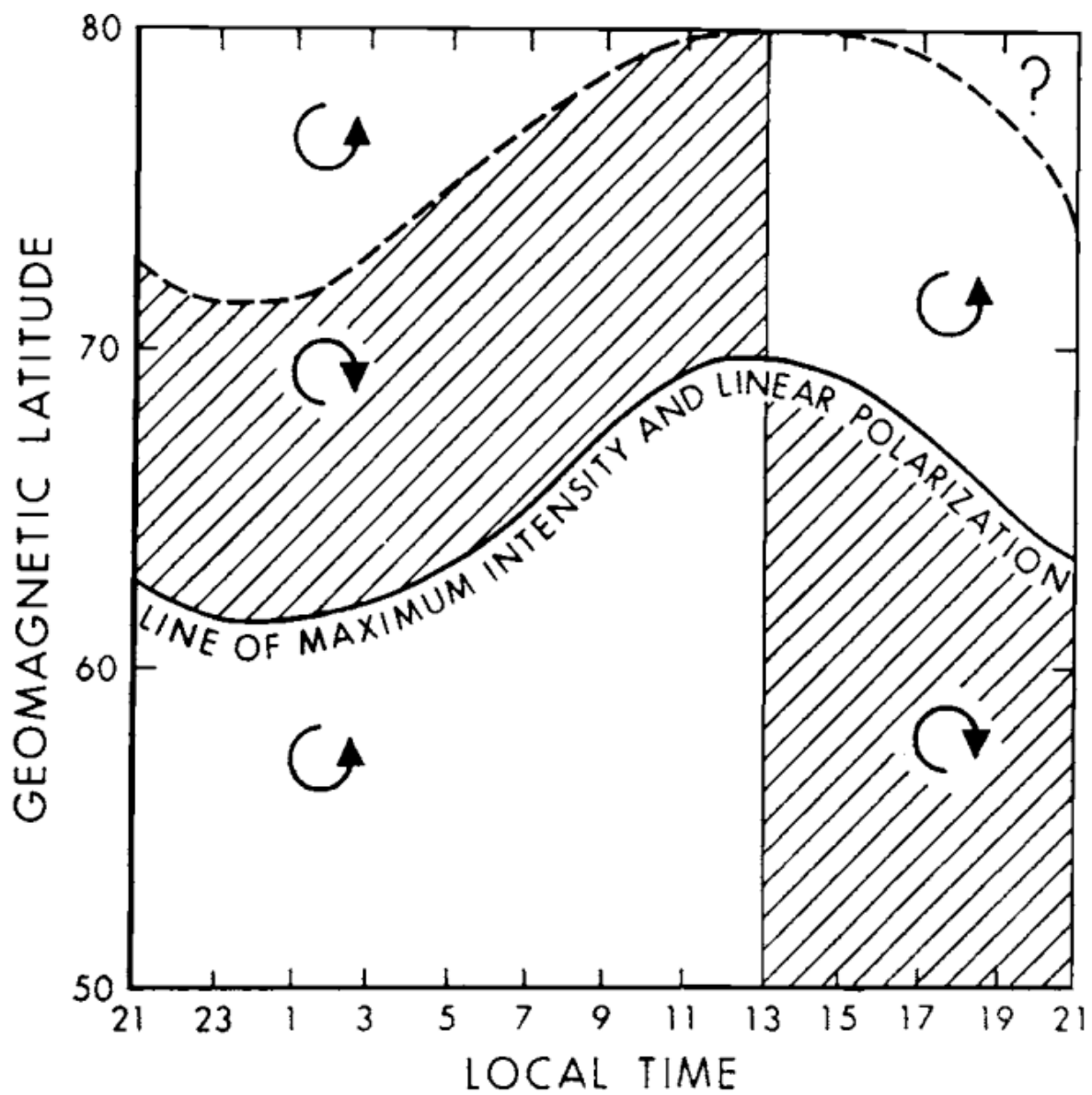
Figure 16.4: The variation of amplitude and the sense of polarization of Pc5's seen at high latitudes with latitude and magnetic local time. (After [Samson +, 1974].)
