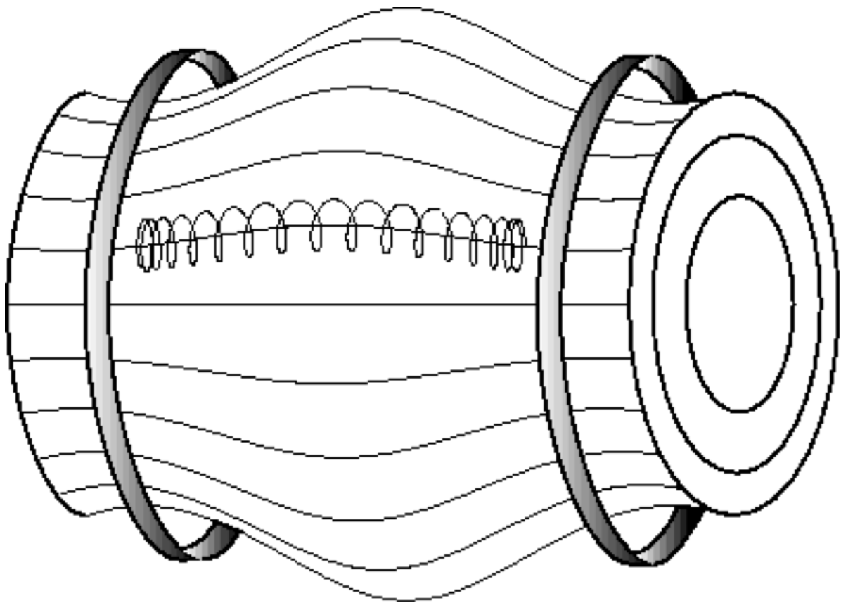
Figure 13.2: Basic magnetic mirror configuration.
