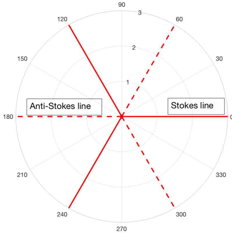
Figure 3.4: Stokes lines and anti-Stokes lines for WKBJ solution of Airy Equation.
