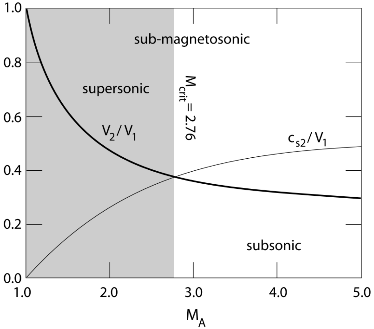
Figure 21.2: Dependence of the downstream normalised flow V_2/V_1 and sound c_{s2} velocities on the upstream Alfvén Mach number for an ideal MHD perpendicular shock with zero upstream pressure P_2 = 0 . The crossing of the two curves defines the critical Mach number which is M_c = 2.76 .
