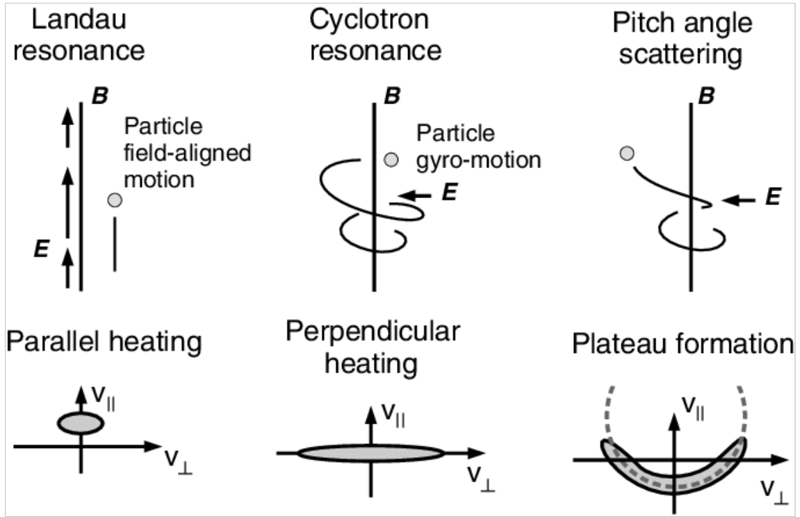
Figure 10.4: Wave-particle interactions and the associated part of the velocity distribution functions. Courtesy of Yasuhito Narita.
