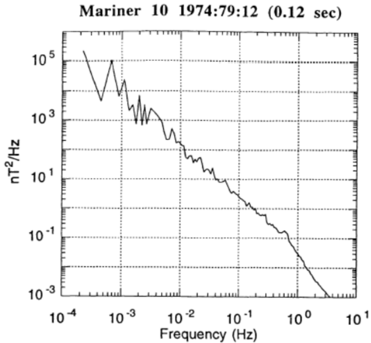
Figure 18.3: Solar wind magnetic field spectrum from Goldstein, Roberts, Matthaeus (1995).
