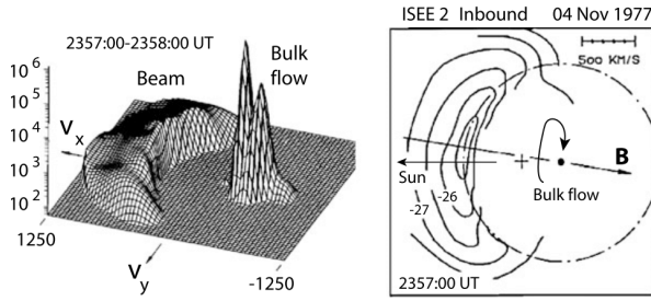
Figure 21.17: Left: A one-minute average pseudo-3D ion velocity-space profile in the (v_x, v_y) -plane showing the spreading of the beam in angle around the bulk flow without merging into the bulk flow. Right: Contour plot of the partial ring distribution.
