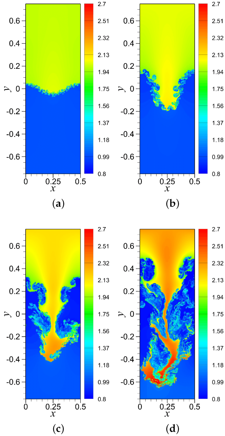
Figure 13.6: Simultaion of Rayleigh-Taylor instability (Rahman and San 2019).
