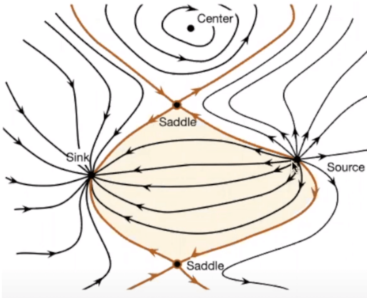
Figure 19.6: Identification of separatrices in 2D.
