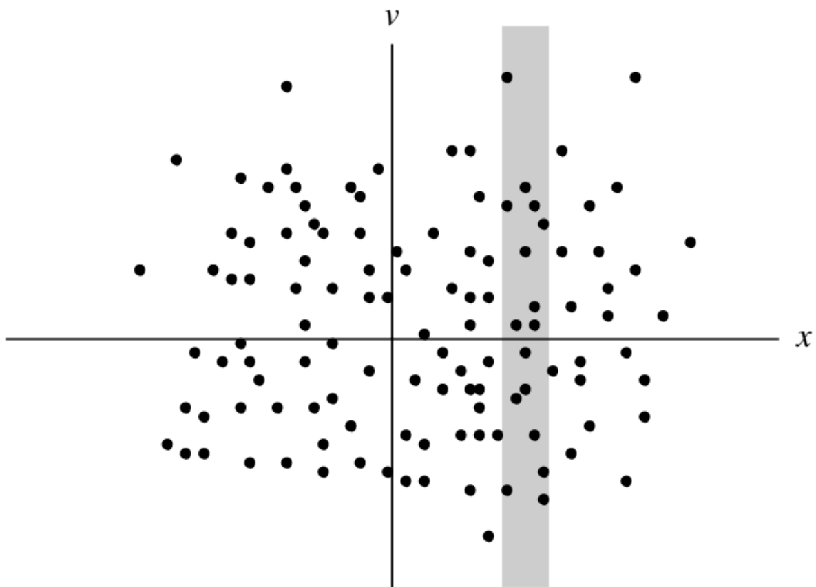
Figure 12.3: Moments give weighted averages of the particles in the shaded vertical strip.
