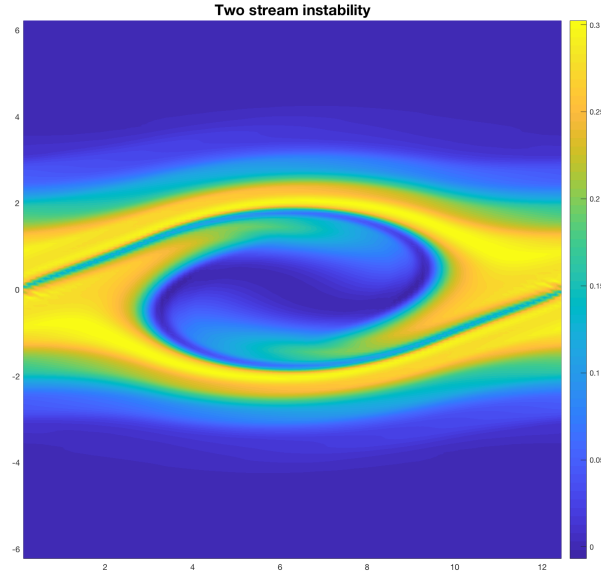
Figure 13.5: 2-stream velocity space distribution.
