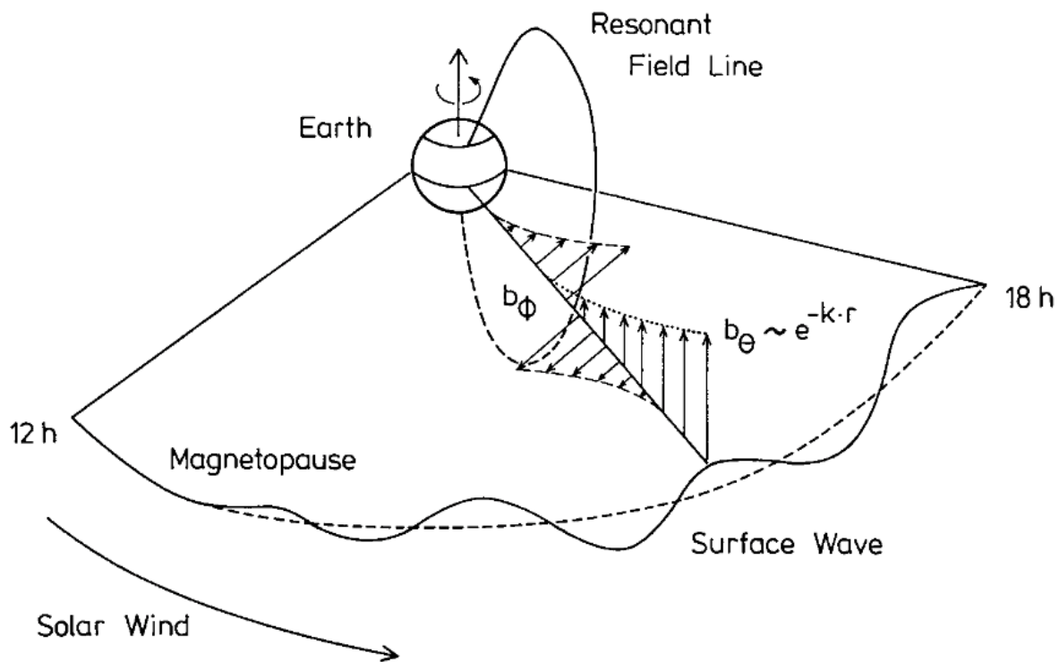
Figure 16.6: Schematic view of the field line resonance, driven by unstable surface wave.
