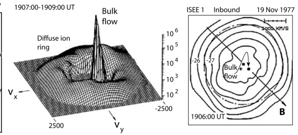
Figure 21.18: Left: A two-minute average pseudo-3D ion velocity-space profile in the (v_x, v_y) -plane showing the undisturbed and cold (narrow) plasma inflow in negative v_x -direction about centred and surrounded by a ring distribution of fast and warm (broad) diffuse ions that have been reflected from the shock but have been processed in the foreshock region when propagating from the foreshock boundary into the foreshock. These ions are hollow in the sense that they separate from the bulk distribution but have a nearly isotropic distribution function. Right: Contour plot of a similar ring a little earlier showing that the ring centre (star) is slightly displaced from the bulk flow (dot) on the magnetic field that connects to the shock and from the centre (cross) of the phase space frame.
