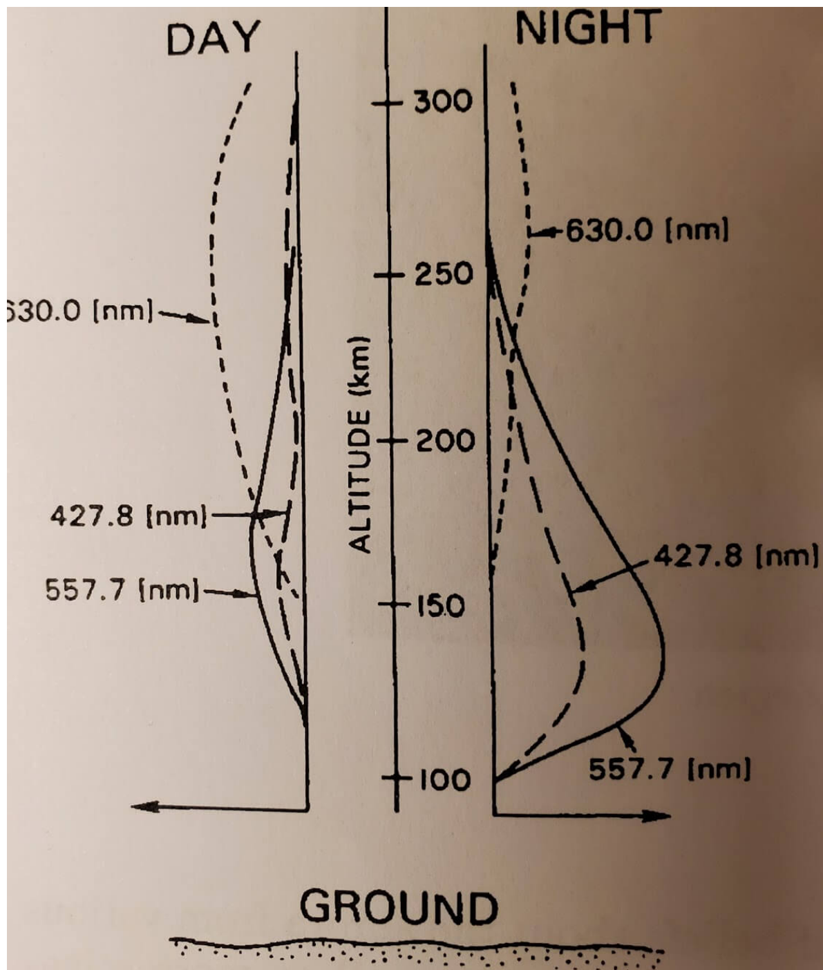
Figure 25.1: The altitude distribution of auroral emissions at day and night.
