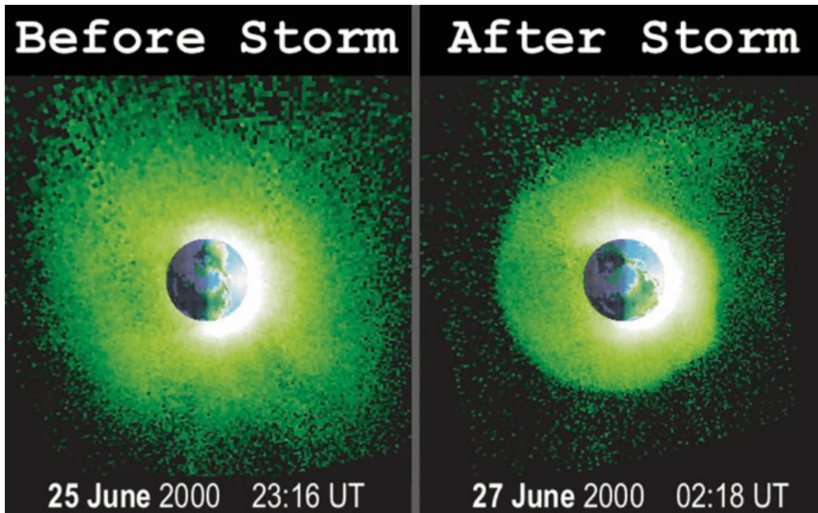
Figure 22.8: Plasmapheric plume and plasmaspheric erosion as observed by the IMAGE EUV instrument. The picture is taken from above the northern hemisphere and the Sun is to the right. (Goldstein+2004)
