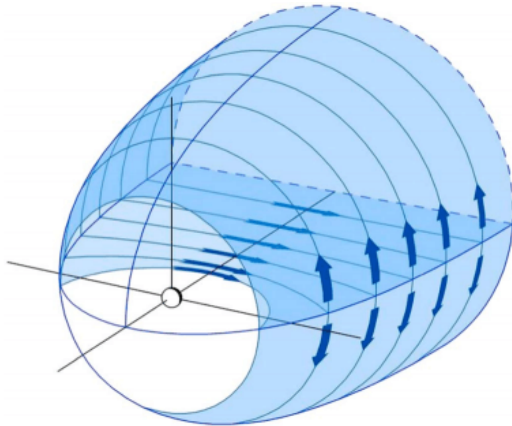
Figure 22.3: The tail current with closure via return current on magnetopause shown in light blue on the wire diagram of the magnetopause, as in Figure 22.2.
