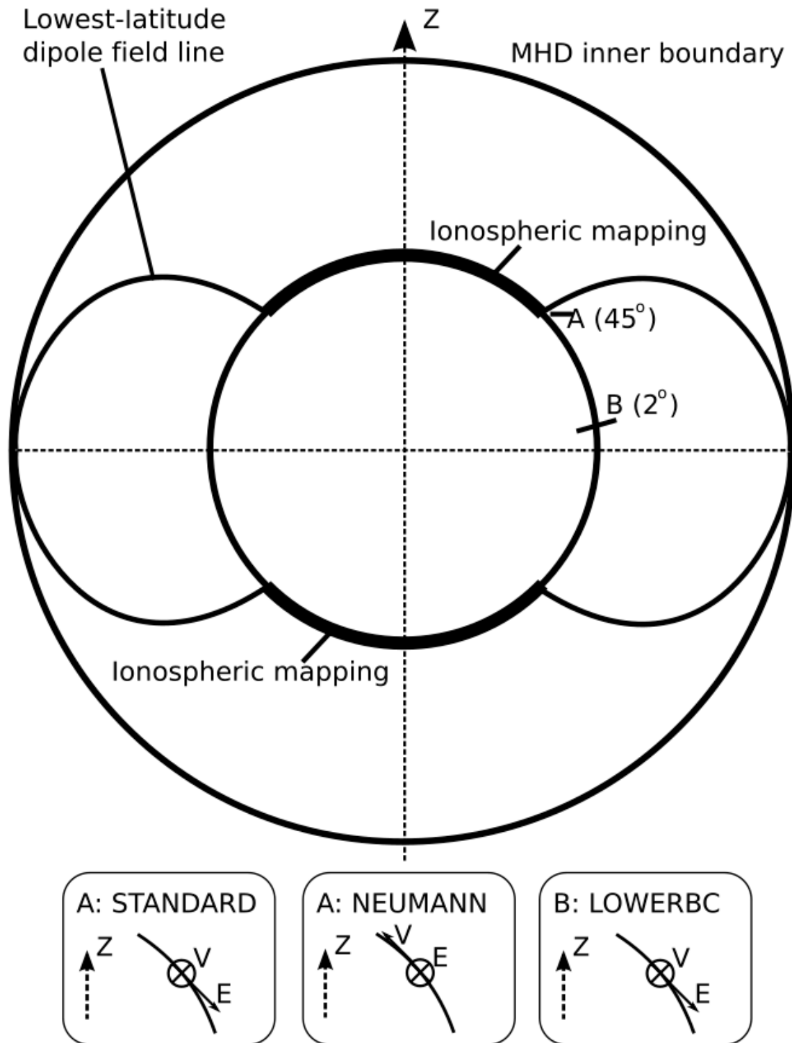
Figure 23.1: A schematic depiction of the inner boundary of the magnetosphere simulation and its ionospheric mapping. The location of the low-latitude boundary of the ionospheric grid is determined by the radius of the inner MHD boundary mapped along the dipole field from the equator. Point A (at 45^\circ ) denotes a typical location of the low-latitude boundary, where the STANDARD and NEUMANN boundary conditions are applied, while point B is where the LOWERBC boundary condition is applied. The three inset plots at the bottom depict schematically the configuration of velocity and electric field vectors with respect to the surface of the ionosphere in a meridional plane. The inset plot titles identify the type of the boundary condition and the point where it is applied. Adopted from (Merkin and
