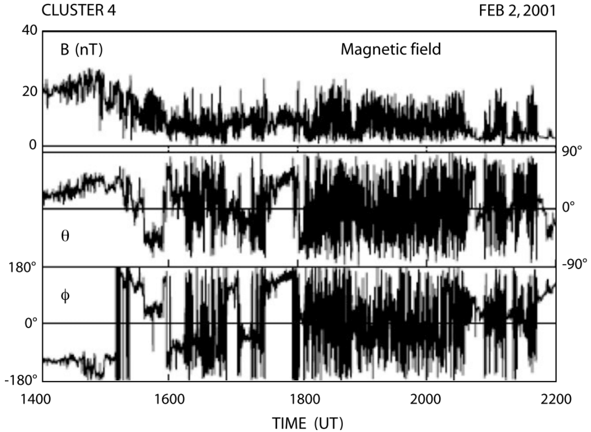
Figure 21.32: Eight hours of CLUSTER magnetic field data during a long passage near and across the quasi-parallel supercritical (Alfvénic Mach number M_A \sim 12 - 13 , ion inertial length d_i \sim 140 km) bow shock. The time resolution was 4 s. The top panel shows the variation in the magnitude of the magnetic field. The two lower panels are the respective elevation and azimuthal angles \theta , \phi in a GSE coordinate frame (Lucek et al. 2002). Large variation in the magnetic compression and direction can be seen to be associated with this quasi-parallel shock crossing. Buried in these large variations on this highly time-compressed scale are many magnetic pulsations (SLAMS). The compressive large amplitude fluctuations in the upper panel are typical for a quasi-parallel shock transition.
