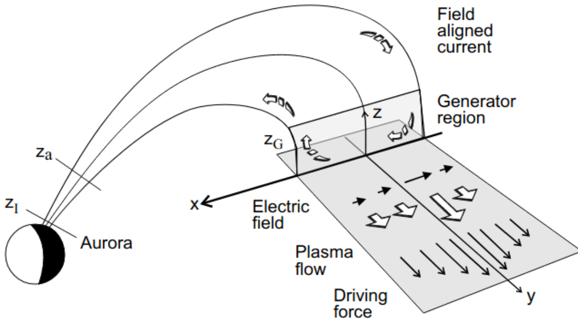
Figure 25.2: Geometry of the auroral current circuit and the generator region in the equatorial magnetosphere.
