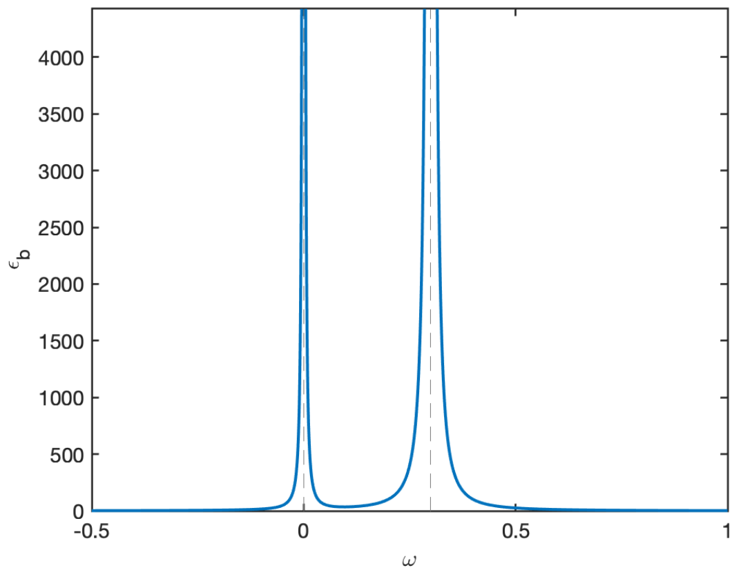
Figure 13.4: 2-stream dielectric function.
