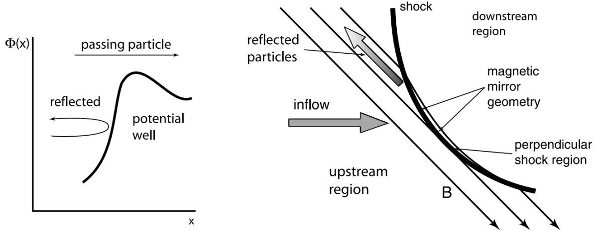
Figure 21.38: The two cases of shock reflection. Left: Reflection from a potential well \Phi(x) . Particles of energy higher than the potential energy e\Phi can pass while lower energy particles become reflected. Right: Reflection from the perpendicular shock region at a curved shock wave as the result of magnetic field compression. Particles move toward the shock like in a magnetic mirror bottle, experience the repelling mirror force and for large initial pitch angles are reflected back upstream.
