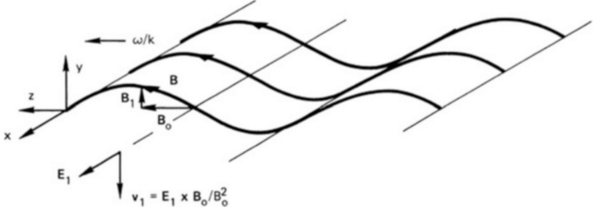
Figure 10.1: Relation among the oscillating quantities in an Alfvén wave and the (exaggerated) distortion of the lines of force.
