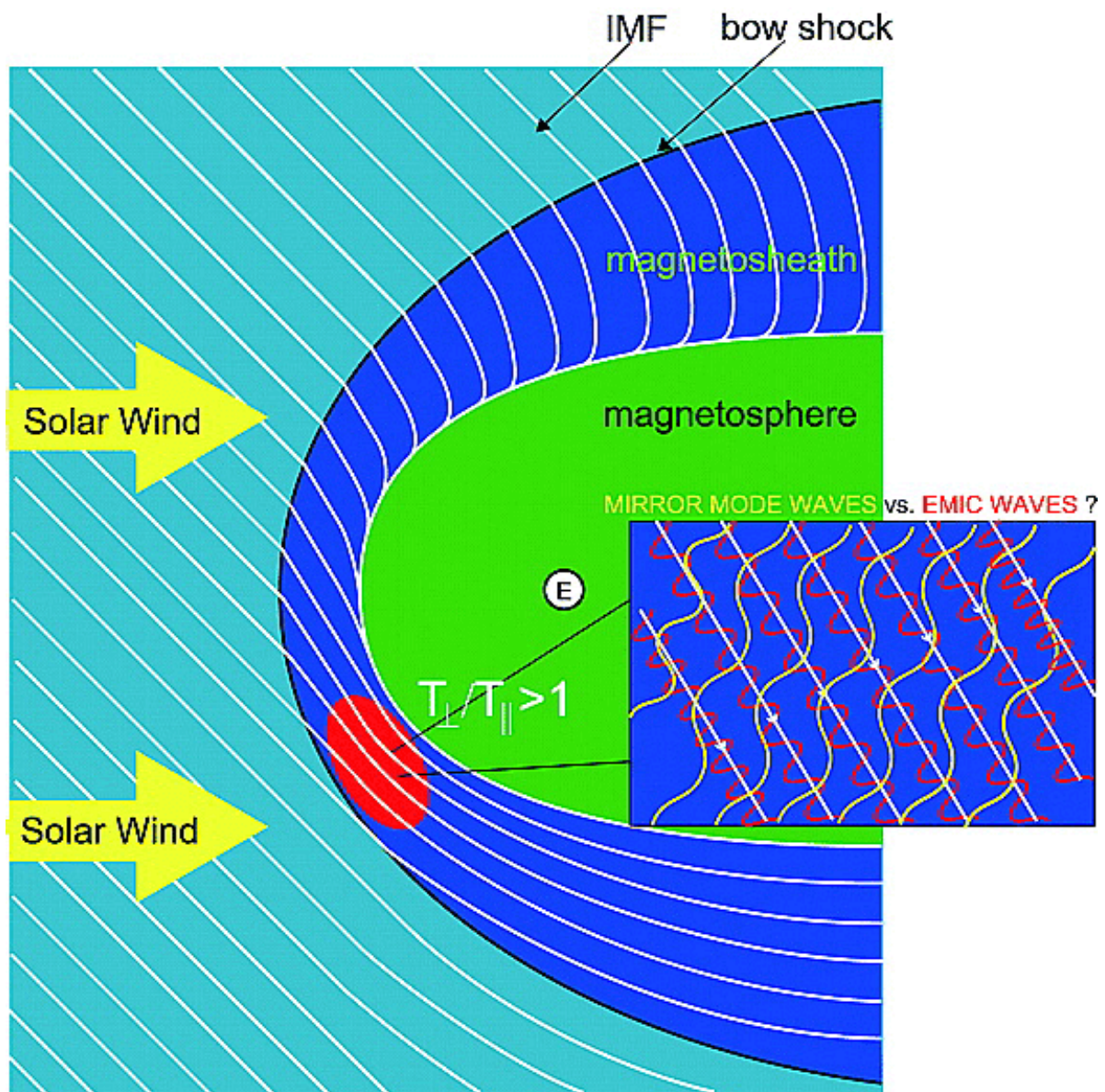
Figure 22.12: Mirror mode waves vs. EMIC waves in the magnetosphere.
