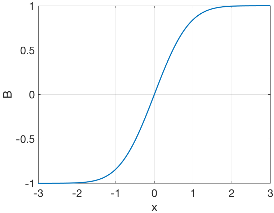
Figure 9.1: Error function.
