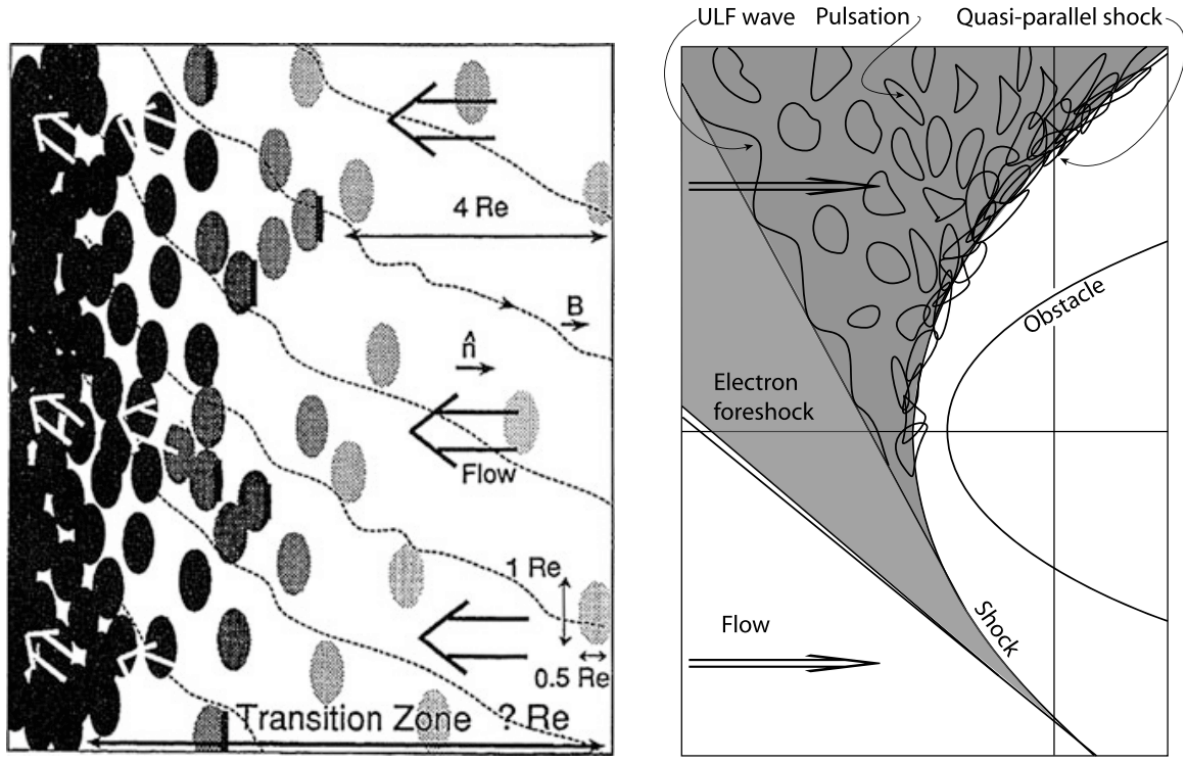
Figure 21.31: The patchwork model of Schwartz and Burgess (1991) of a quasi-parallel super-critical shock reformation. Left: Magnetic pulsations (SLAMS) grow in the ion foreshock and are convected toward the shock where they accumulate, thereby causing formation of an irregular shock structure. Note also the slight turning of the magnetic field into a direction that is more perpendicular to the shock surface with the shock surface itself becoming very irregular. Right: The same model with the pulsations being generated in the relatively broad ULF-wave-unstable region in greater proximity to the ion-foreshock boundary. When the ULF waves evolve to large amplitude and form localised structures these are convected toward the shock, grow, steepen, overlap, accumulate and lead to the build up of the irregular quasi-parallel shock structure which overlaps into the downstream direction.
