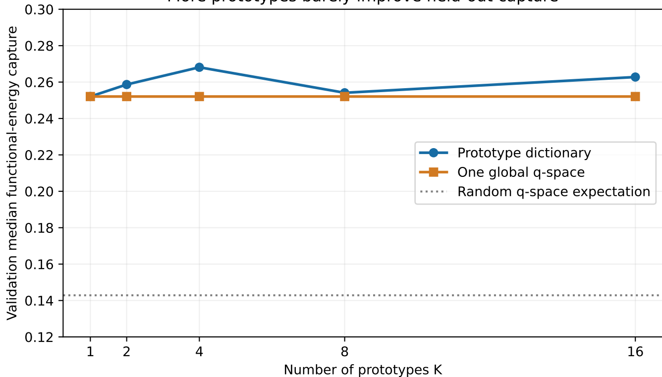
More prototypes barely improve held-out capture
