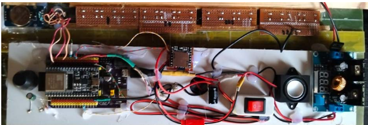
Inside the enclosure — the ESP32 expansion board and wiring. / Binne die behuising — die ESP32-uitbreidingsbord en bedrading.
