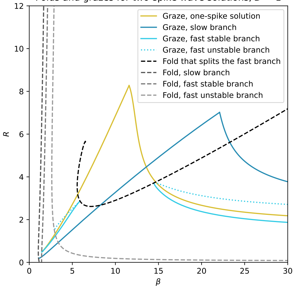
Folds and grazes for two-spike wave solutions, D = 1
