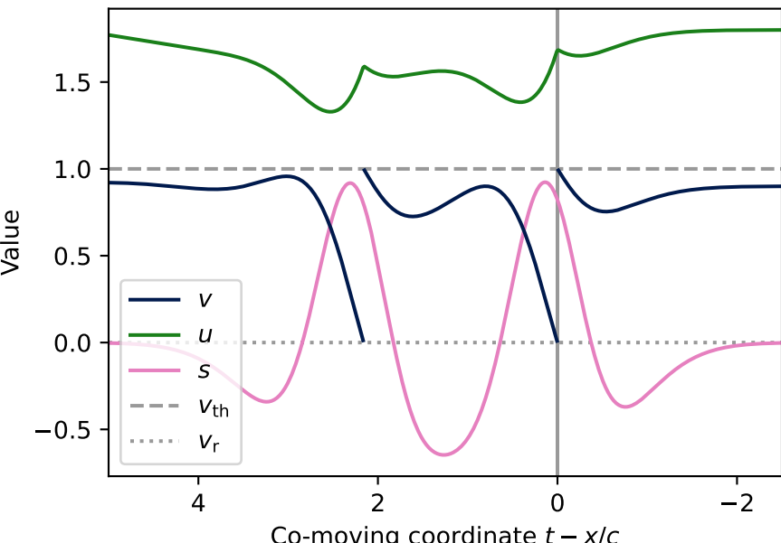
Travelling wave profile, c = 2.69
