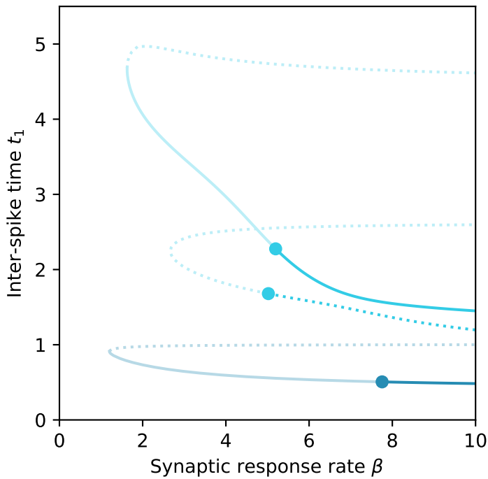
Wave solutions for given \beta ; R = 2.5
