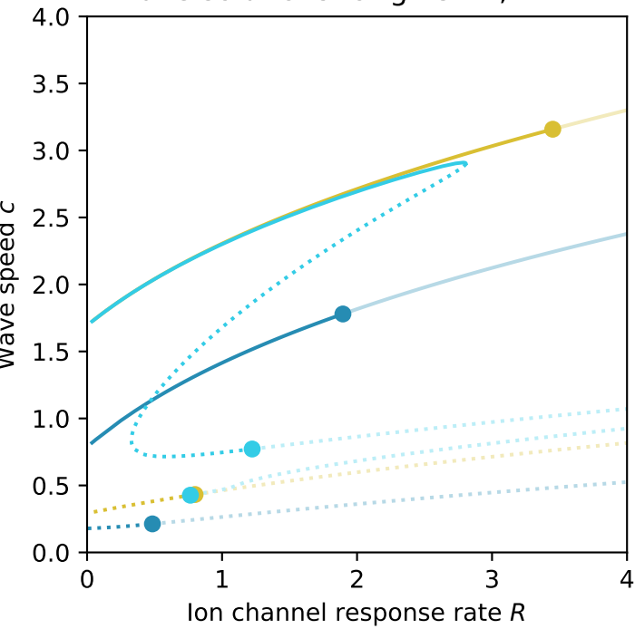
Wave solutions for given R ; D = 1
