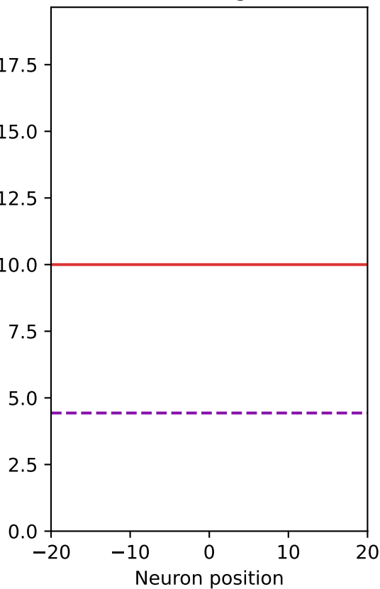
Neuron firing times
