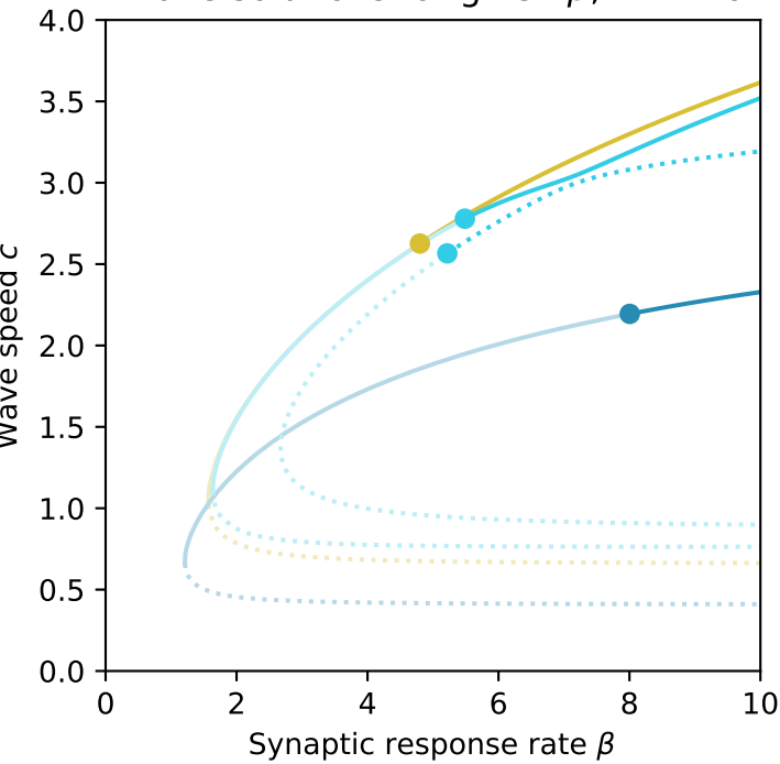
Wave solutions for given \beta ; R = 2.6
