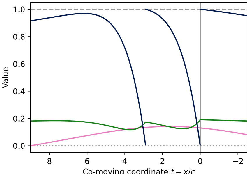
Travelling wave profile, c = 0.18
