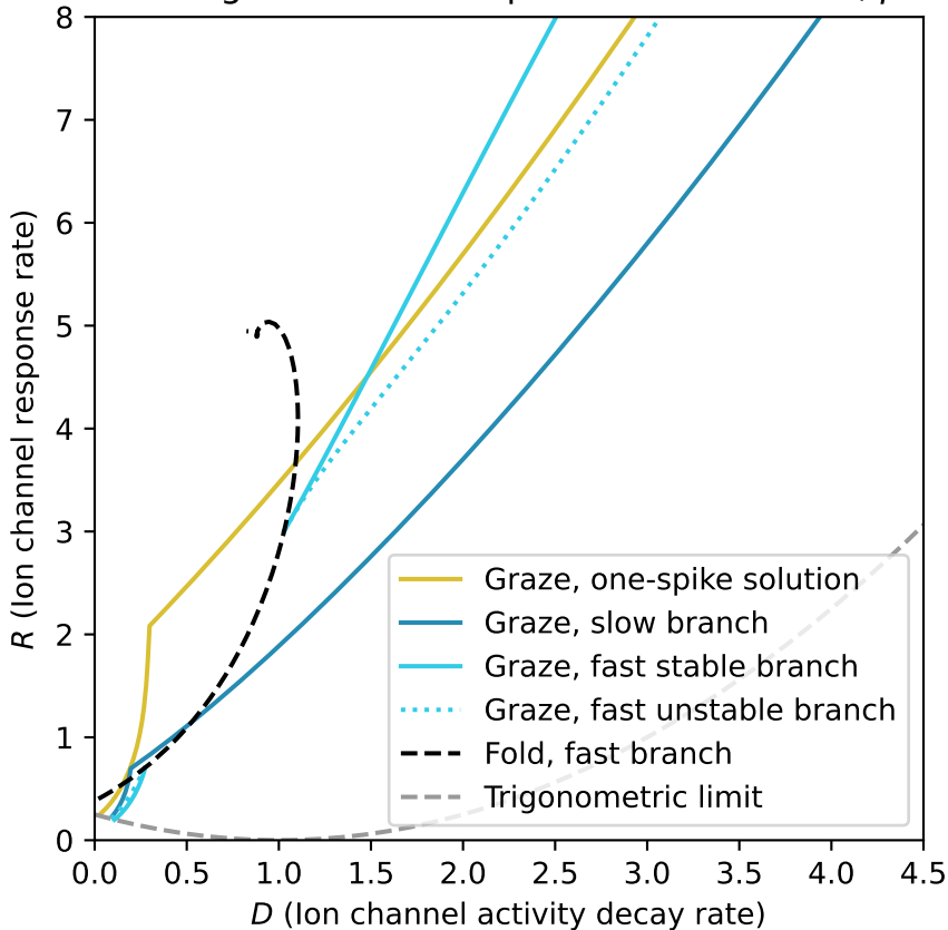
Folds and grazes for two-spike wave solutions, \beta = 6
