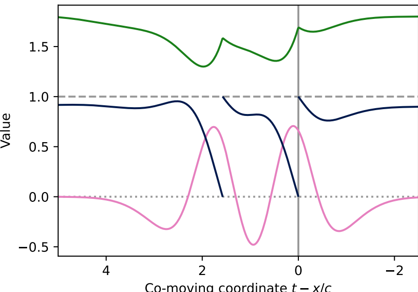
Travelling wave profile, c = 2.40
