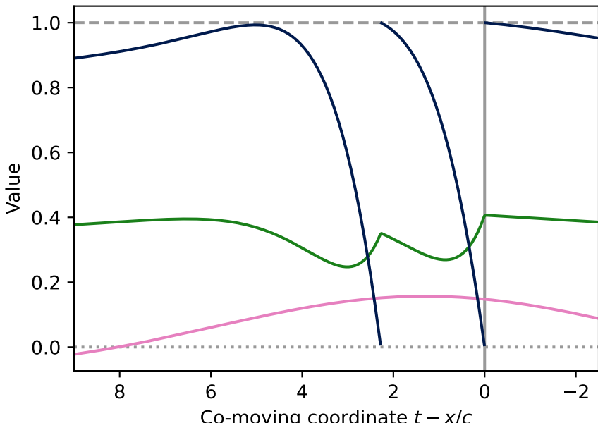
Travelling wave profile, c = 0.20
