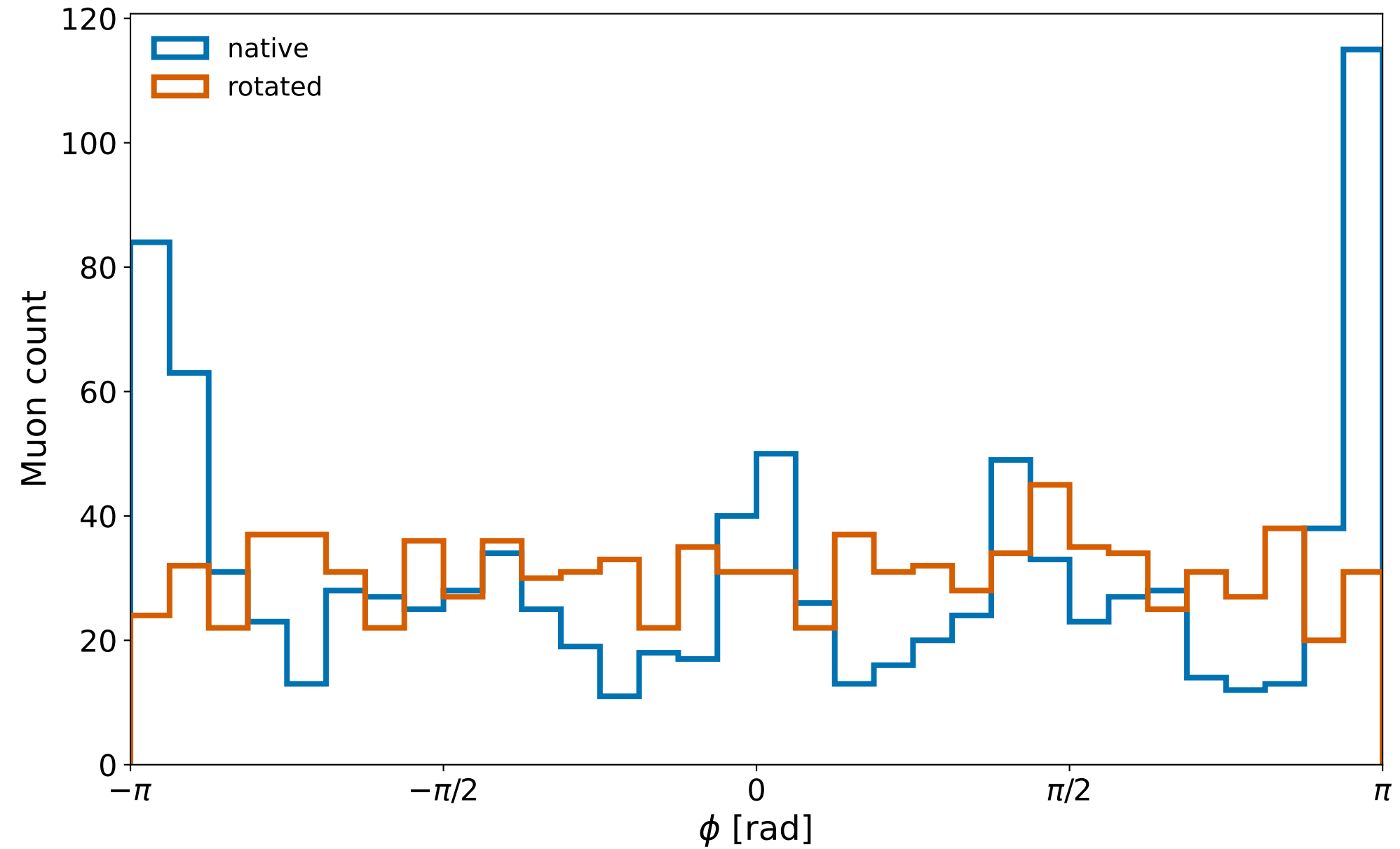
Muon momentum \phi (987 muons)
