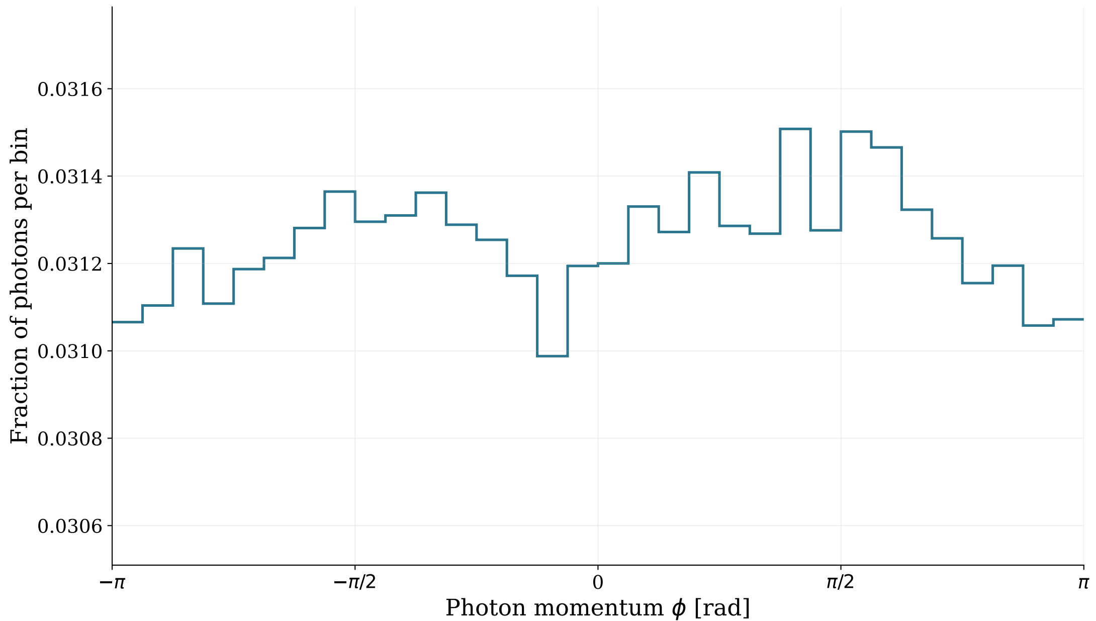
Unrotated BIB photon \phi : 0.5 \leq E < 2 MeV (5,521,766 photons)
