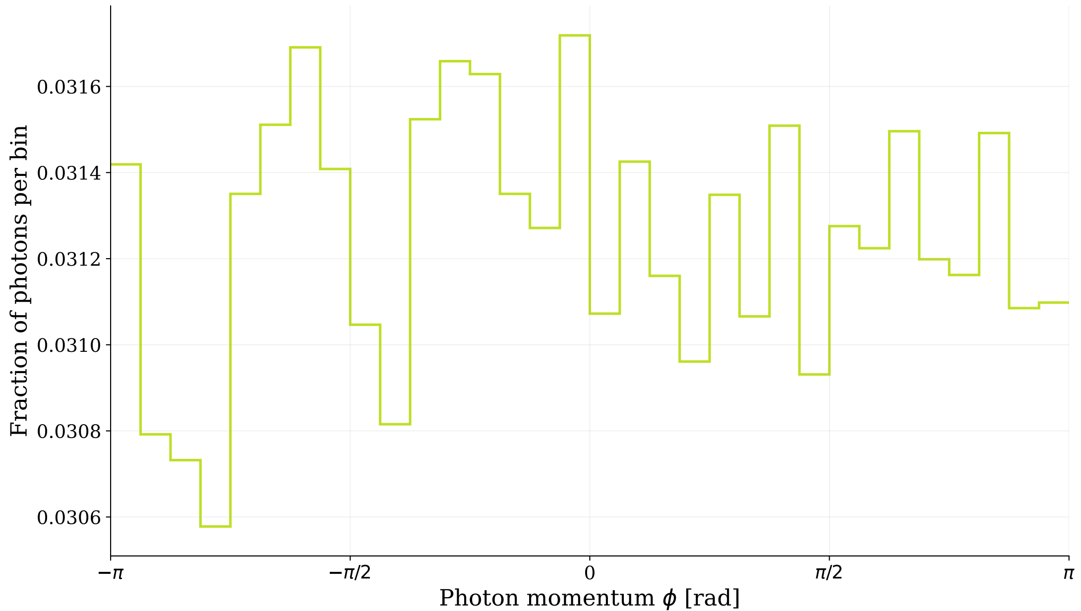
Unrotated BIB photon \phi : E \geq 5 MeV (467,265 photons)
