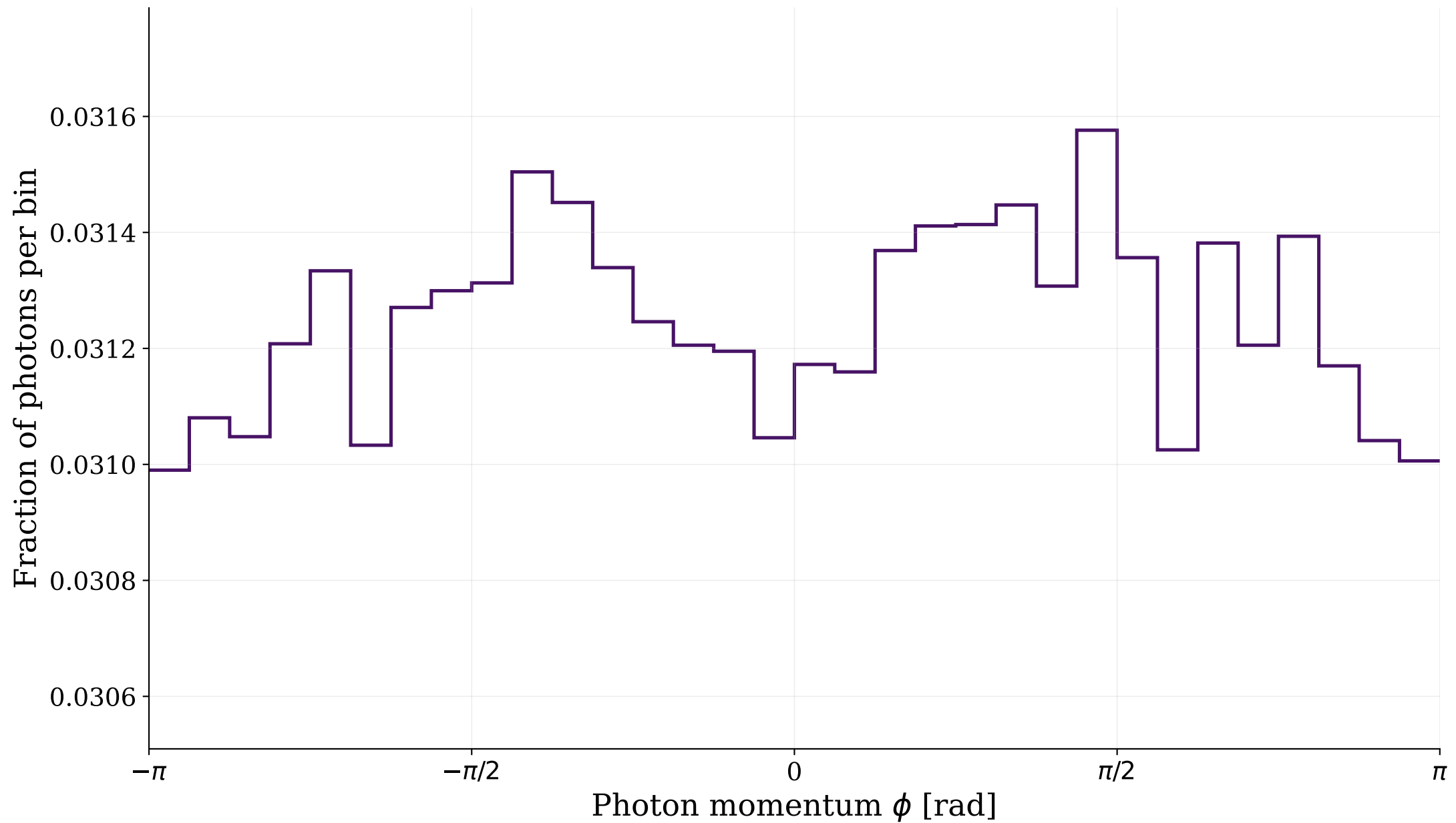
Unrotated BIB photon \phi : E < 0.5 MeV (1,629,230 photons)
