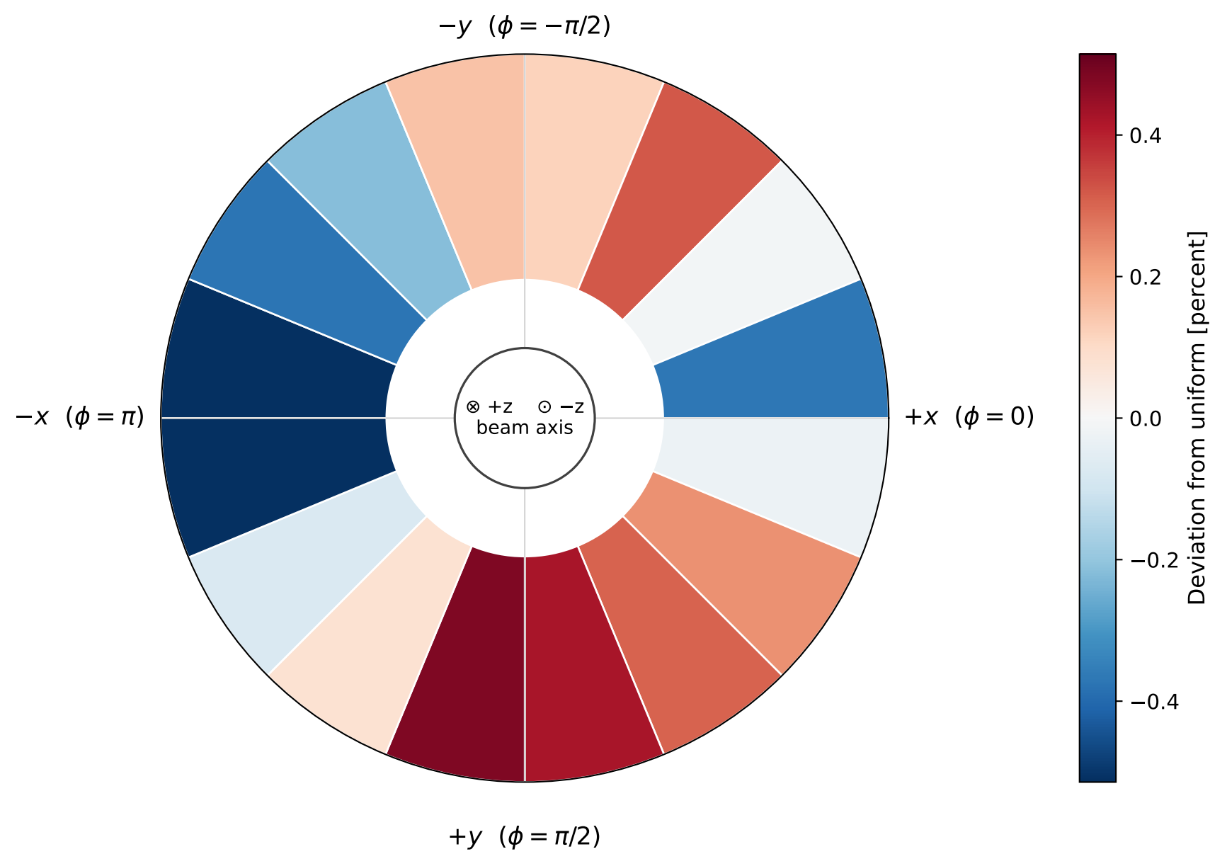
BIB photon momentum in the x-y plane (9,415,611 photons)
