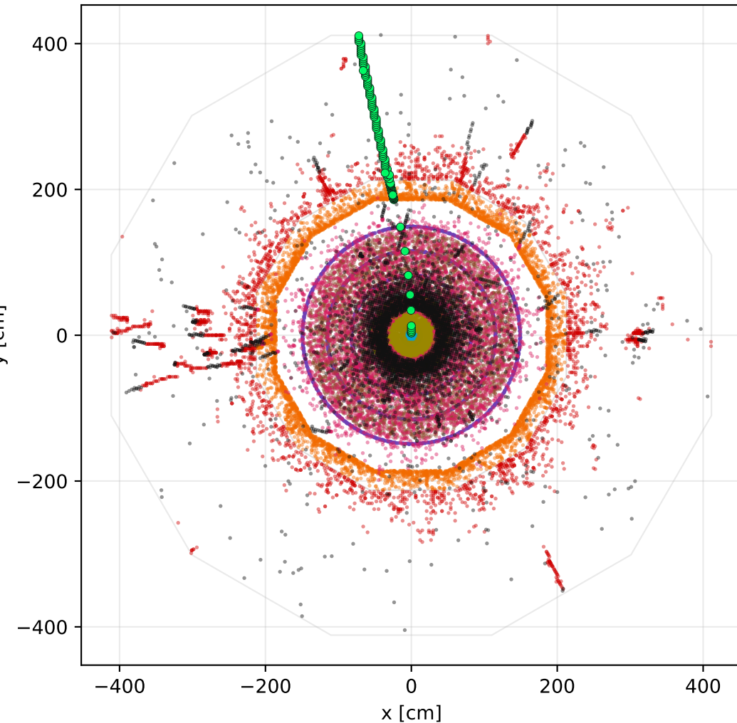
Barrel muon + BIB, event 0: all hits plotted 47,877 of 372,407 hits
