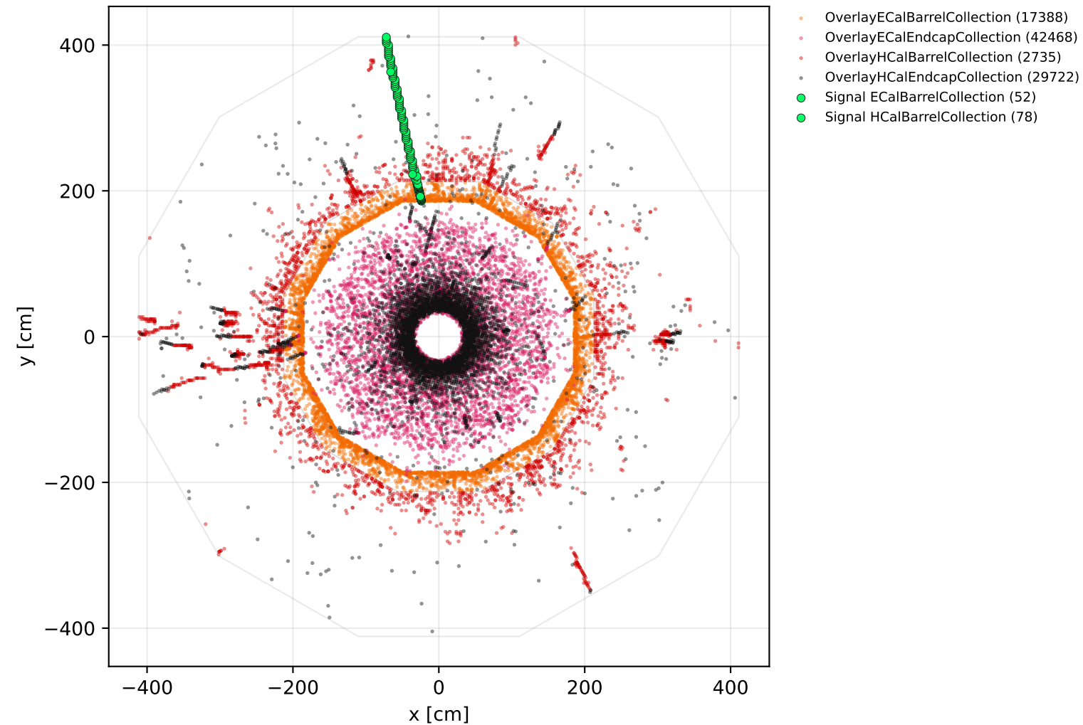
Barrel muon + BIB, event 0: calorimeter hits plotted 17,865 of 92,443 hits
