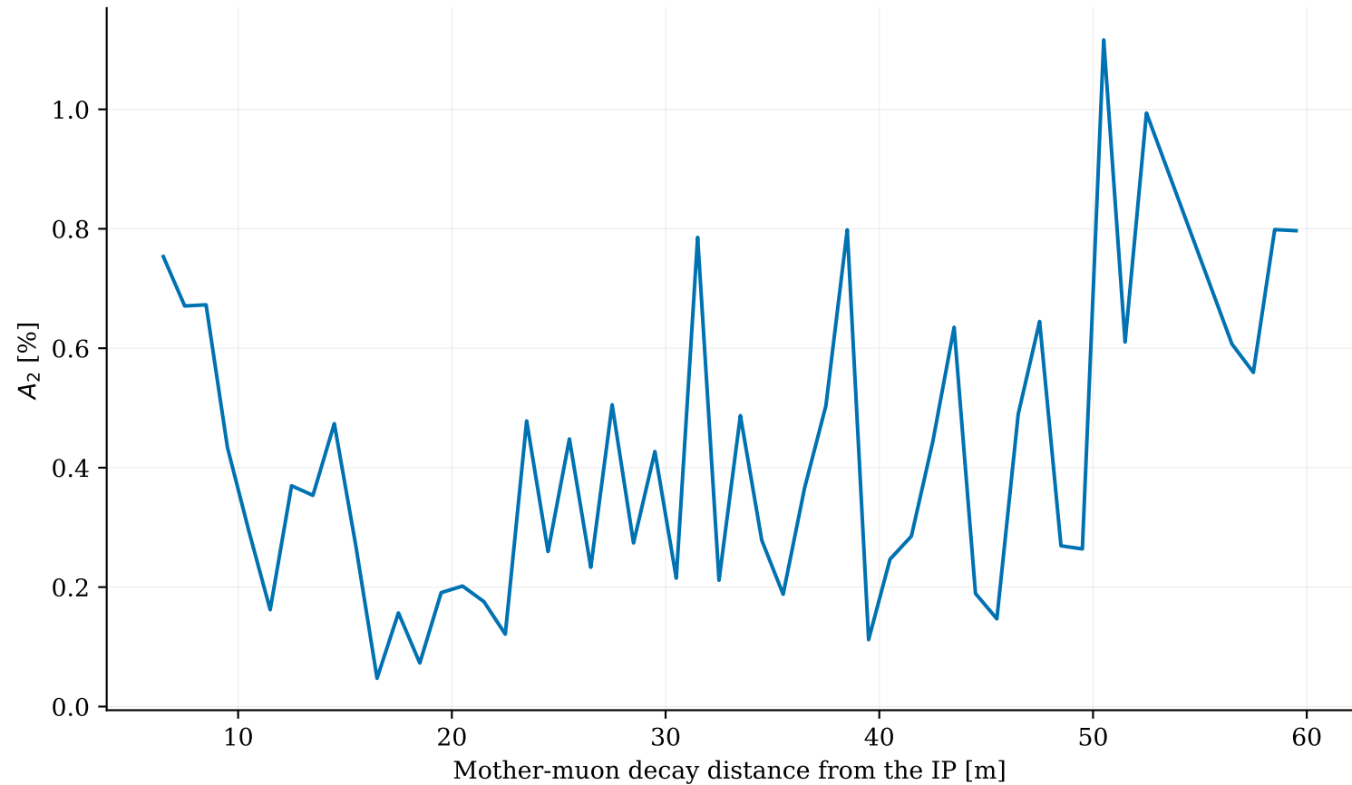
BIB photon A_2 versus mother-muon decay position
