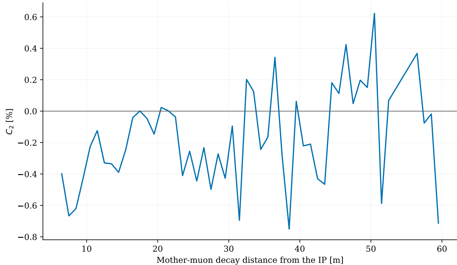
BIB photon C_2 versus mother-muon decay position
