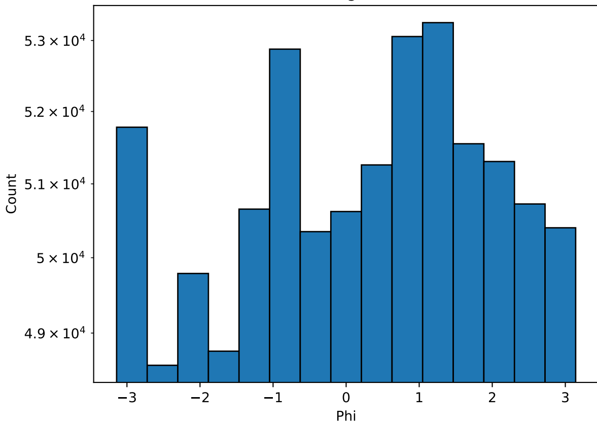
Phi for Meaningful Tracks [0]
