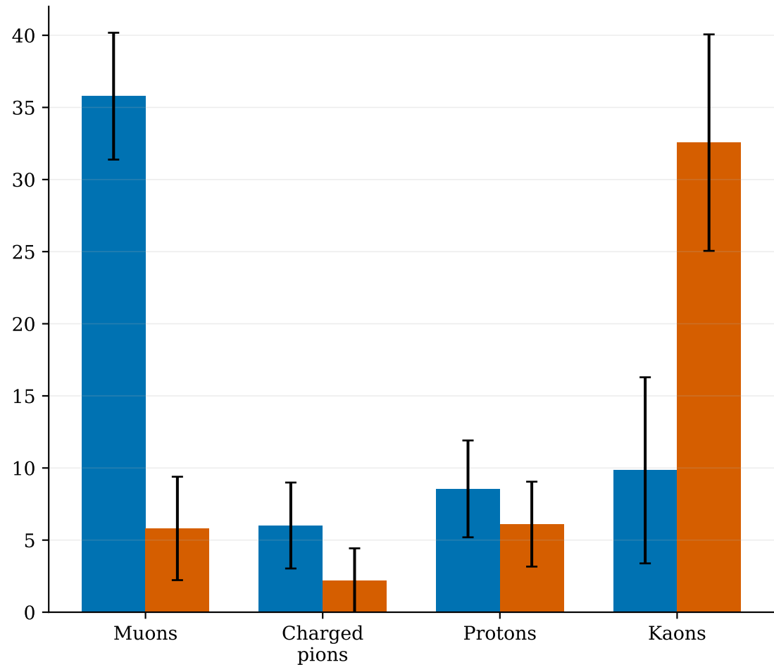
Second harmonic of BIB particle momentum \phi
