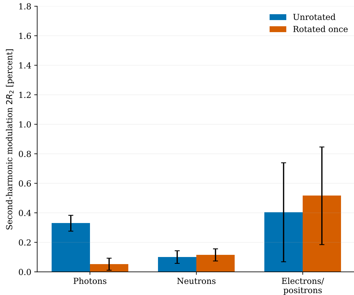
Second harmonic of BIB particle momentum \phi
