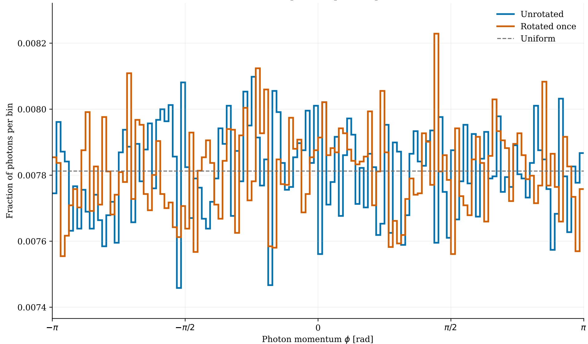
BIB photon momentum \phi , E > 5 MeV 467,265 photons per sample
