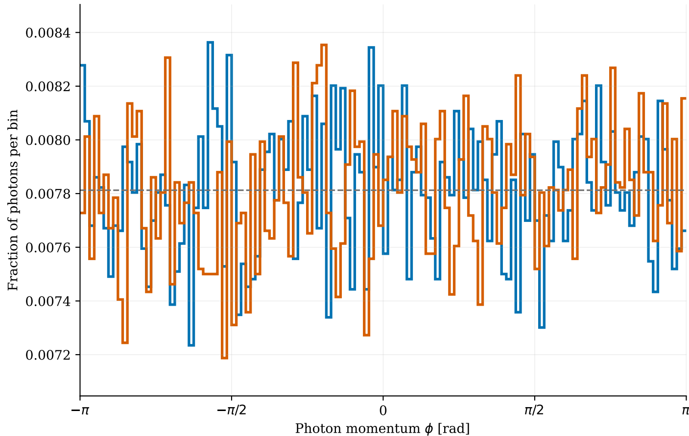
BIB photon momentum \phi , E > 10 MeV 105,463 photons per sample
