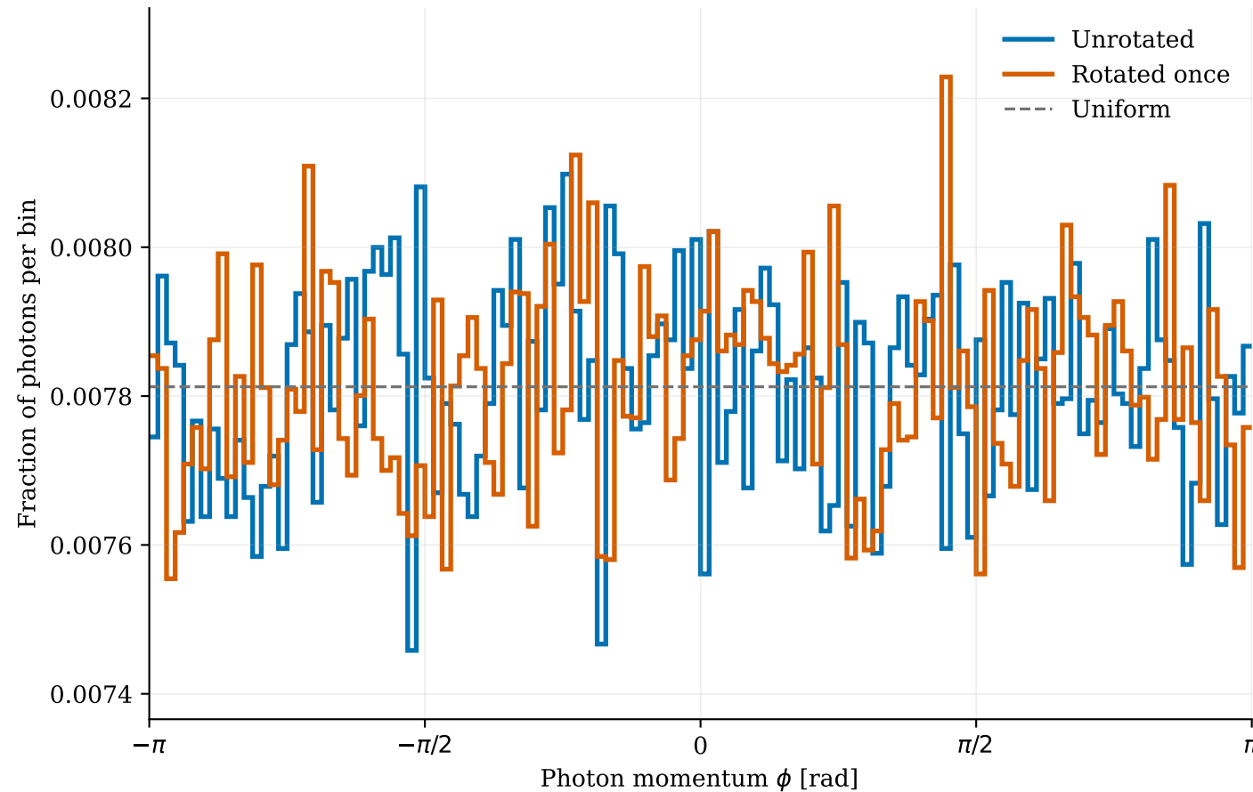
BIB photon momentum \phi , E > 5 MeV 467,265 photons per sample
