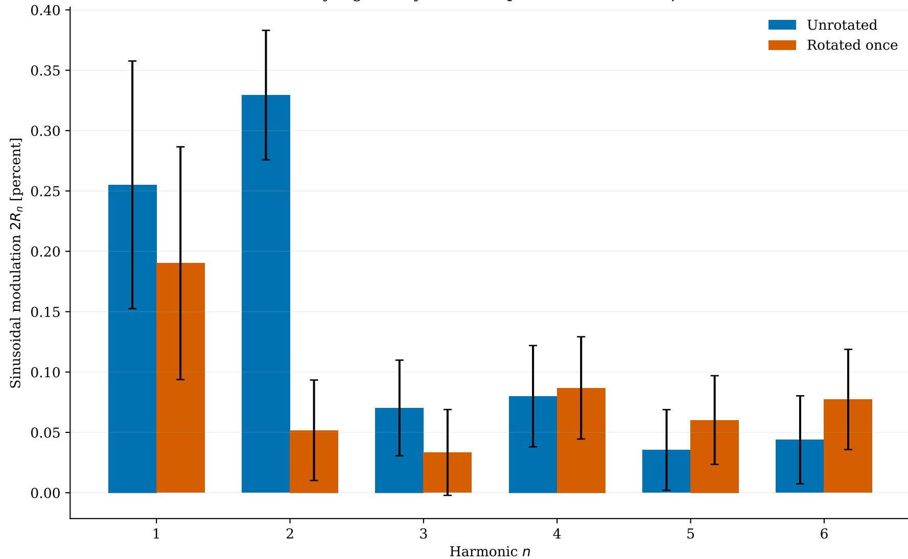
Rayleigh analysis of BIB photon momentum \phi
