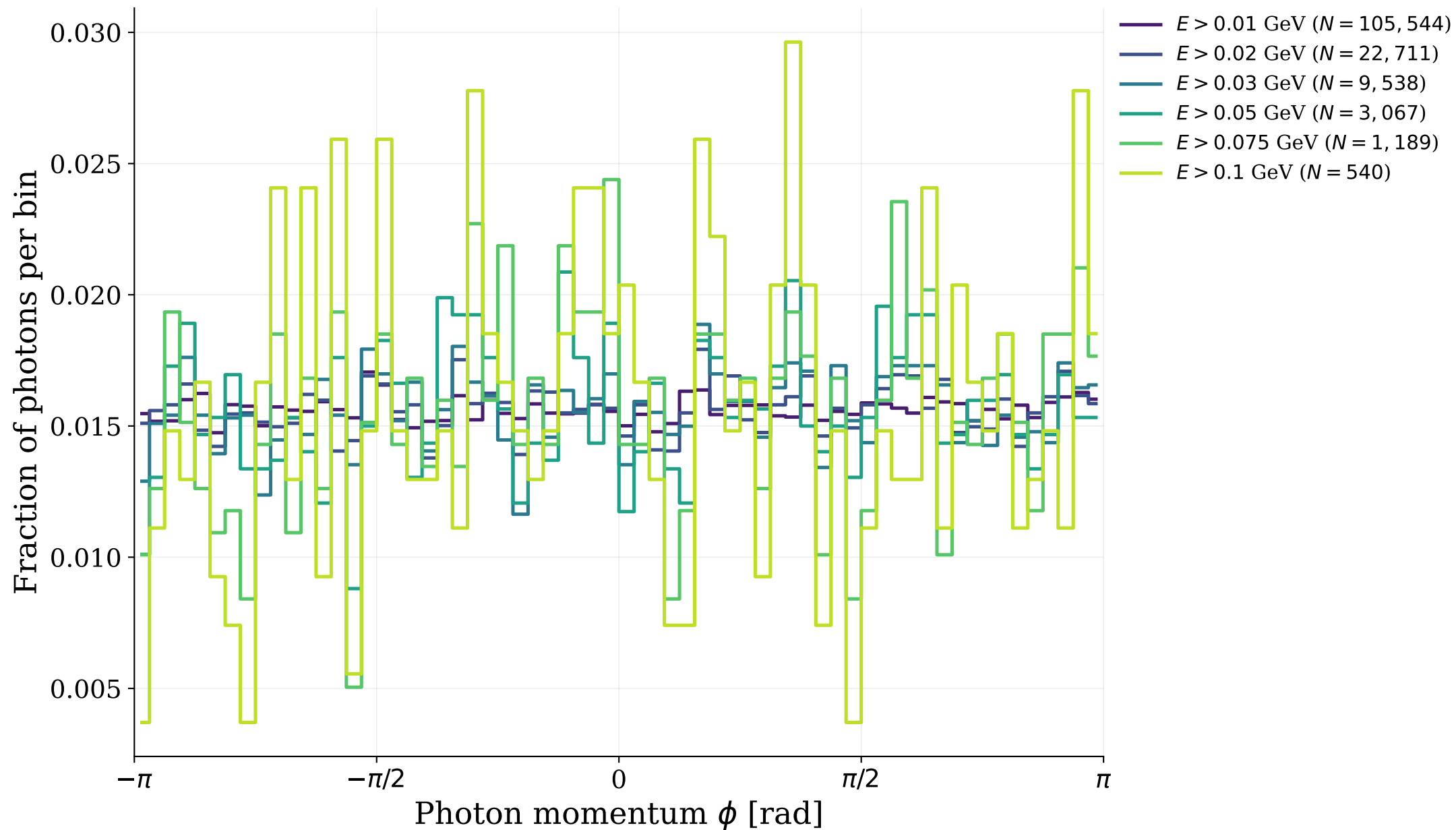
Unrotated BIB photon \phi by energy threshold
