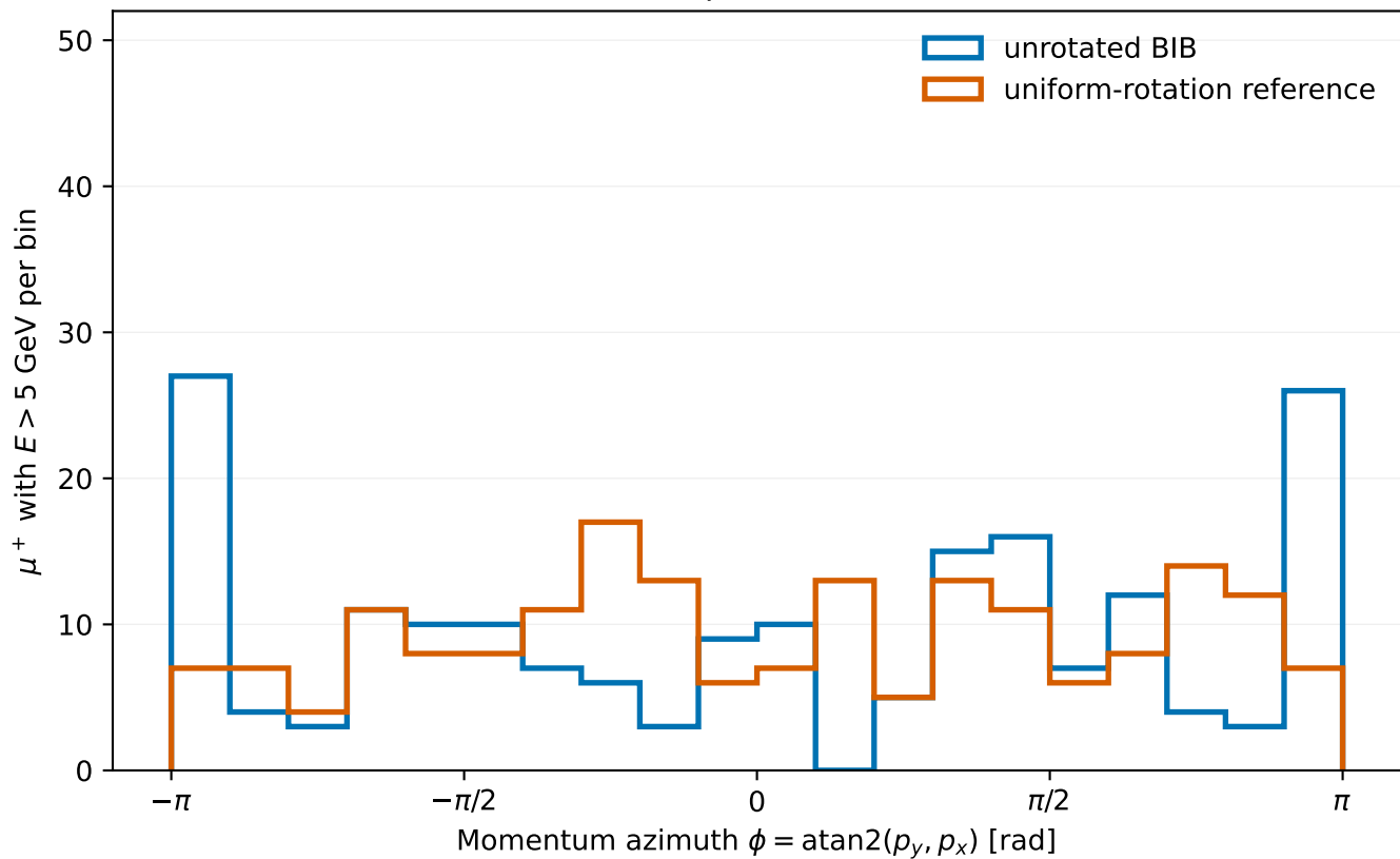
MUPLUS GEN BIB: \mu^+ momentum azimuth
