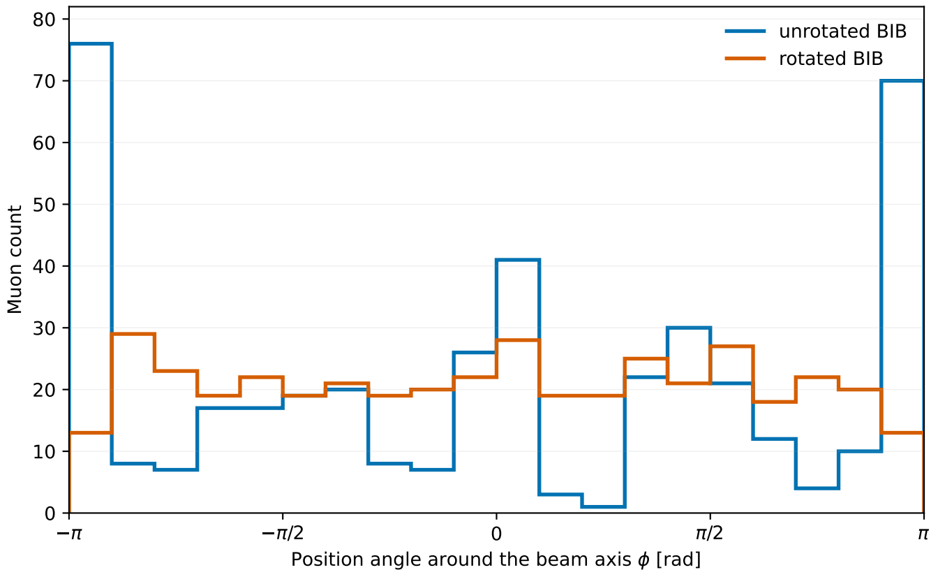
High-energy muon position in MUPLUS BIB ( E > 5 GeV)
