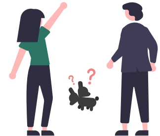
Inconsistent Training
