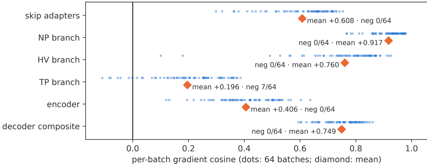
DSB gate B amended rerun: Dead vs common-class gradients (fold 1)
