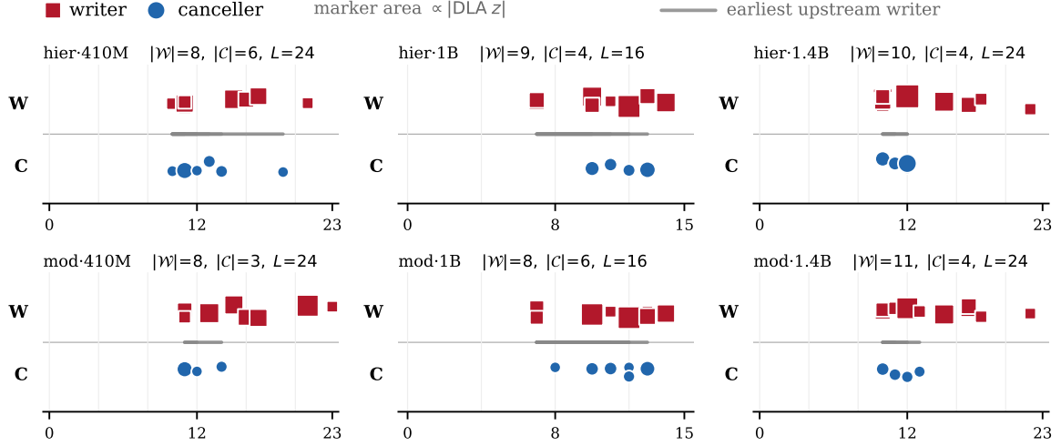
Figure 3: Layer distribution of writers and cancellers. Marker area \propto z -scored |DLA| ; grey lines connect each canceller to its earliest upstream writer. Cancellers cluster in early-to-mid layers and 23/27 have an upstream writer, ruling out late-stage suppression.
