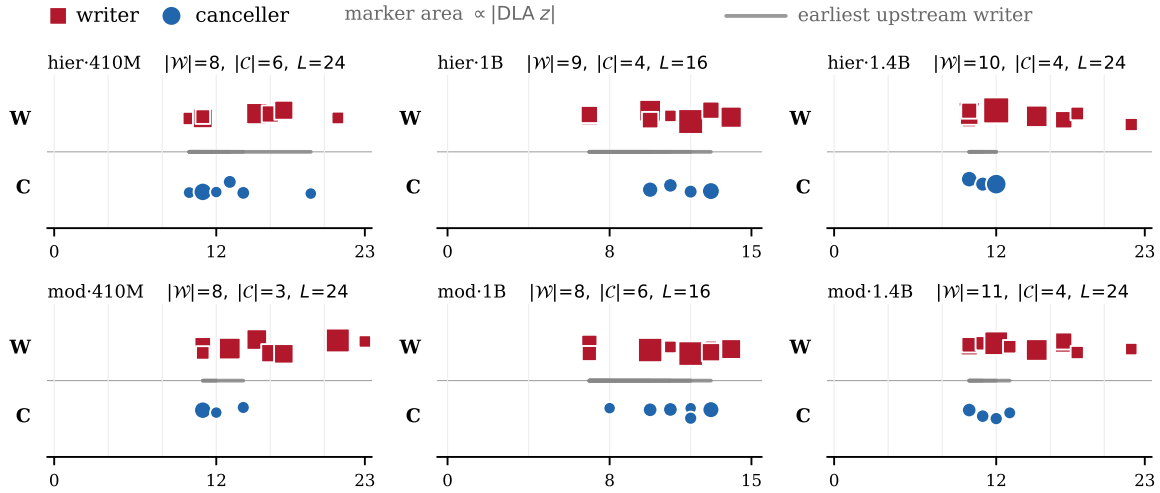
Figure 5: Layer distribution of writers and cancellers. Marker area \propto z -scored |DLA| ; gray lines connect each canceller to its earliest upstream writer. Cancellers cluster in early-to-mid layers and 23/27 have an upstream writer, ruling out late-stage suppression.
