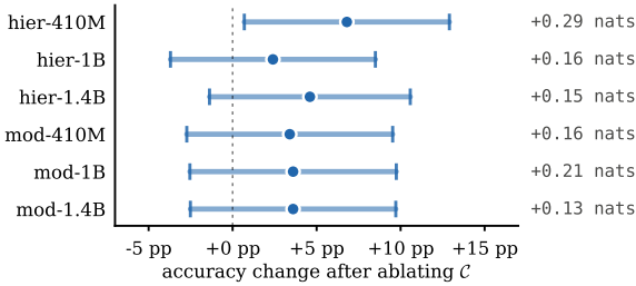
Figure 3: Cancellation ablation: actionable consequence. Per-cell accuracy delta after zero-ablating \mathcal{C} , with paired-bootstrap 95% CI; logit-shift magnitude annotated on the right. Sign is positive in 6/6 main cells; CI excludes 0 on hier-410M. App. D.3 Table 21.
