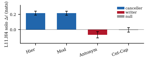
Figure 4: L11.H4 case study: cross-template sign-flip. Solo-ablation \Delta\ell on the four templates (paired bootstrap 95% CI). Blue = canceller, red = writer, grey = null. The head’s address transfers across all four templates but its role is task-conditional.
