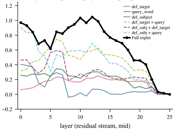
(a) Layer-wise patching by source group (Gemma-2-2B)
